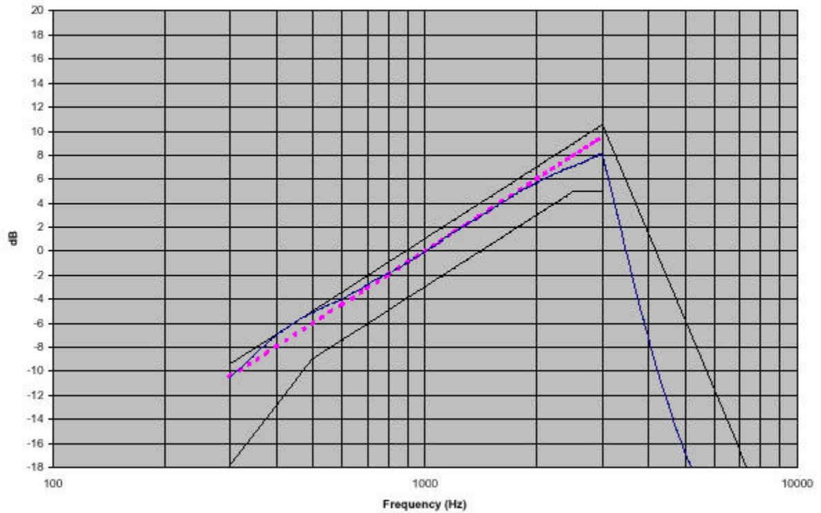
Channel 4 - 12.5 kHz Audio Frequency Response
