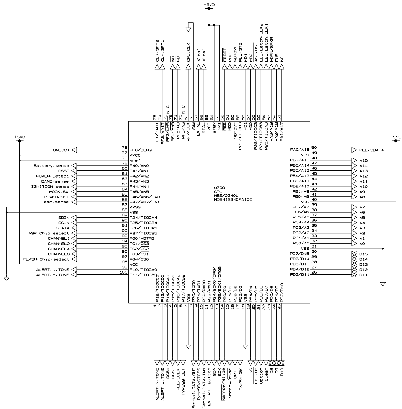
PANTHER 300M UHF-H LOGIC SCHEMATIC DIAGRAM (G2UD06391, Rev0, Sheet 4 of 4)
