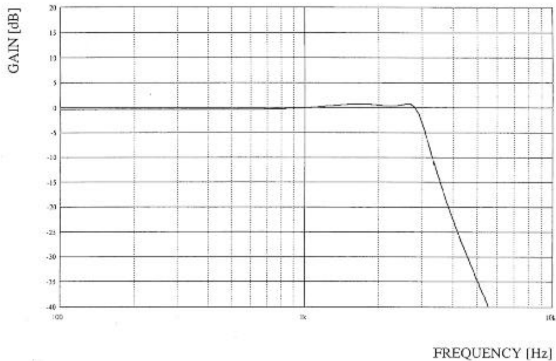
Fig.4 B LPF( F_c=2.55\text{kHz} ) Frequency Response (Reference)
