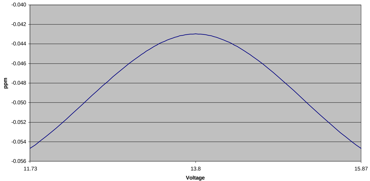
Voltage Frequency Stability (13.8 Nominal) Worst Case -0.055 ppm
