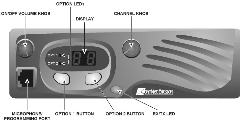
Figure 1 – PANTHER 300M mobile radio Front View
