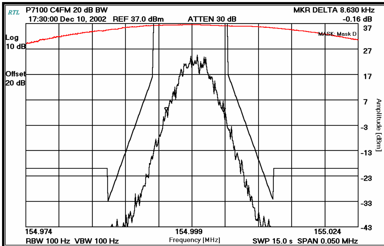
PLOT 7-5: OCCUPIED BANDWIDTH; NARROW BAND; 20 DB BANDWIDTH; C4FM DIGITAL MODULATION
