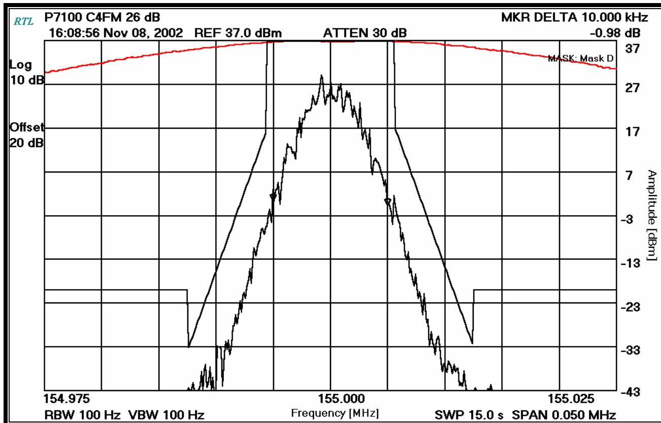
PLOT 13-3: 26 DB BANDWIDTH; NARROW BAND; C4FM DIGITAL MODULATION
