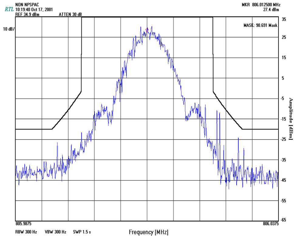
PLOT 7-4: OCCUPIED BANDWIDTH {MASK EA; (2 LEVEL FM DIGITAL MODULATION)} PART 90.210
