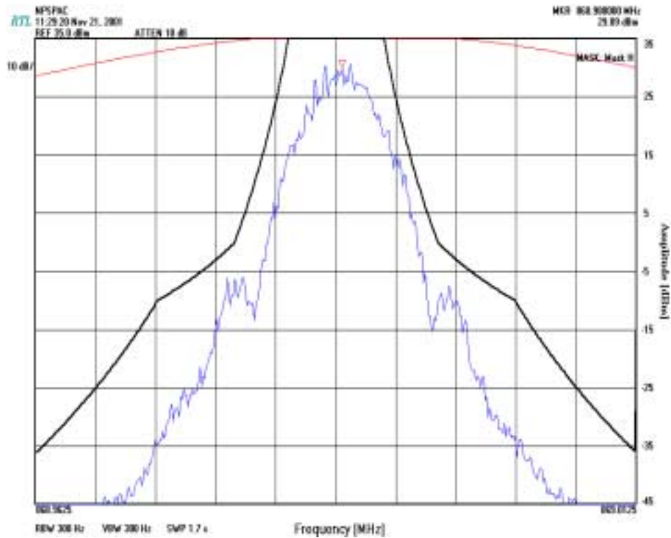
PLOT 7-5: OCCUPIED BANDWIDTH {MASK H; (NPSPAC 2 LEVEL FM DIGITAL MODULATION)} PART 90.210
