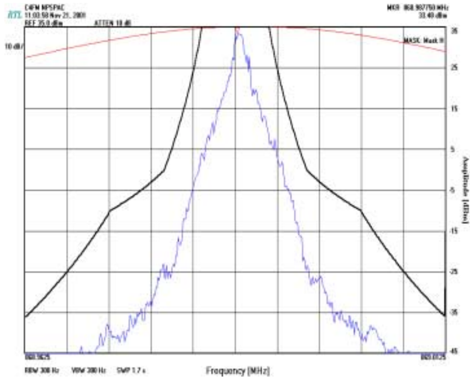
PLOT 7-9: OCCUPIED BANDWIDTH {MASK H; (C4FM NPSPAC DIGITAL MODULATION)} PART 90.210
