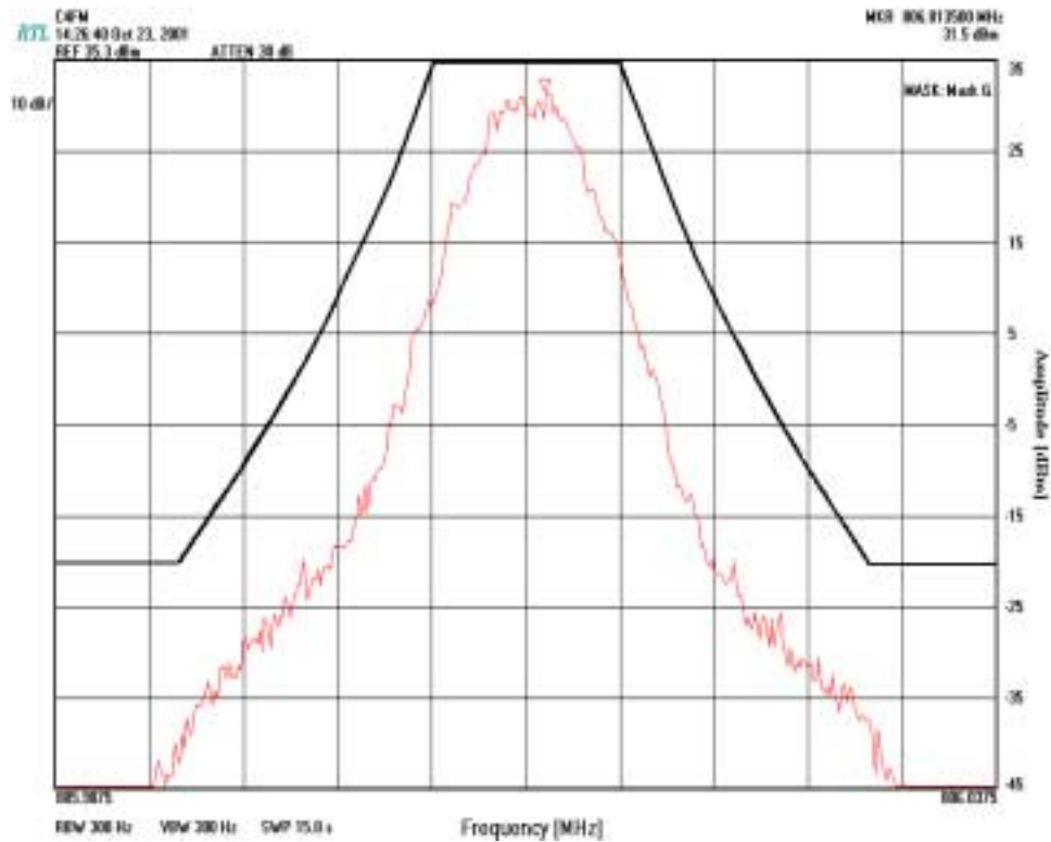
PLOT 7-8: OCCUPIED BANDWIDTH {MASK G; (C4FM NON-NPSPAC DIGITAL MODULATION)} PART 90.210
