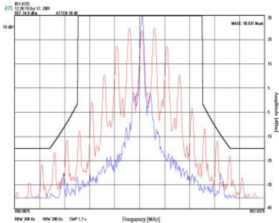
PLOT 7-3: OCCUPIED BANDWIDTH {25 kHz CHANNEL BANDWIDTH: MASK EA; FCC PART 90.691(AUDIO MODULATION: 2,500 HZ)} PART 90.210
