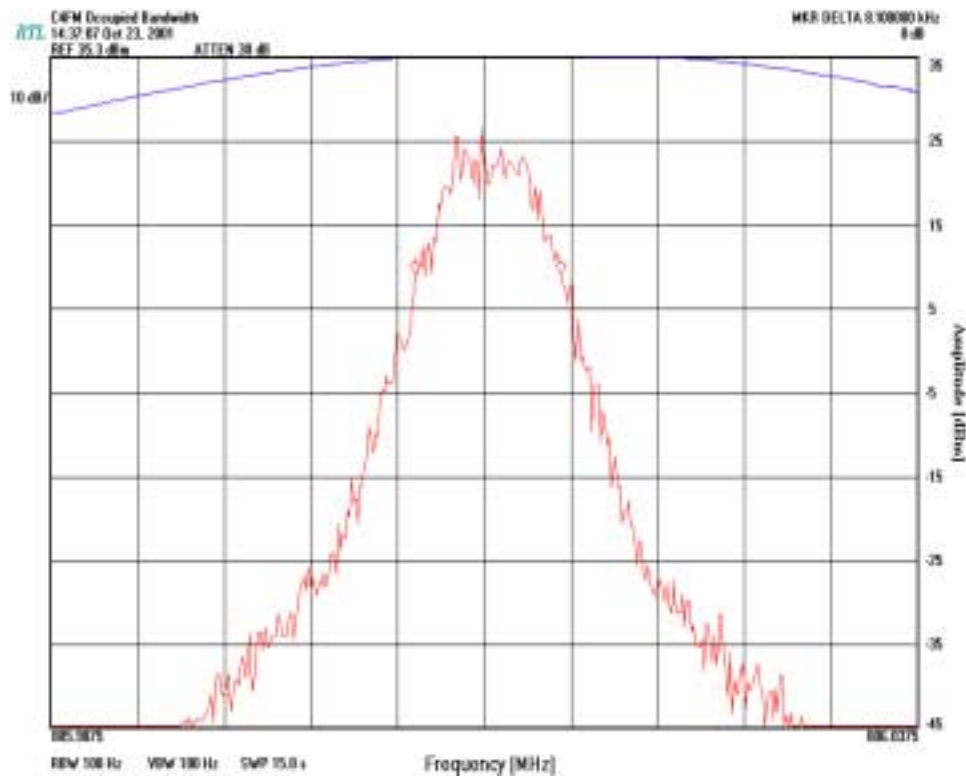
PLOT 7-11: OCCUPIED BANDWIDTH (C4FM NON-NPSPAC DIGITAL MODULATION) (8.1 KHZ) – 99% POWER BANDWIDTH; PART 90.210
