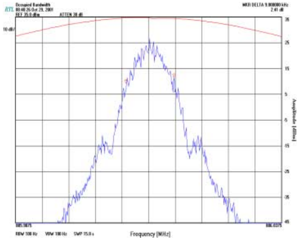
PLOT 7-10: OCCUPIED BANDWIDTH (NON-NPSPAC 2 LEVEL FM DIGITAL MODULATION) (9 KHZ) – 99% POWER BANDWIDTH; PART 90.210
