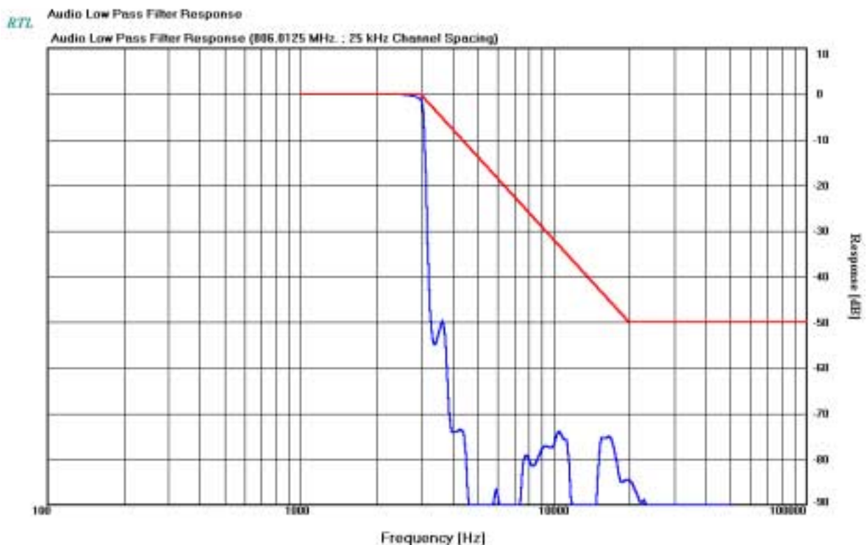
PLOT 10-1: MODULATION CHARACTERISTICS – AUDIO LOW PASS FILTER
