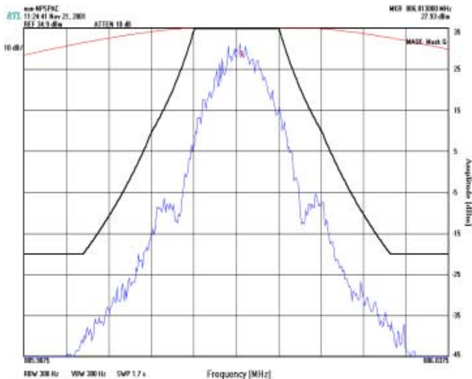
PLOT 7-6: OCCUPIED BANDWIDTH {MASK G; (NON-NPSPAC 2 LEVEL FM DIGITAL MODULATION)} PART 90.210
