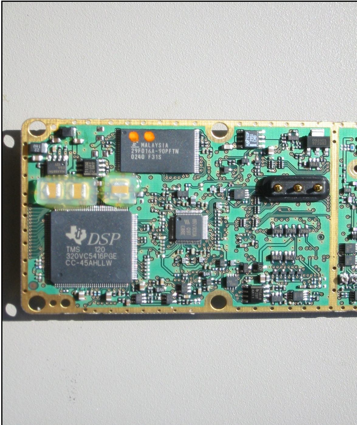
PHOTOGRAPH 3: MAIN PCB BOTTOM VIEW LEFT SIDE
