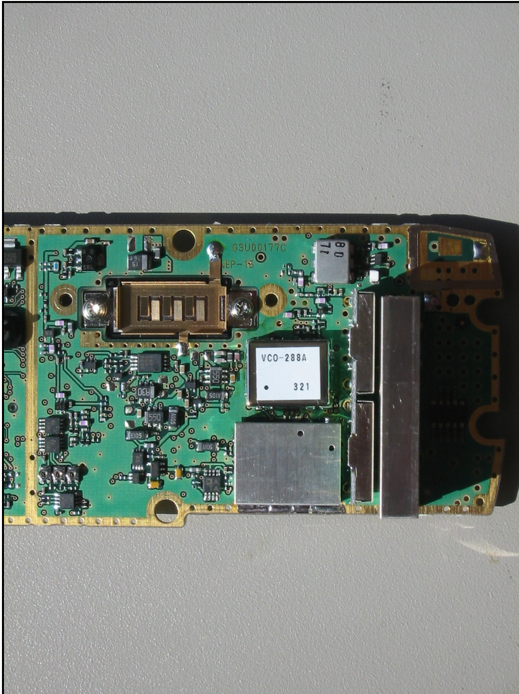
PHOTOGRAPH 4: MAIN PCB BOTTOM VIEW RIGHT SIDE
