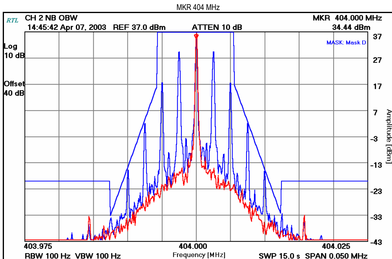
PLOT 9-2: OCCUPIED BANDWIDTH; NARROW BAND; AUDIO MODULATION: 2,500 HZ
