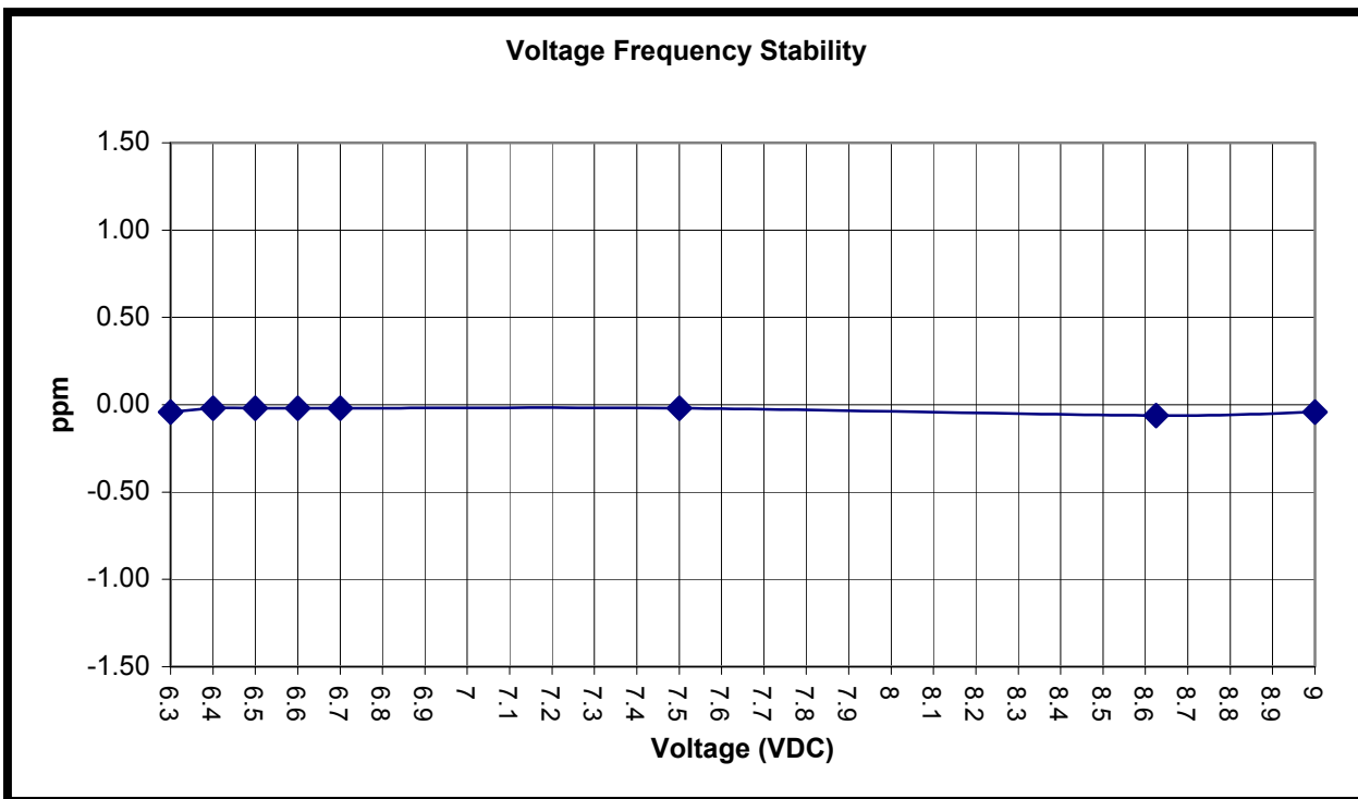
PLOT 10-2: VOLTAGE FREQUENCY STABILITY
