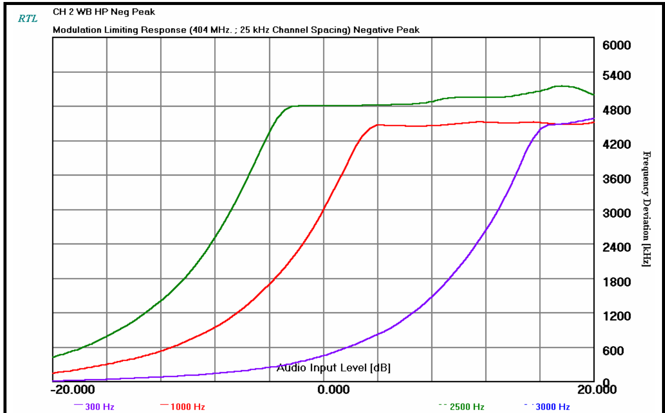
PLOT 13-2: MODULATION CHARACTERISTICS – MODULATION LIMITING: WIDE BAND; NEGATIVE PEAK
