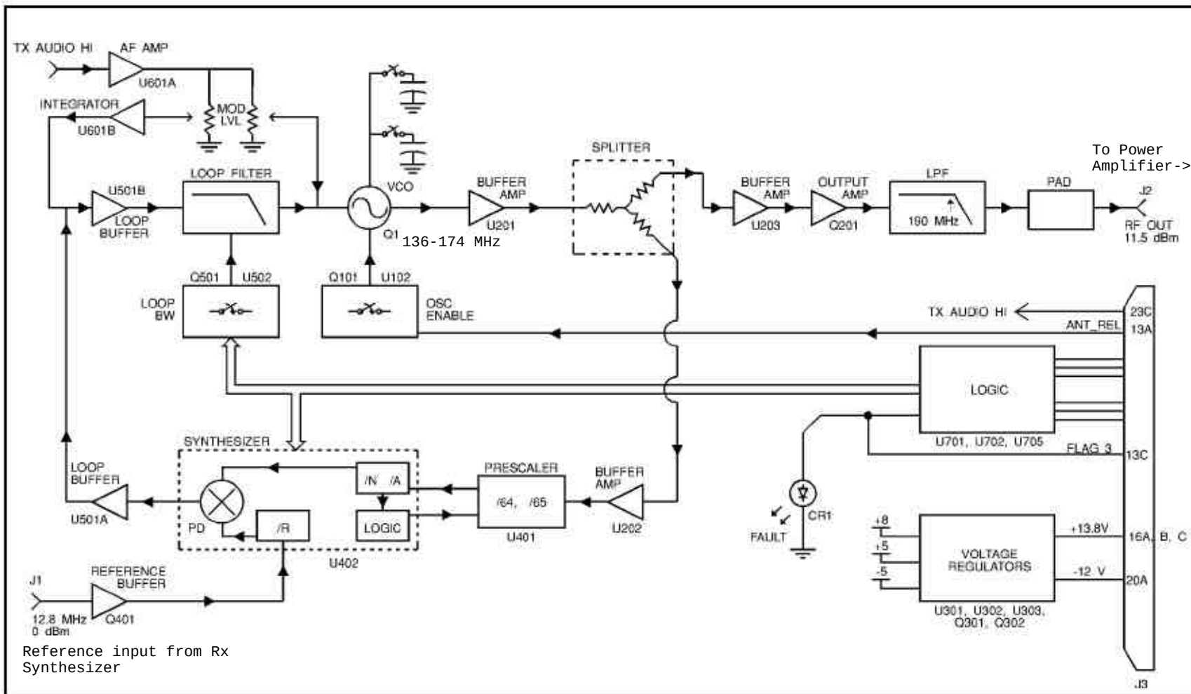
Figure 1 - Tx Synthesizer Block Diagram
