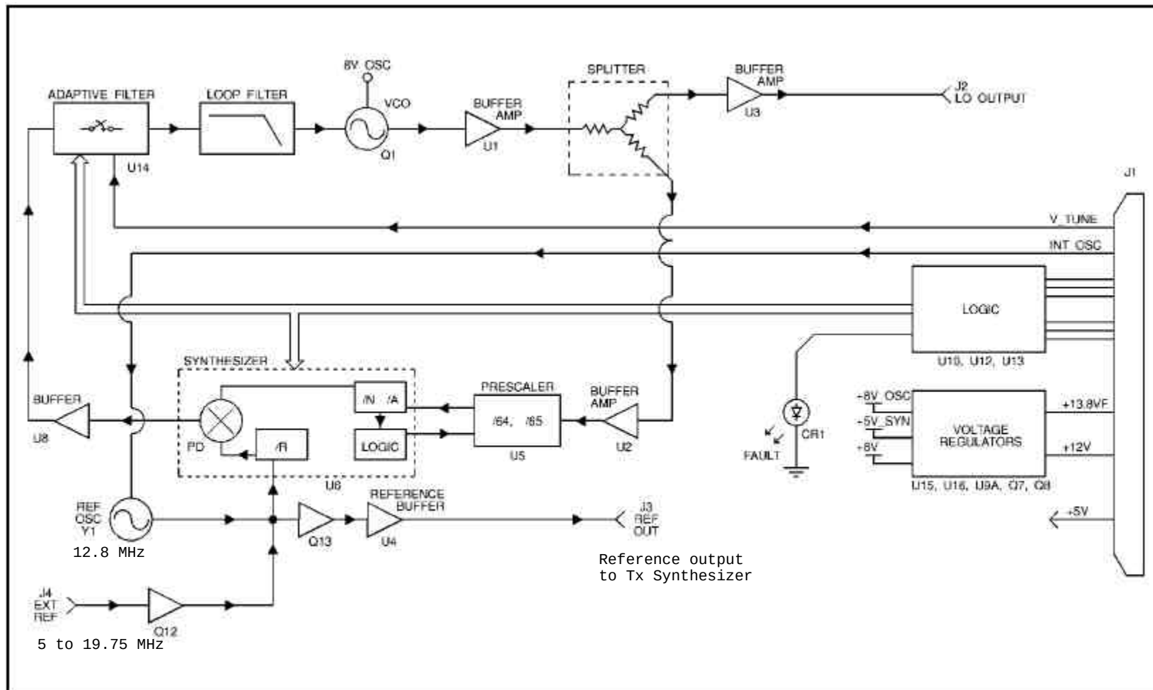
Figure 3 - Rx Synthesizer Block Diagram
