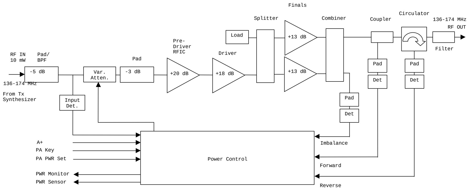
Figure 2 - VHF Power Amplifier Block Diagram
