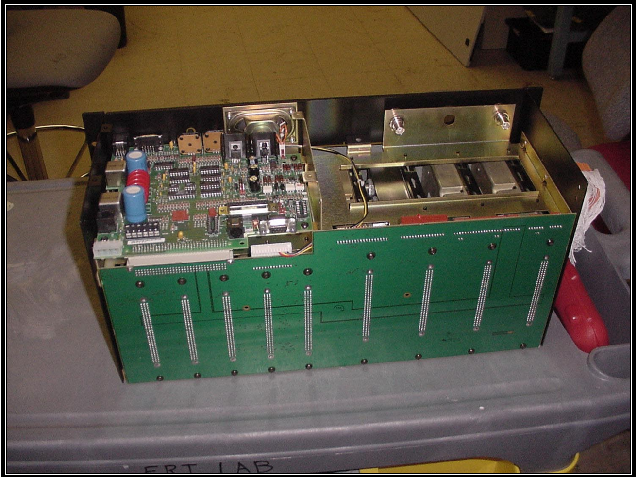
PHOTOGRAPH 4: MASTR III BACK TOP
