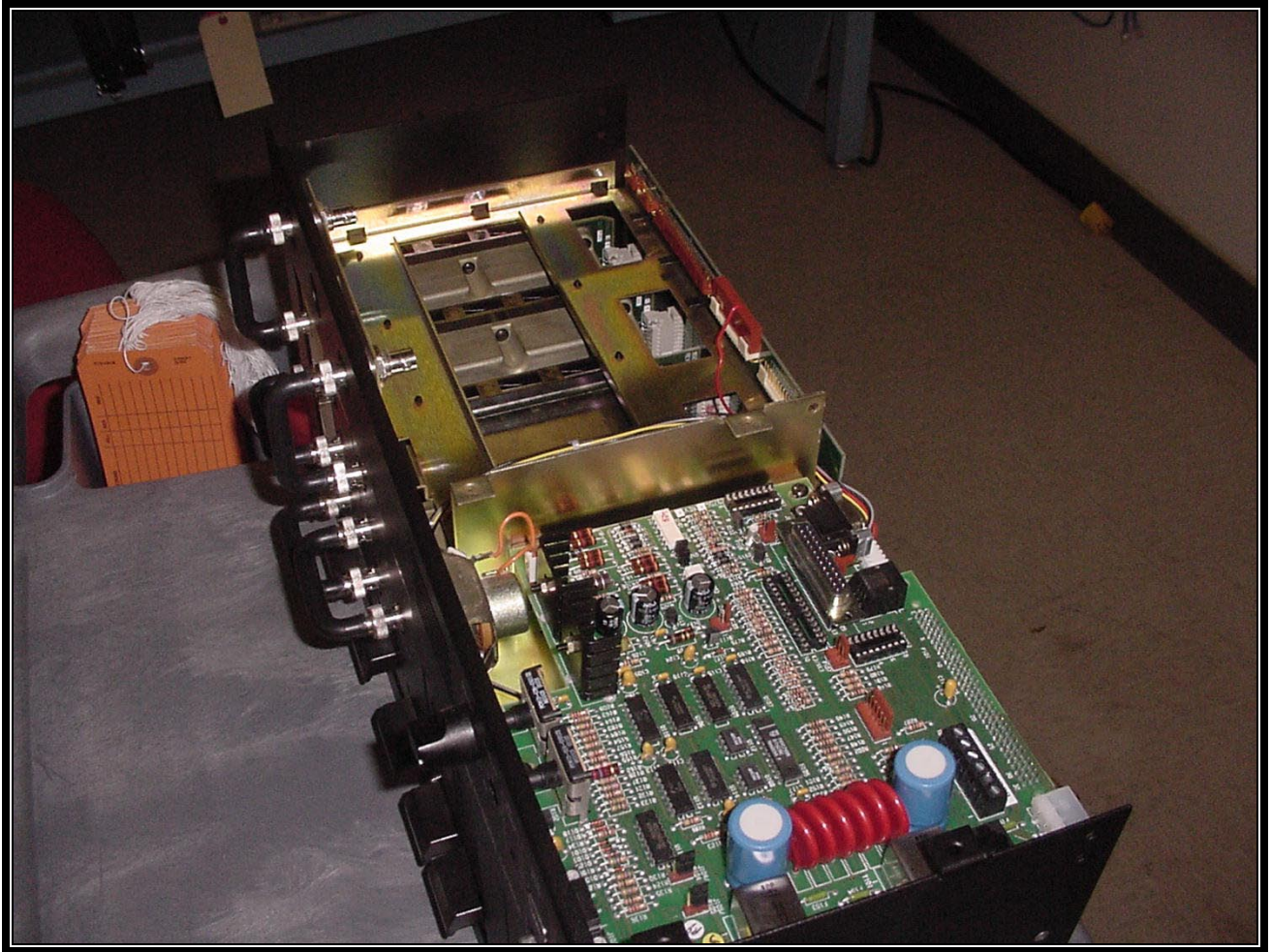
PHOTOGRAPH 5: MASTR III SIDE TOP
