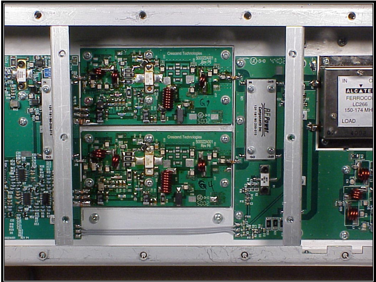
PHOTOGRAPH 16: VHF PA FINALS
