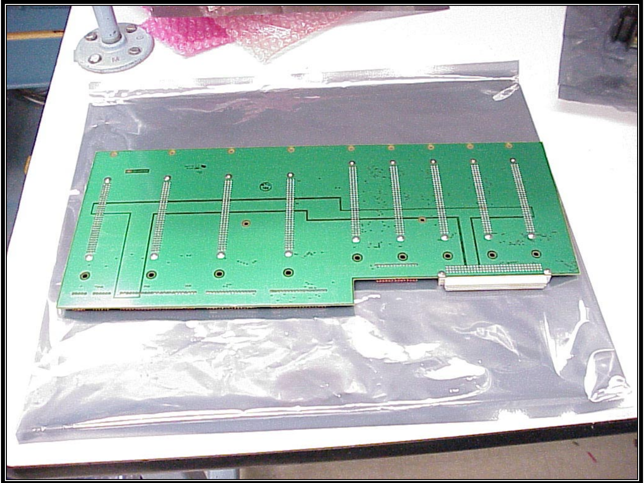
PHOTOGRAPH 7: BACK PLANE BOTTOM
