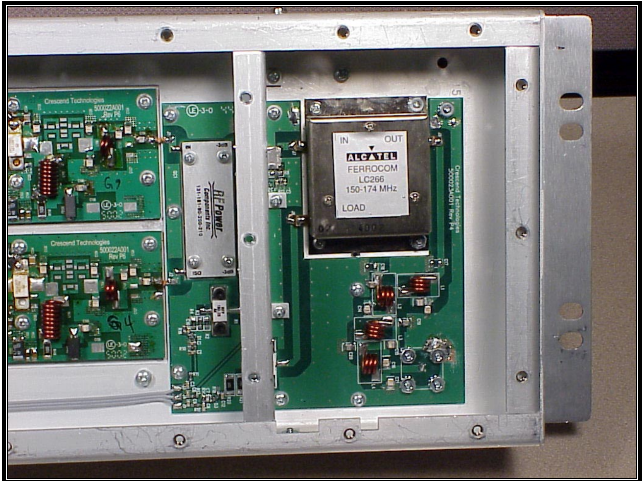
PHOTOGRAPH 15: VHF PA OUTPUT
