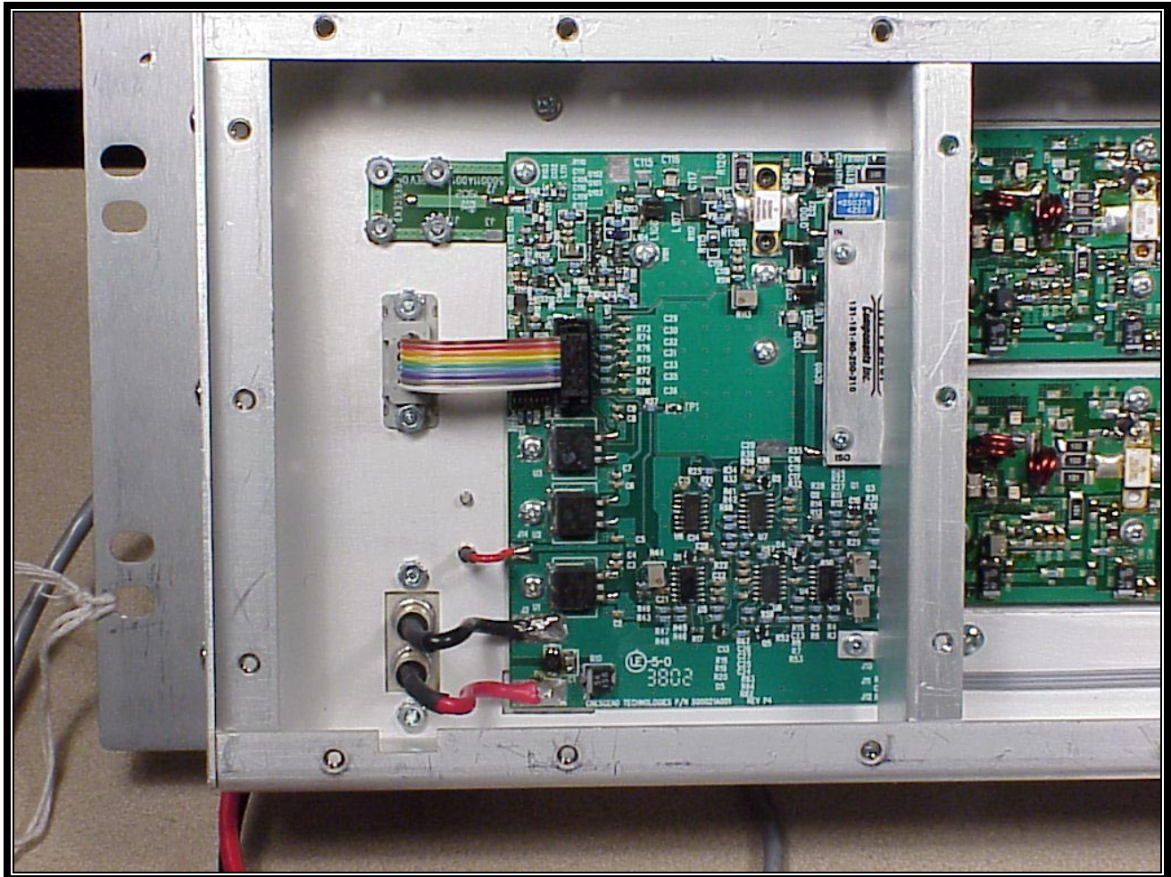
PHOTOGRAPH 14: VHF PA INPUT
