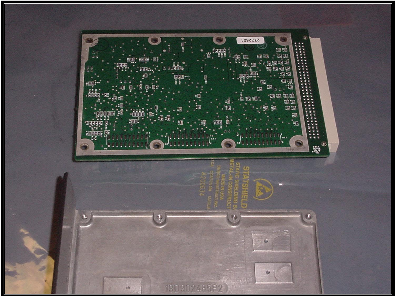
PHOTOGRAPH 10: DSP BOARD BOTTOM
