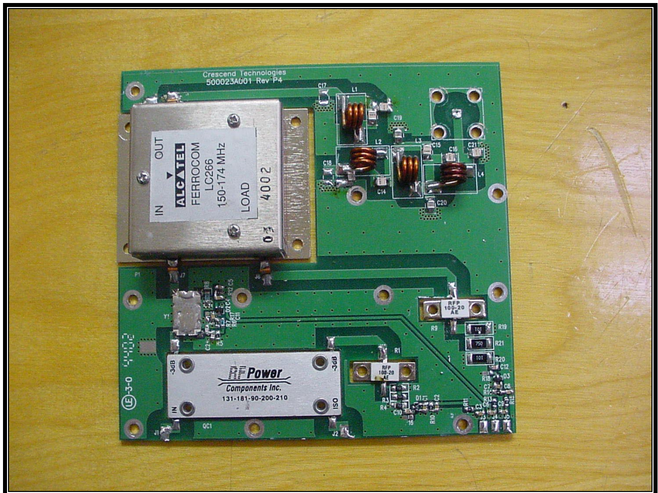
PHOTOGRAPH 18: VHF PA PCB #1 TOP
