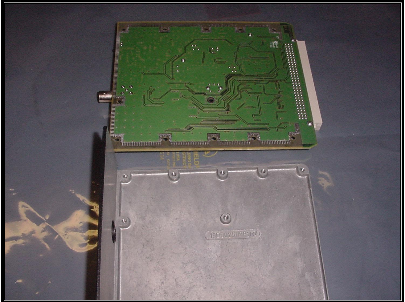
PHOTOGRAPH 42: RX IF BOARD BOTTOM
