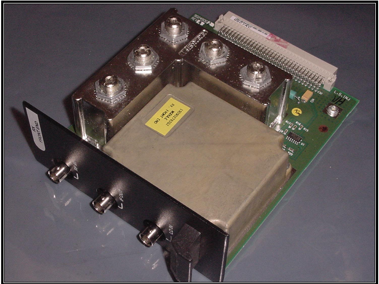
PHOTOGRAPH 37: RX FRONT END
