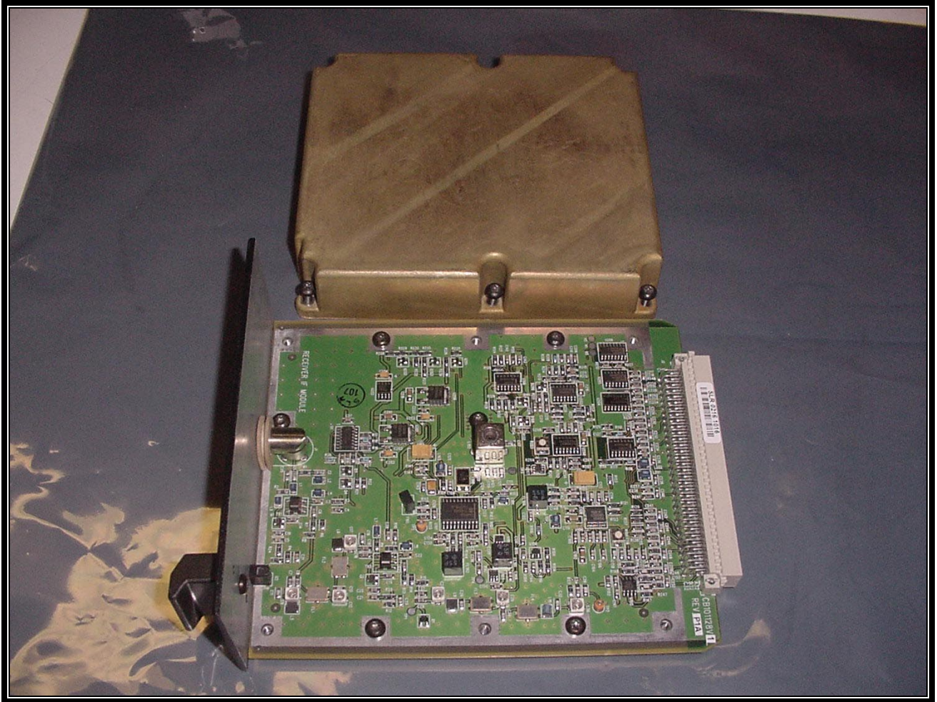
PHOTOGRAPH 41: RX IF BOARD TOP
