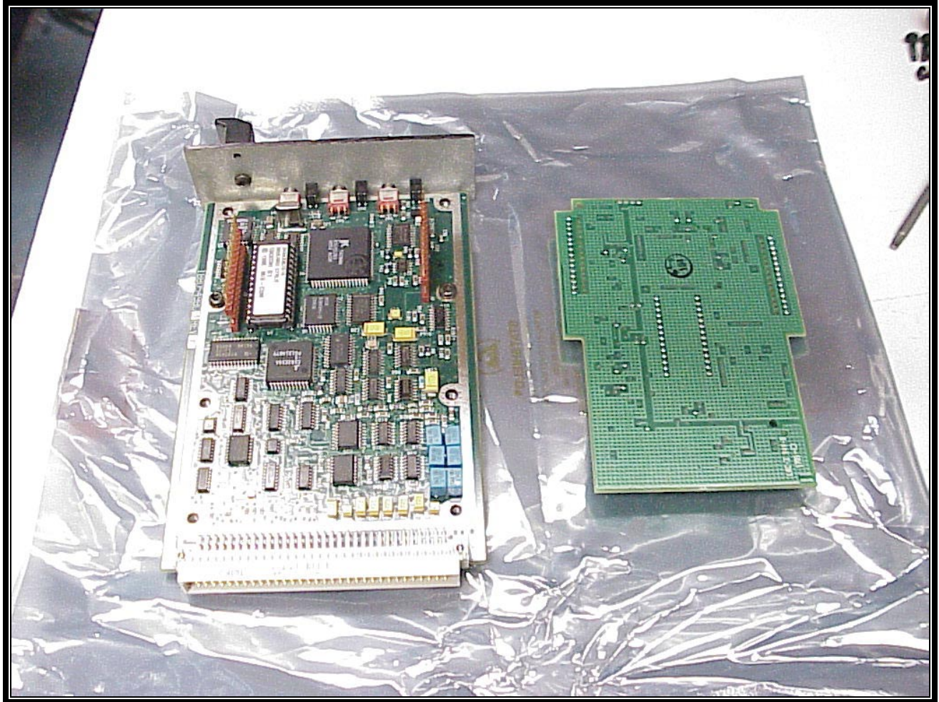
PHOTOGRAPH 33: SYSTEM MODULE, DSP BOTTOM
