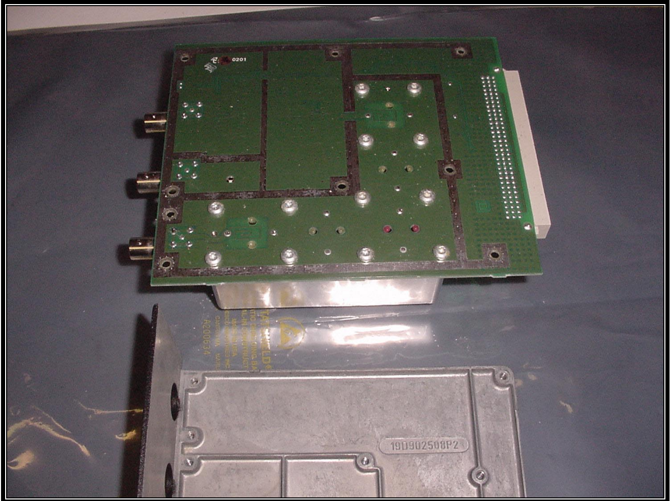
PHOTOGRAPH 39: RX FRONT END BOARD BOTTOM
