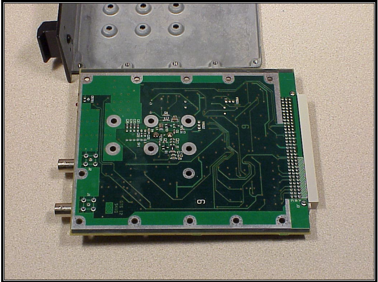
PHOTOGRAPH 50: TX SYNTH BOARD BOTTOM
