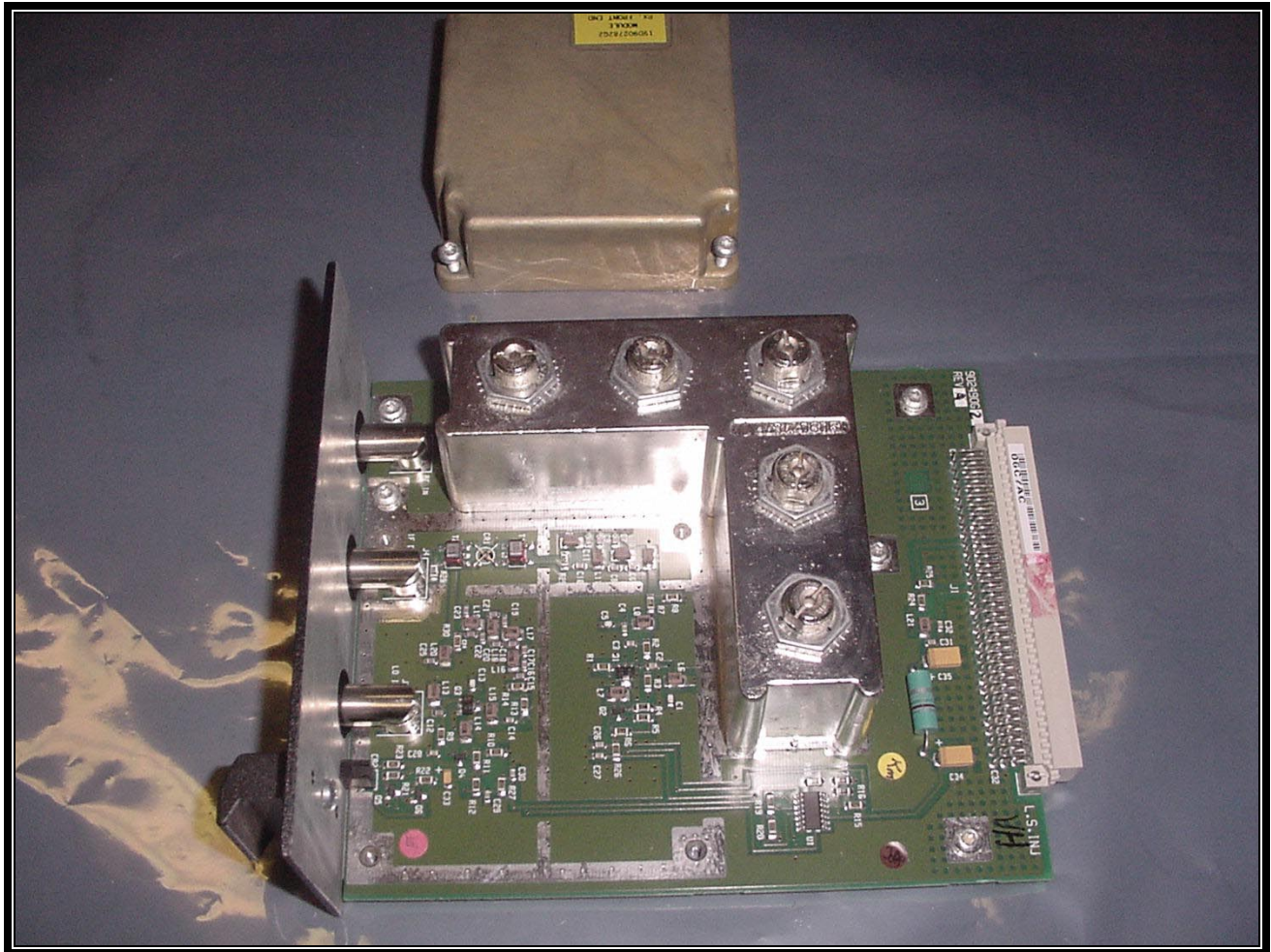
PHOTOGRAPH 38: RX FRONT END BOARD TOP
