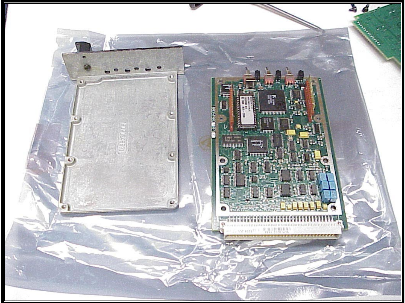
PHOTOGRAPH 30: SYSTEM MODULE MAIN BOARD TOP
