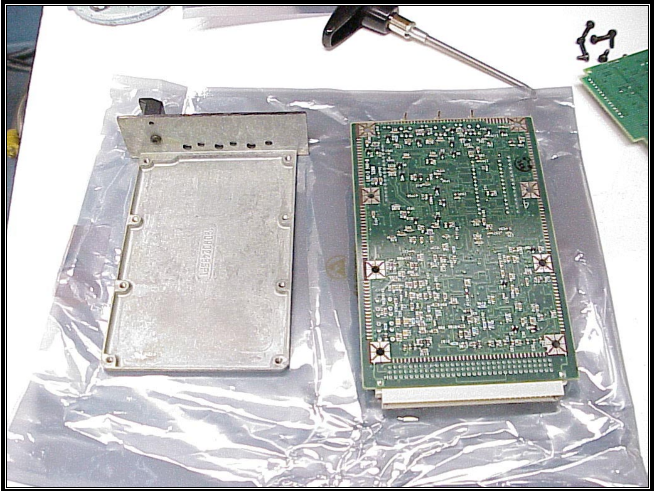
PHOTOGRAPH 31: SYSTEM MODULE MAIN BOARD BOTTOM
