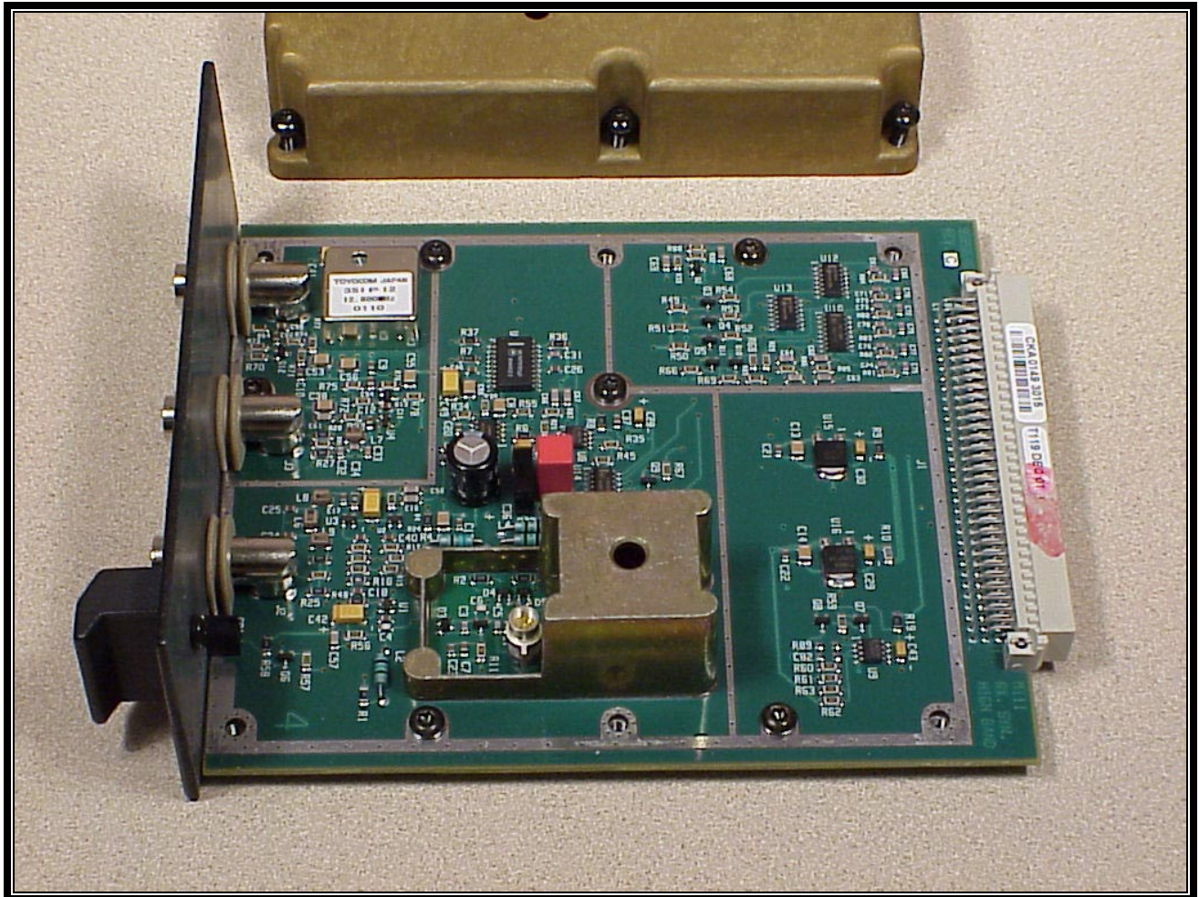
PHOTOGRAPH 45: RX SYNTH BOARD TOP
