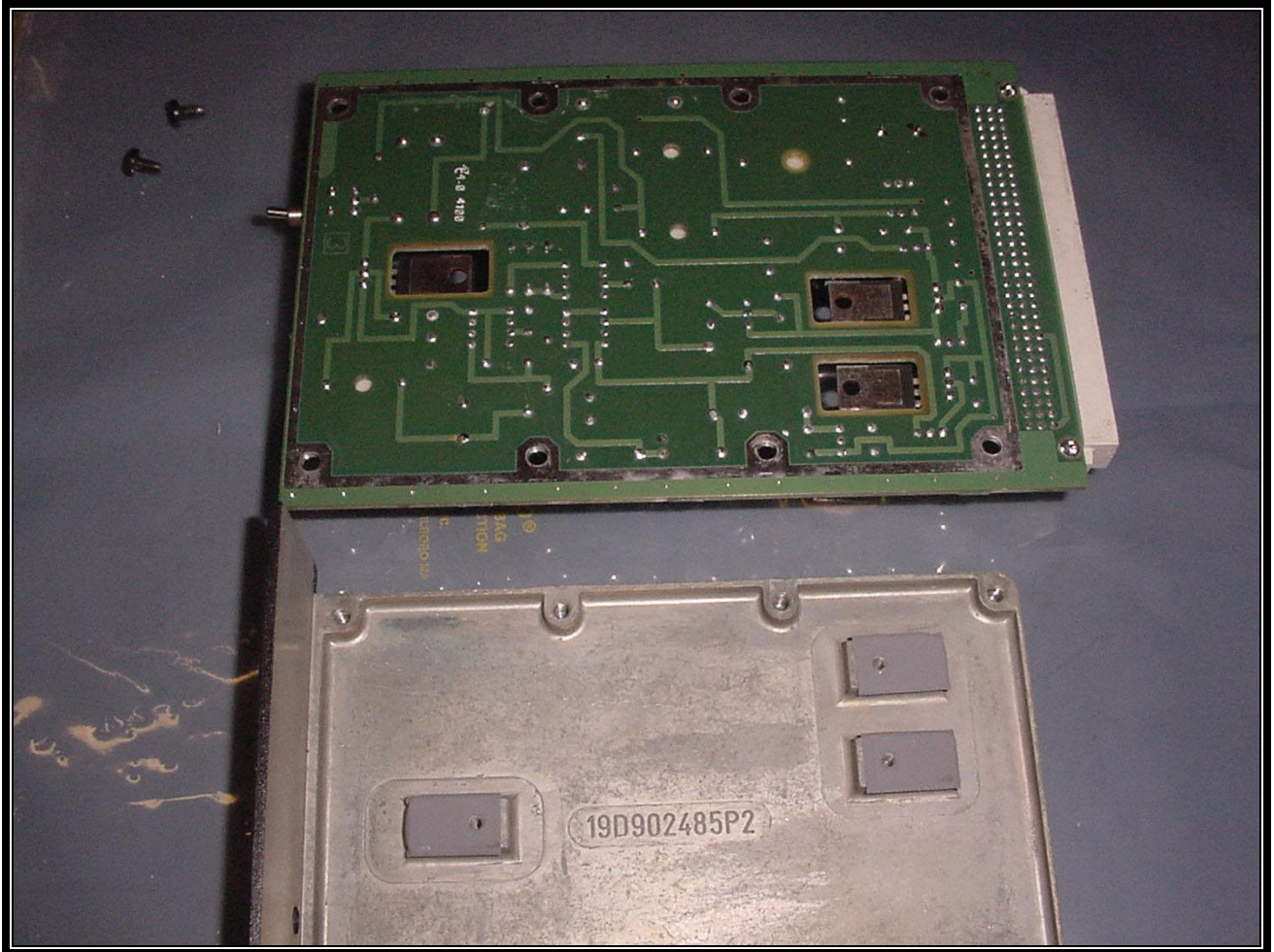
PHOTOGRAPH 36: POWER MODULE BOARD BOTTOM
