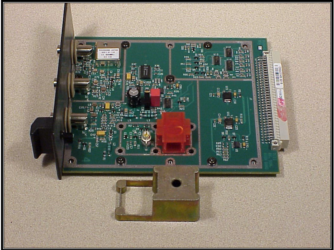
PHOTOGRAPH 44: RX SYNTH VCO
