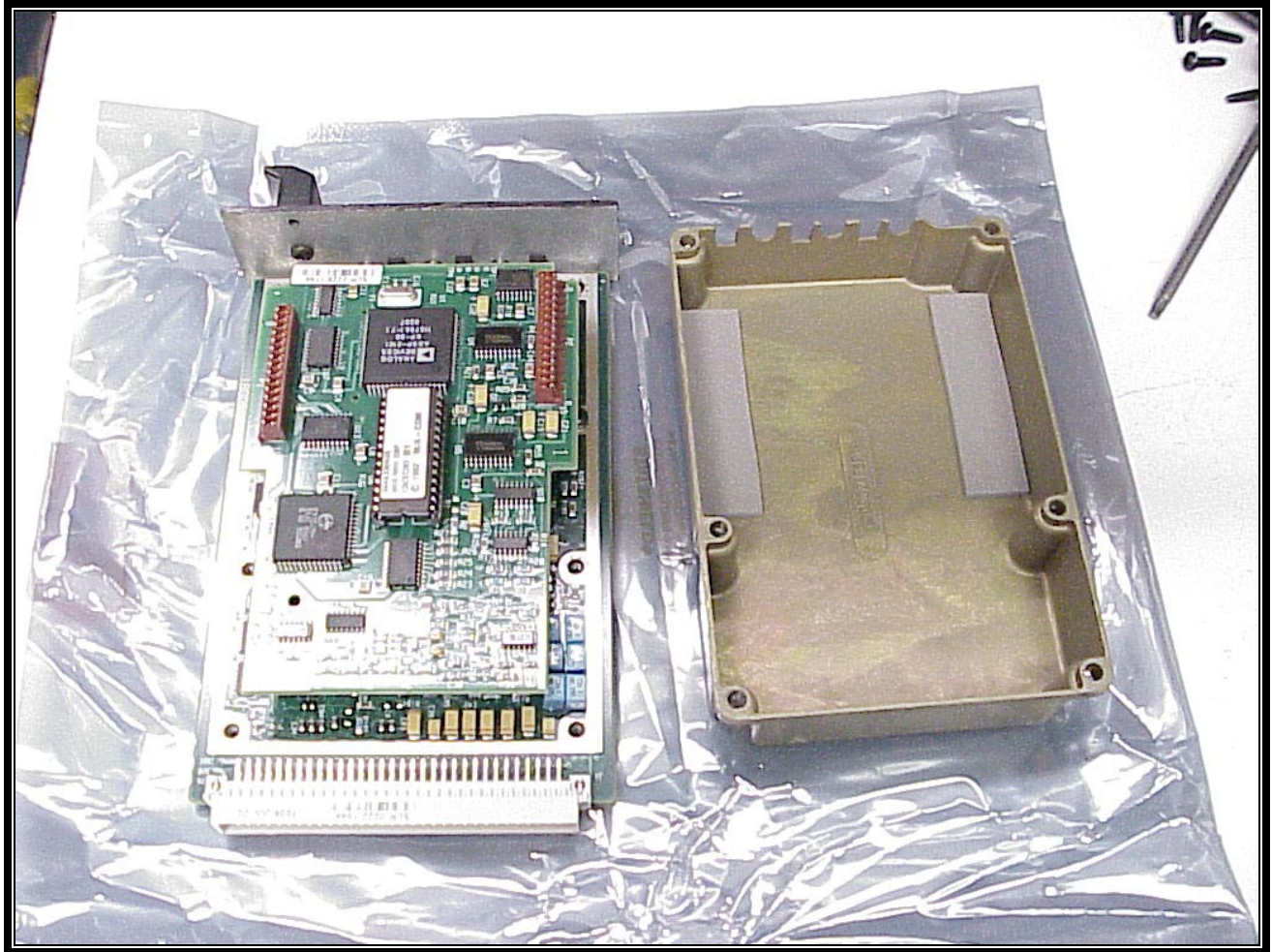
PHOTOGRAPH 29: SYSTEM MODULE COVER REMOVED
