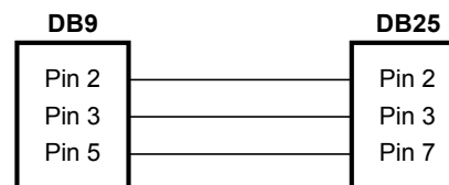
Figure 13 - 3-Wire Adapter
