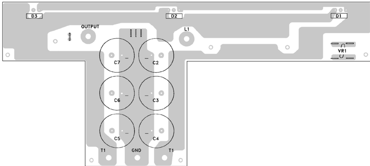
COMPONENT SIDE
