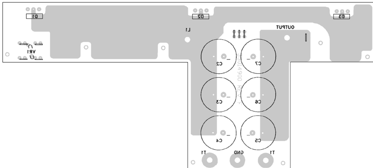
SOLDER SIDE
