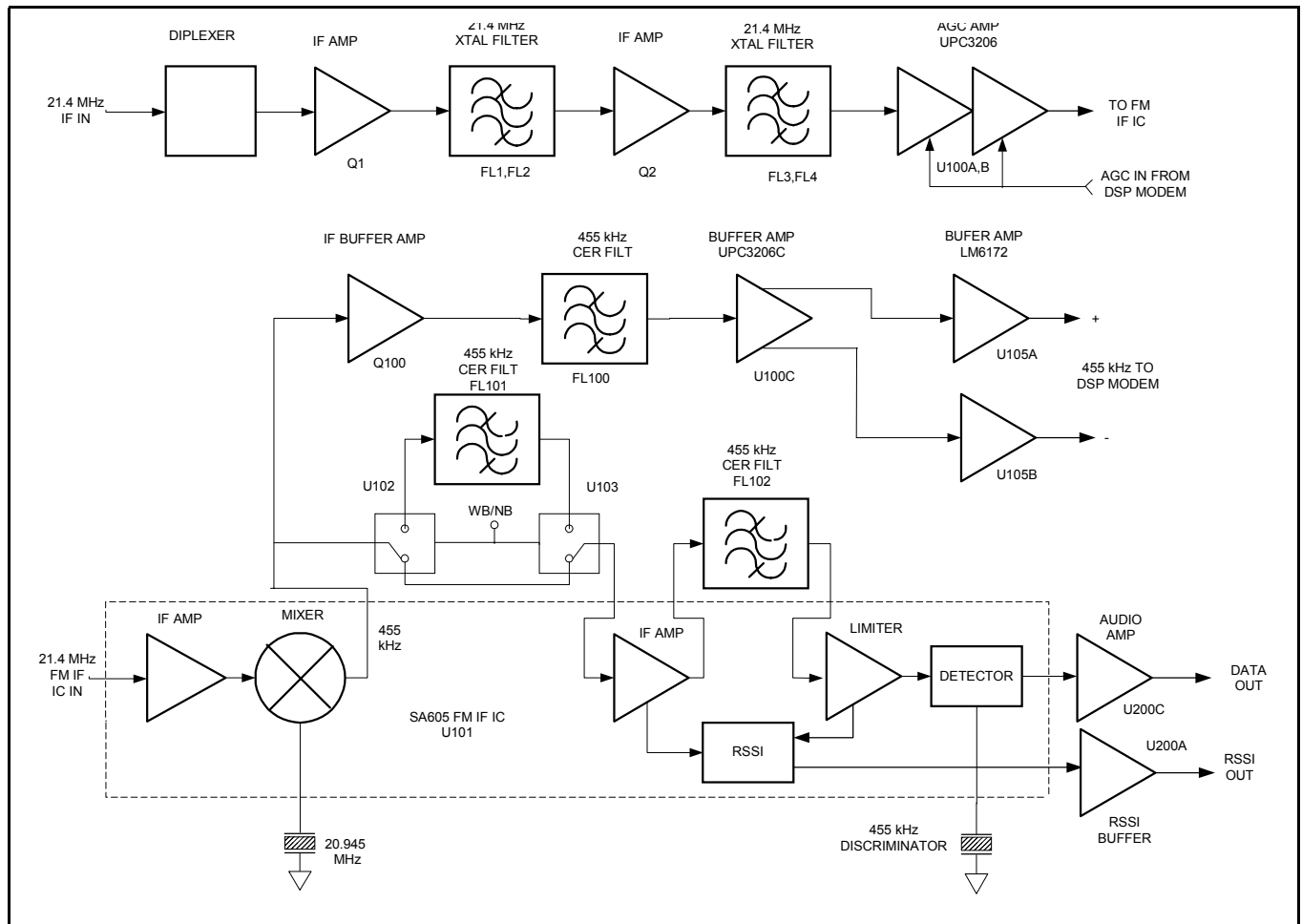
Figure 2 – 21.4 MHz IF Module Block Diagram
