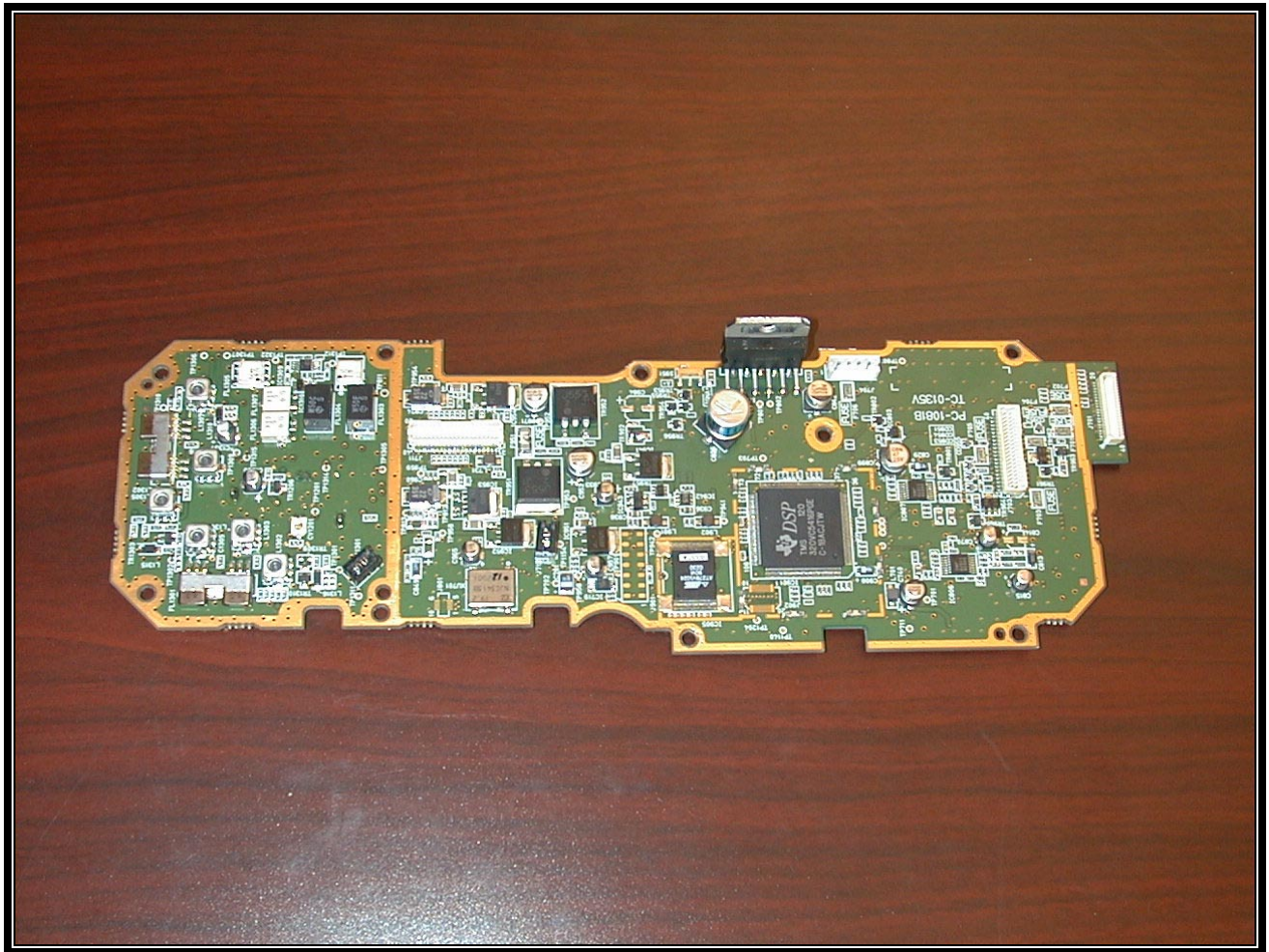
PHOTOGRAPH 13: AUDIO LOGIC BOARD TOP
