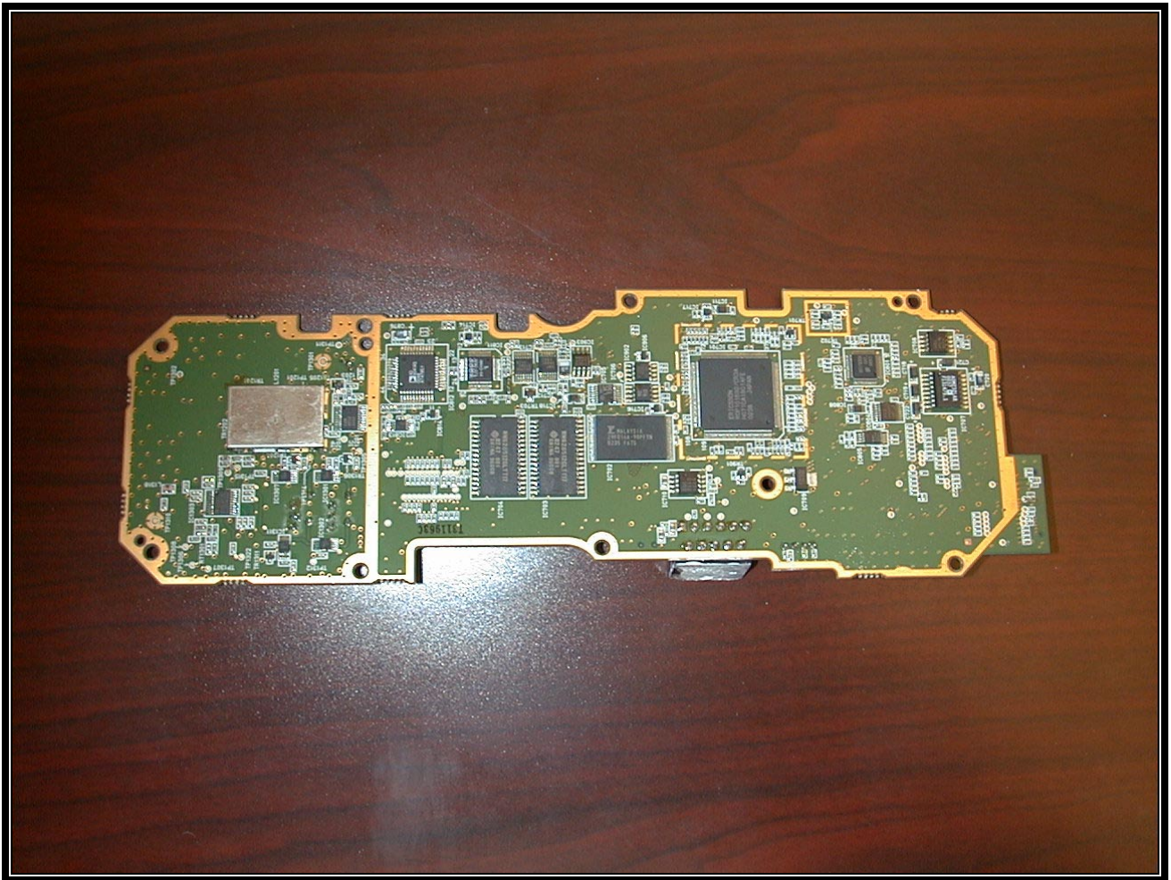
PHOTOGRAPH 14: AUDIO LOGIC BOARD BOTTOM
