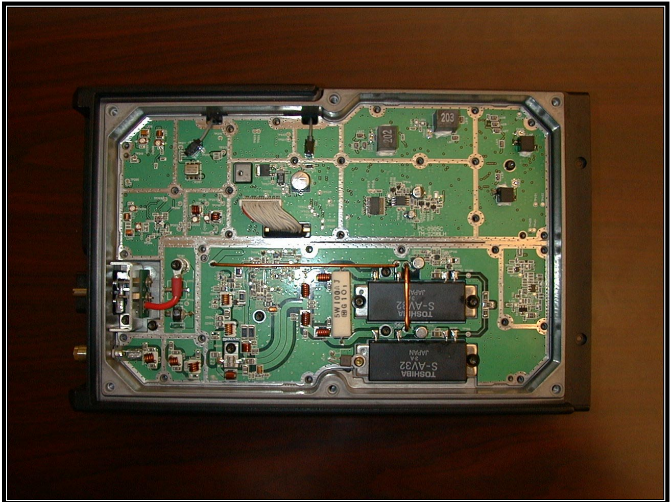
PHOTOGRAPH 15: TRANSMITTER & SYNTHESIZER – SHIELDS REMOVED
