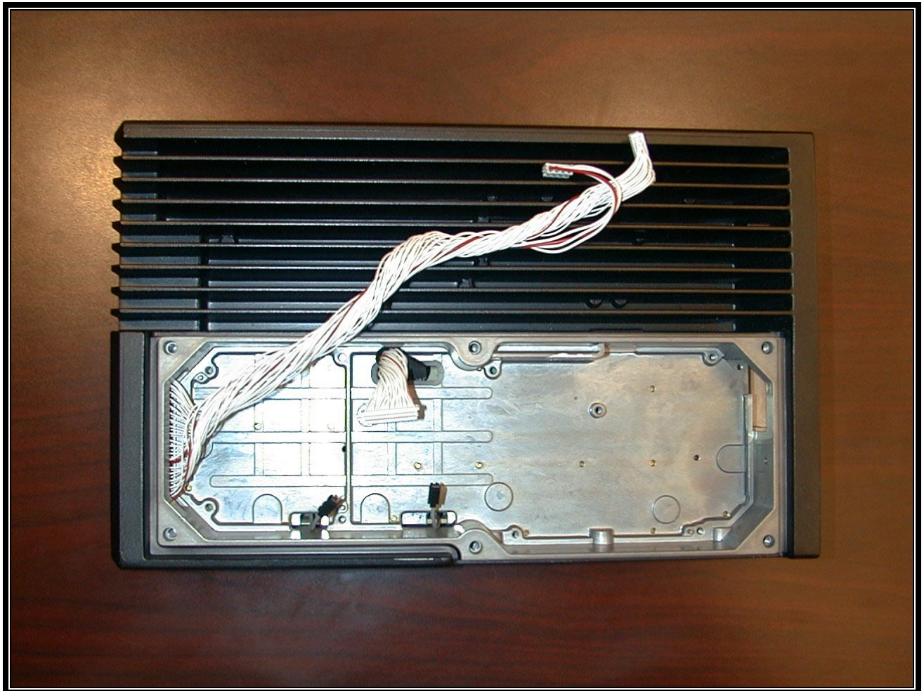
PHOTOGRAPH 12: AUDIO LOGIC BOARD REMOVED
