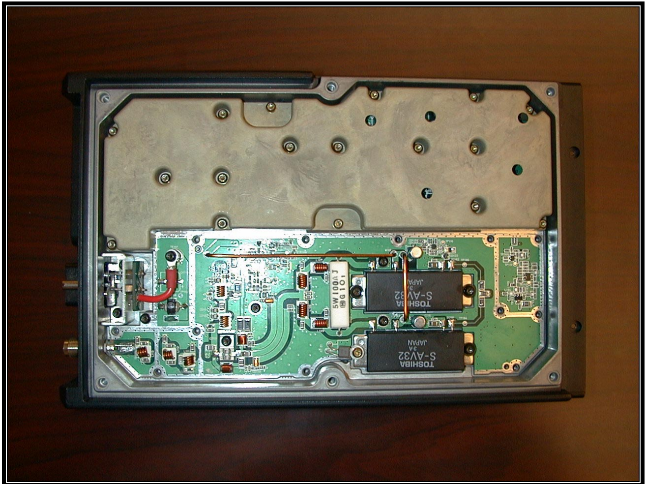
PHOTOGRAPH 16: TRANSMITTER - SHIELD REMOVED
