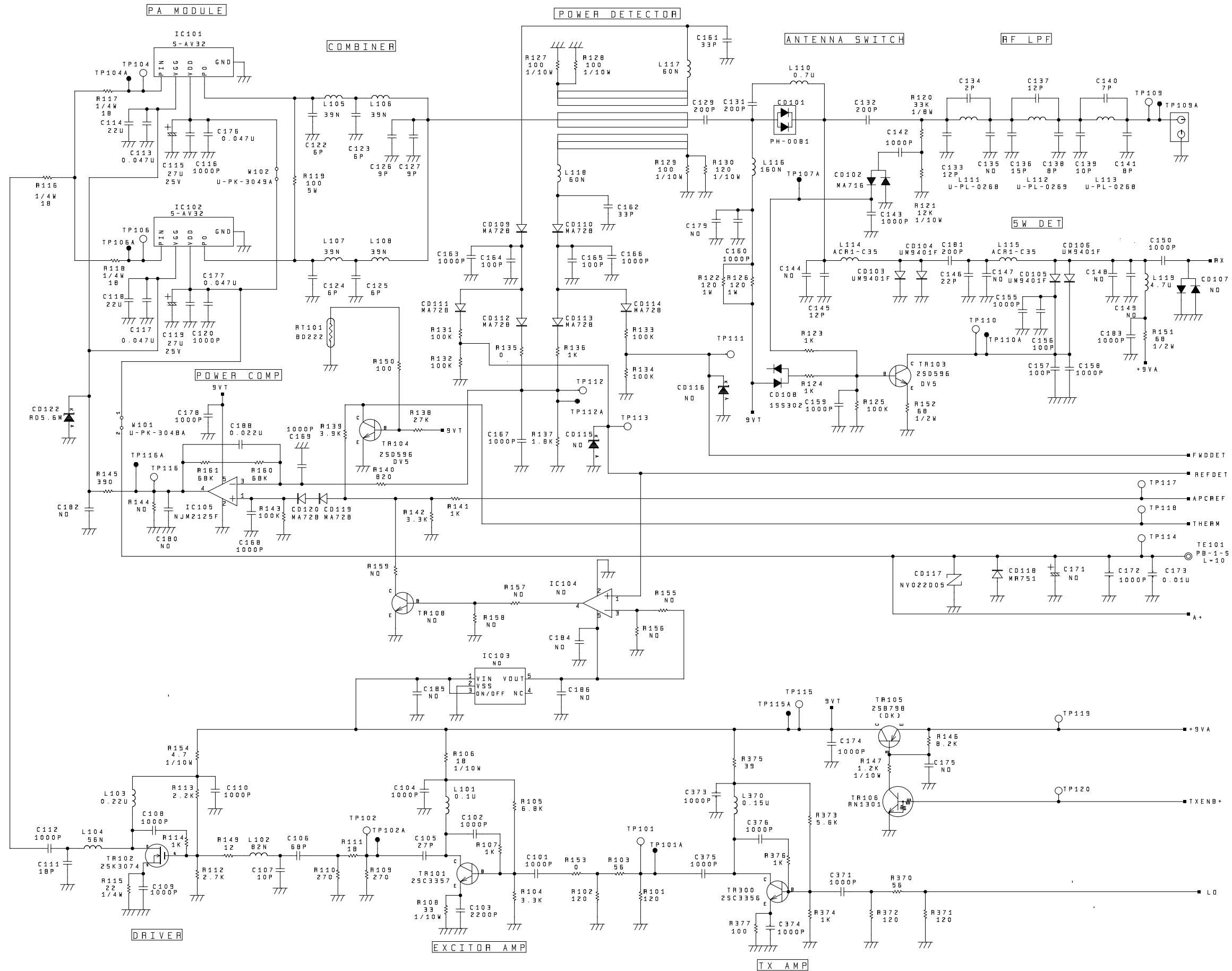
Schematic of M7100 VHF TRX/SYNTHESIZER UNIT TM-0298 EDCMN0018I
