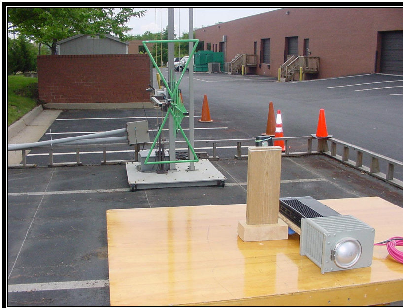
PHOTOGRAPH 3: RADIATED EMISSIONS REAR VIEW
