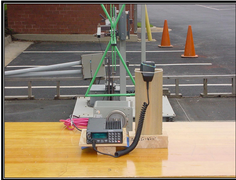
PHOTOGRAPH 2: RADIATED EMISSIONS FRONT VIEW
