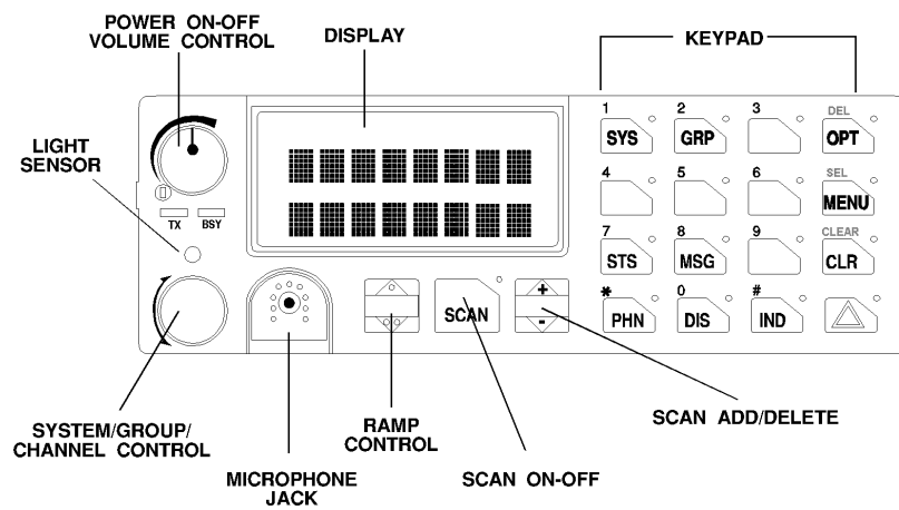
Figure 1 - M7100 IP Series Mobile Radio System Model Front Panel
