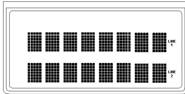
Figure 6 – M7100 IP Series Mobile Radio Display
