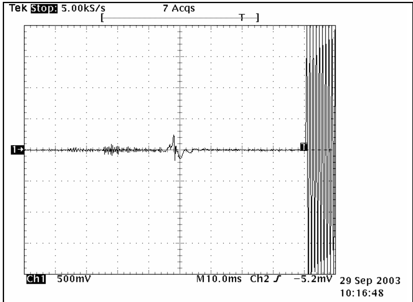
PLOT 13-2: TRANSIENT FREQUENCY BEHAVIOR – 404 MHZ; HIGH POWER; WIDE BAND; CARRIER OFF TIME
