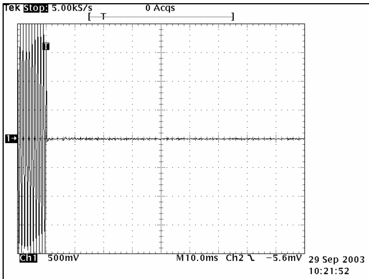
PLOT 13-1: TRANSIENT FREQUENCY BEHAVIOR – 404 MHZ; HIGH POWER; WIDE BAND; CARRIER ON TIME
