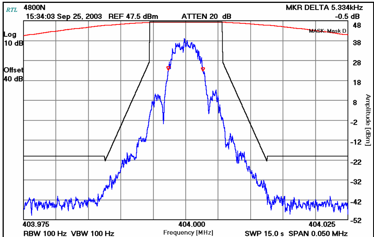
PLOT 8-5: 99% OCCUPIED BANDWIDTH - 2 LEVEL DIGITAL; NARROW BAND; 4800 BAUD
