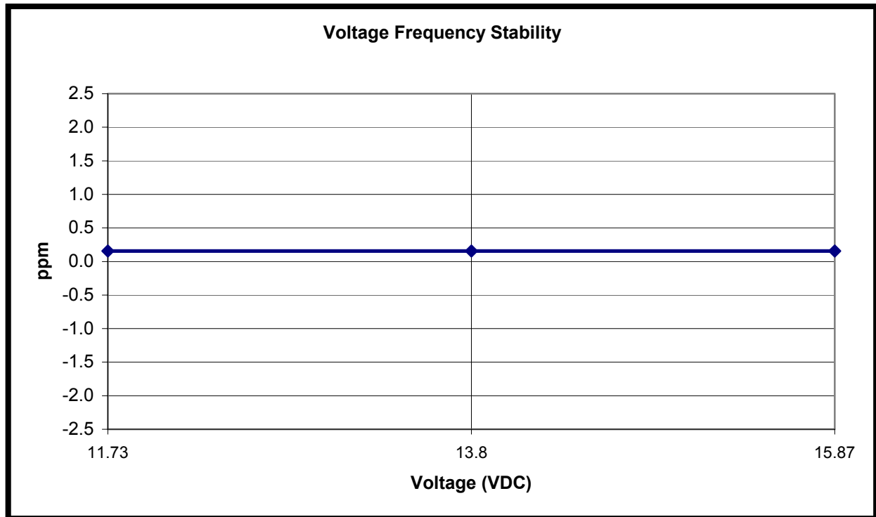
PLOT 9-2: VOLTAGE FREQUENCY STABILITY
