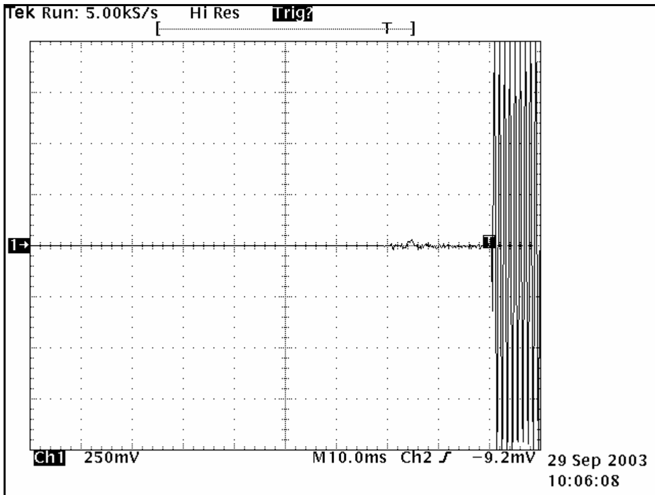
PLOT 13-4: TRANSIENT FREQUENCY BEHAVIOR – 404 MHZ; HIGH POWER; NARROW BAND; CARRIER OFF TIME
