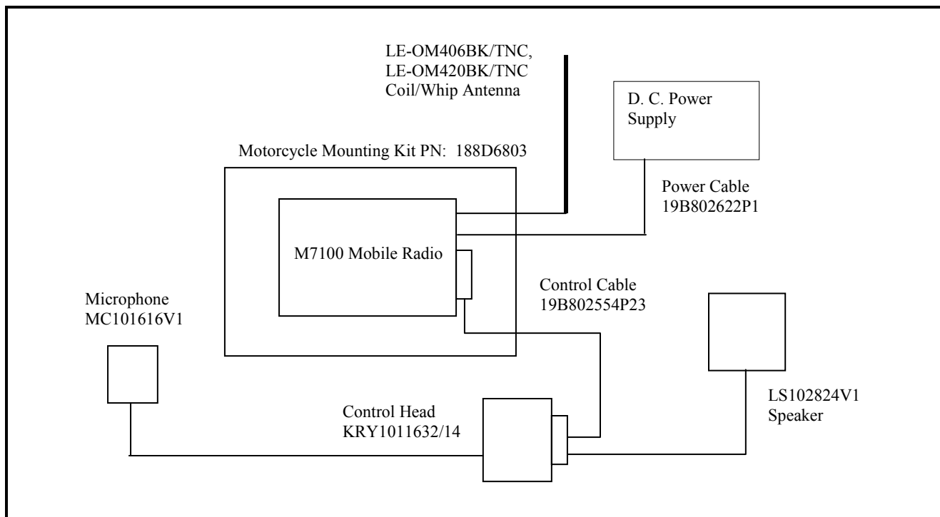
FIGURE 1: MOTORCYCLE OPTION CONFIGURATION
