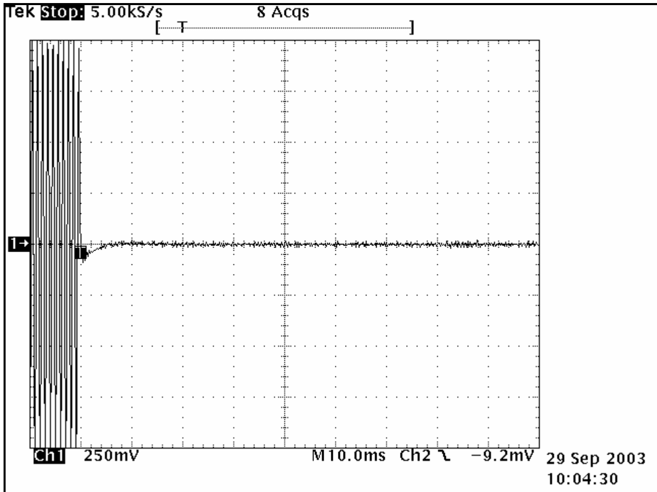
PLOT 13-3: TRANSIENT FREQUENCY BEHAVIOR – 404 MHZ; HIGH POWER; NARROW BAND; CARRIER ON TIME
