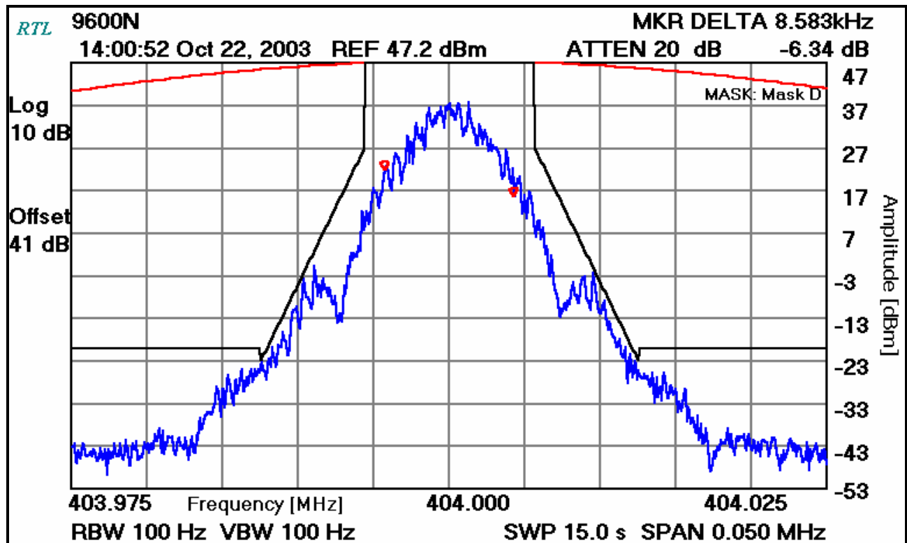
PLOT 8-4: 99% OCCUPIED BANDWIDTH - 2 LEVEL DIGITAL; NARROW BAND; 9600 BAUD
