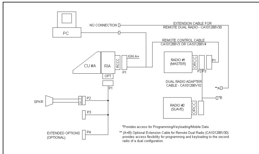
Figure 32 - M7100 IP Dual Radio Remote Mount/Remote Mount Installation Configuration
