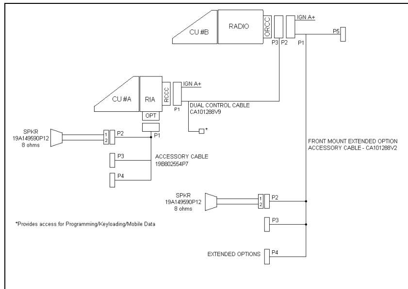
Figure 25 – M7100 IP Dual Control Unit Front Mount/Remote Mount Installation Configuration – Parallel Audio
