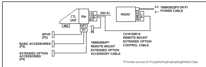
Figure 7 – Remote Mount Extended Option Accessory Interconnections
