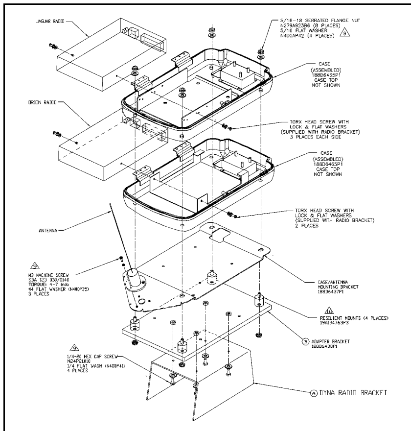
Figure 6-1: Radio Installation
