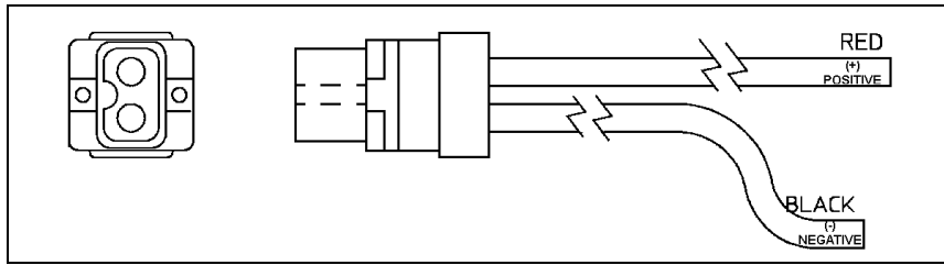
Figure 9-3: Power Cable 19B802622P1 or P3
