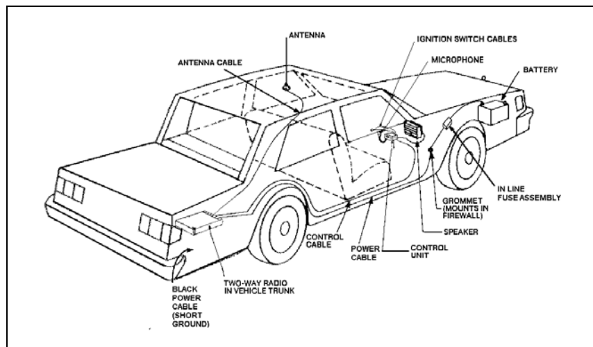
Figure 7-1: Typical Installation (Remote Mount Shown)
