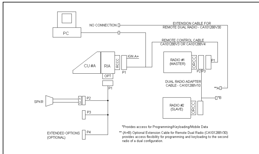
Figure 11-2: M7100 IP Dual Radio Remote Mount/Remote Mount Installation Configuration
