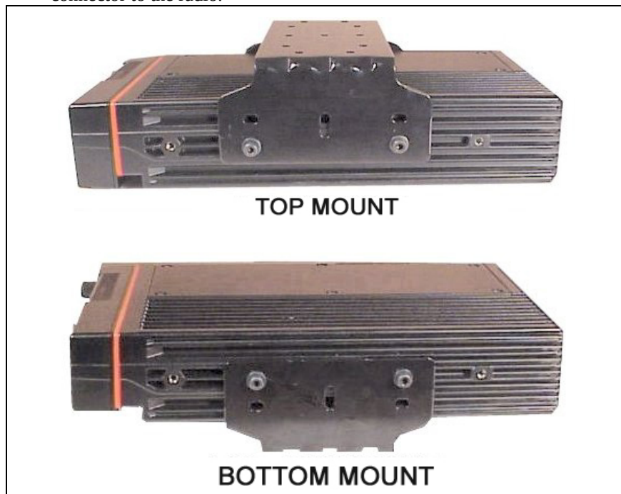
Figure 9-14: Mounting Bracket Installation (110W VHF Shown)
