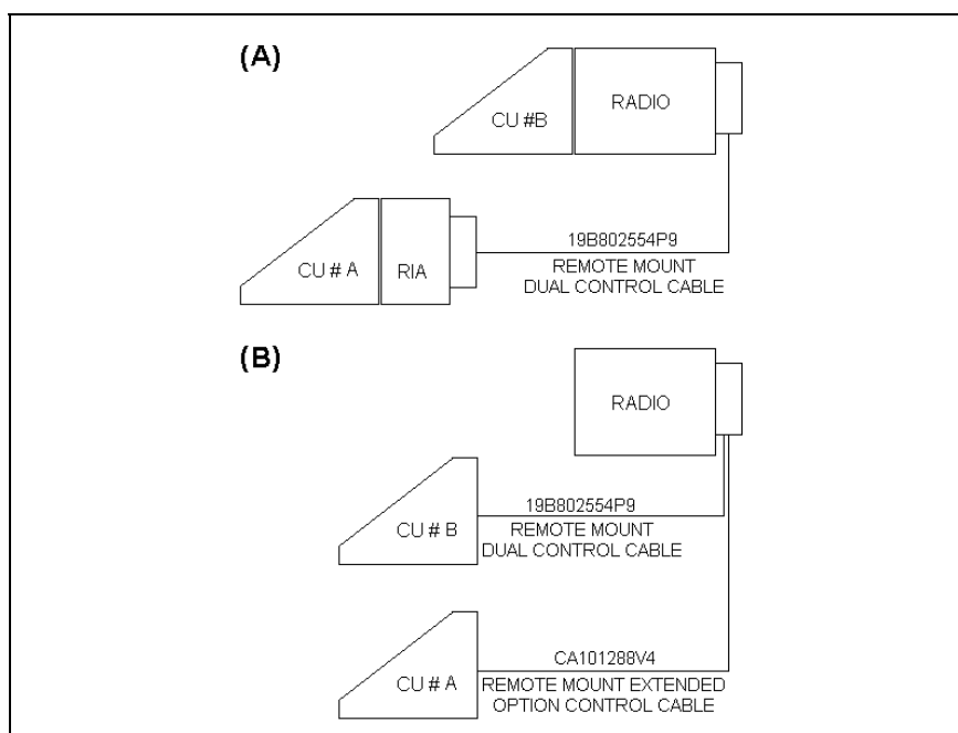
Figure 10-1: Dual Control Unit – Basic Configurations for Front Mount and Remote Mount Installations
