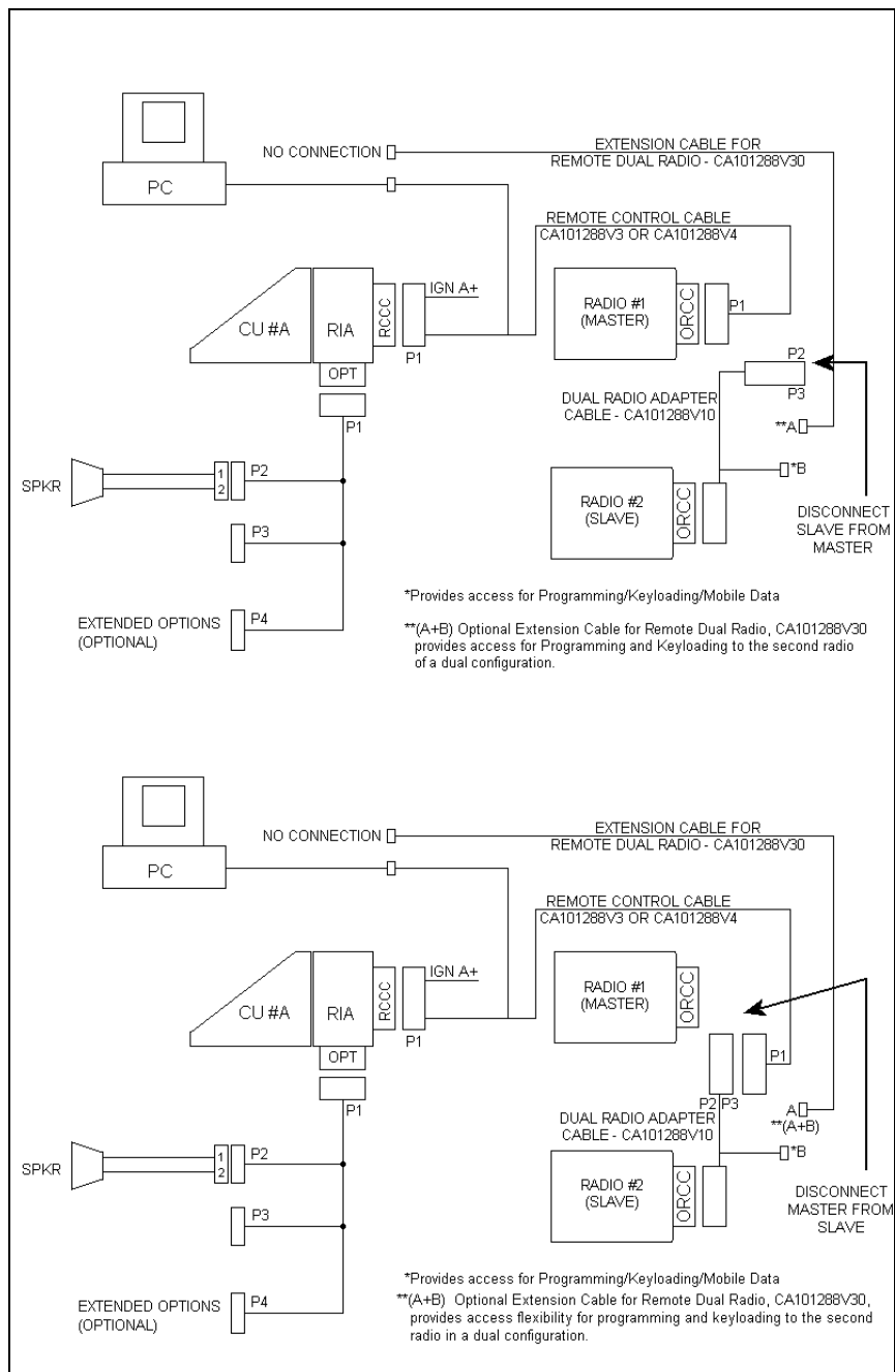
Figure 11-4: Dual Radio Configuration – Remote/Remote Mount PC Programming Procedure
