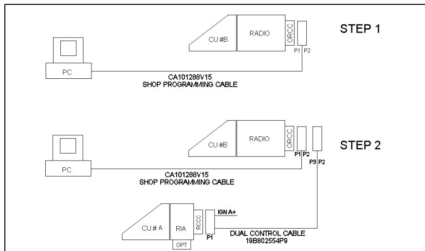
Figure 10-2: M7100 IP Dual Control Unit PC Programming Configuration
