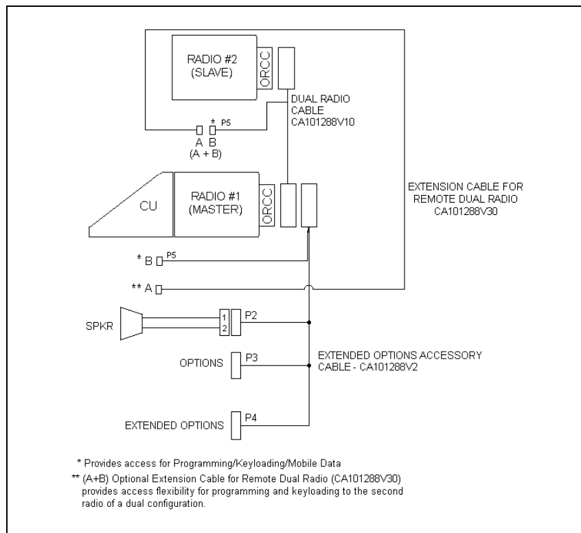
Figure 11-1: M7100 IP Dual Radio Front Mount/Remote Mount Installation Configuration
