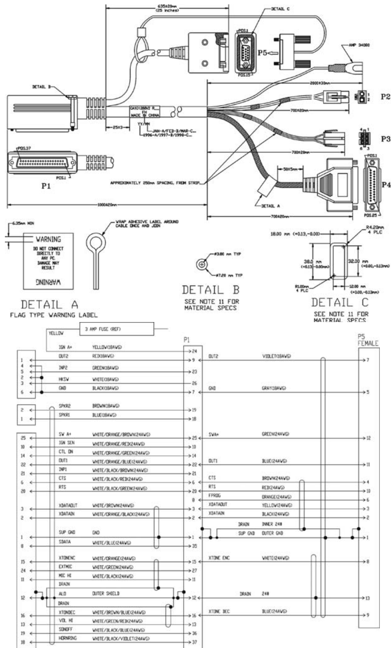
Figure 9-4 - Front Mount Extended Option Accessory Cable CA101288V2
