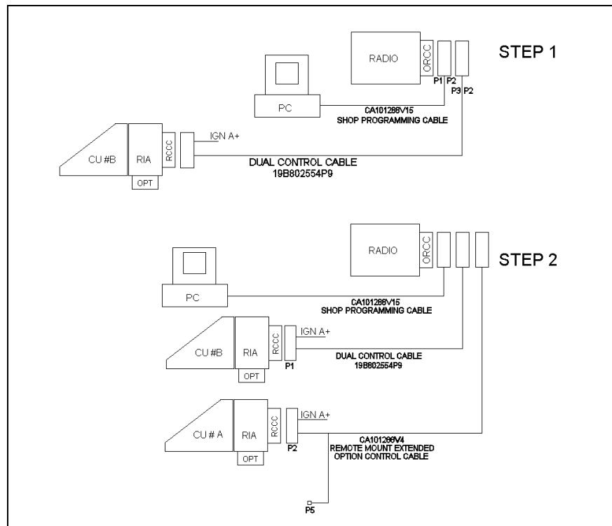
Figure 10-3: M7100 IP Dual Control Unit PC Programming Configuration Remote Mount
