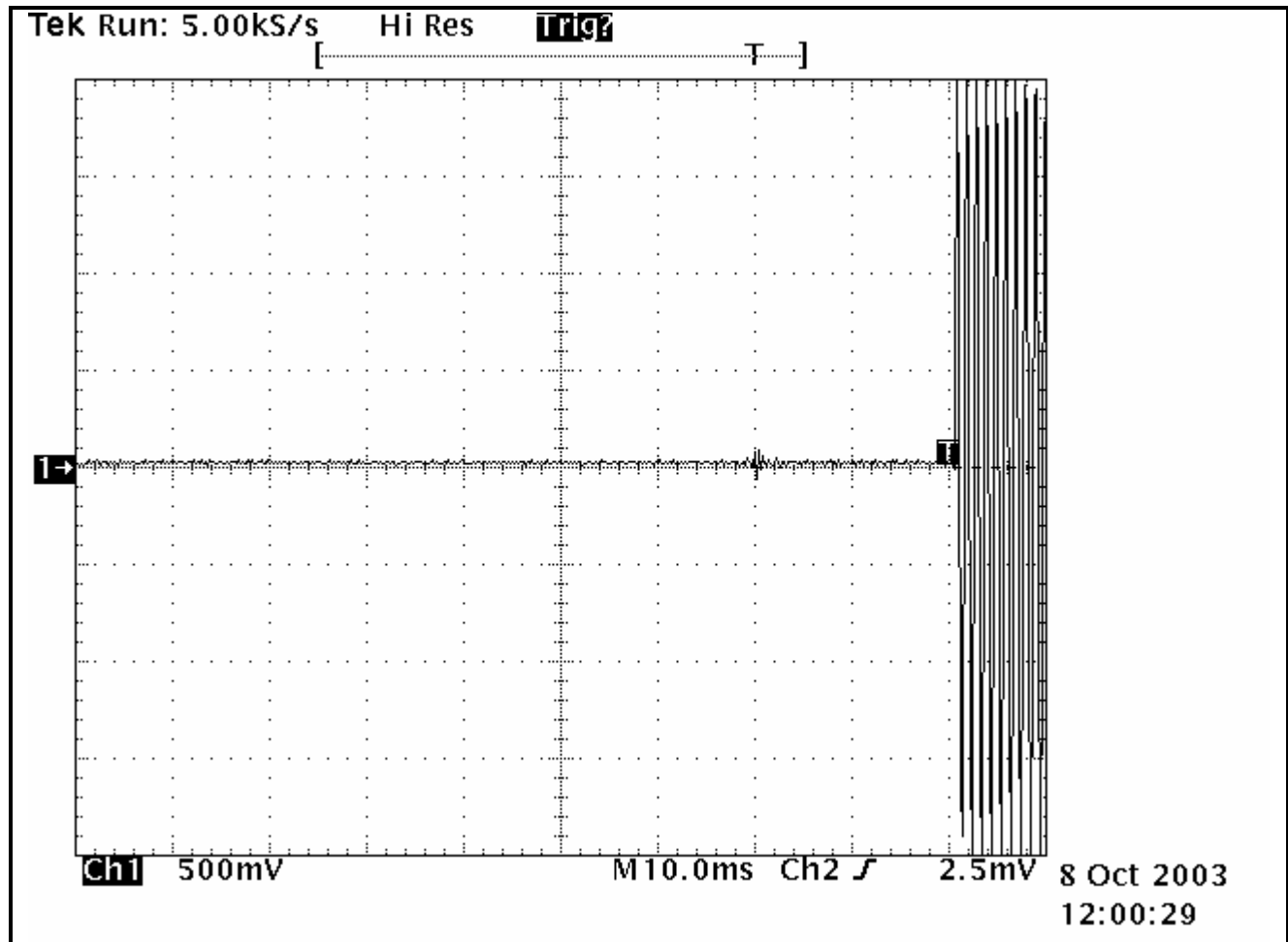
PLOT 13-2: TRANSIENT FREQUENCY BEHAVIOR – 500 MHZ; HIGH POWER; WIDE BAND; CARRIER OFF TIME
