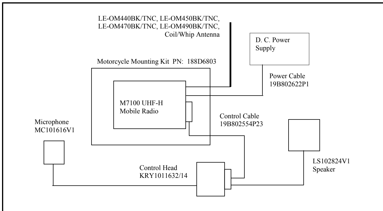
FIGURE 3-1: MOTORCYCLE OPTION CONFIGURATION
