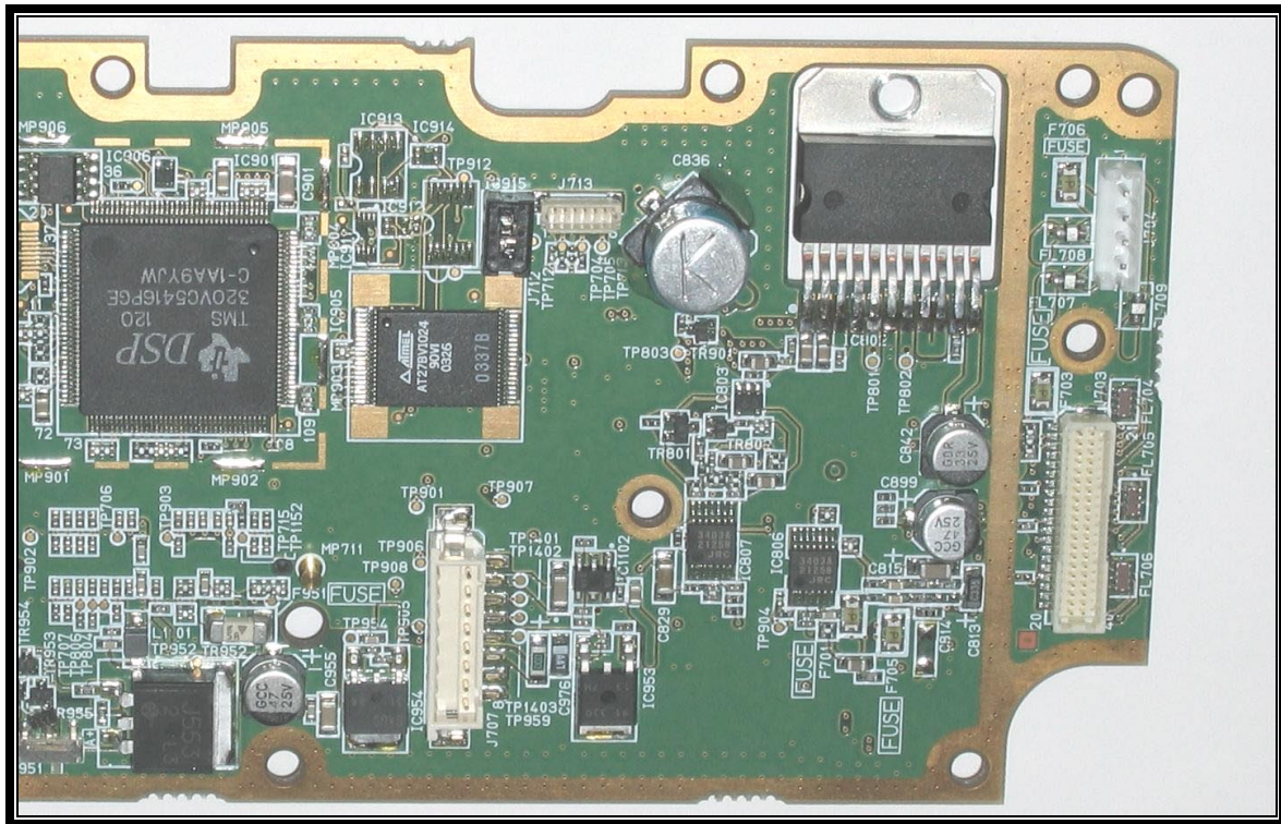
PHOTOGRAPH 13: AUDIO LOGIC BOARD COMPONENT SIDE, RIGHT SIDE
