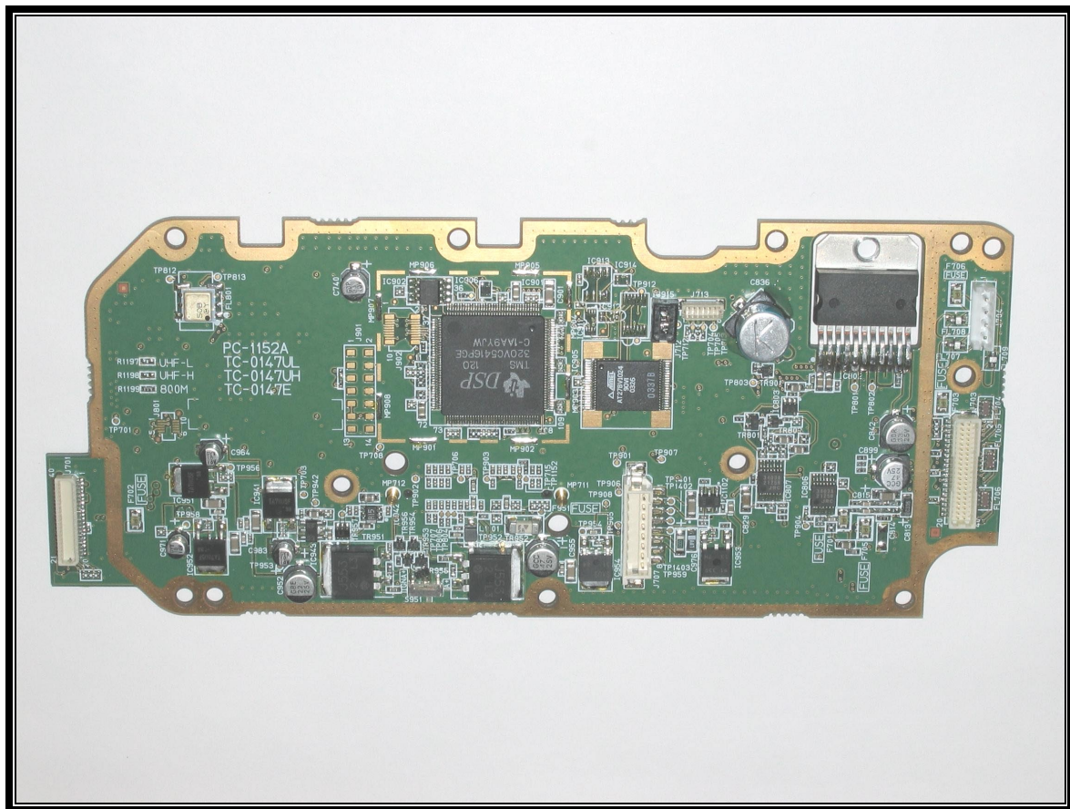
PHOTOGRAPH 11: AUDIO LOGIC BOARD COMPONENT SIDE, COMPLETE VIEW
