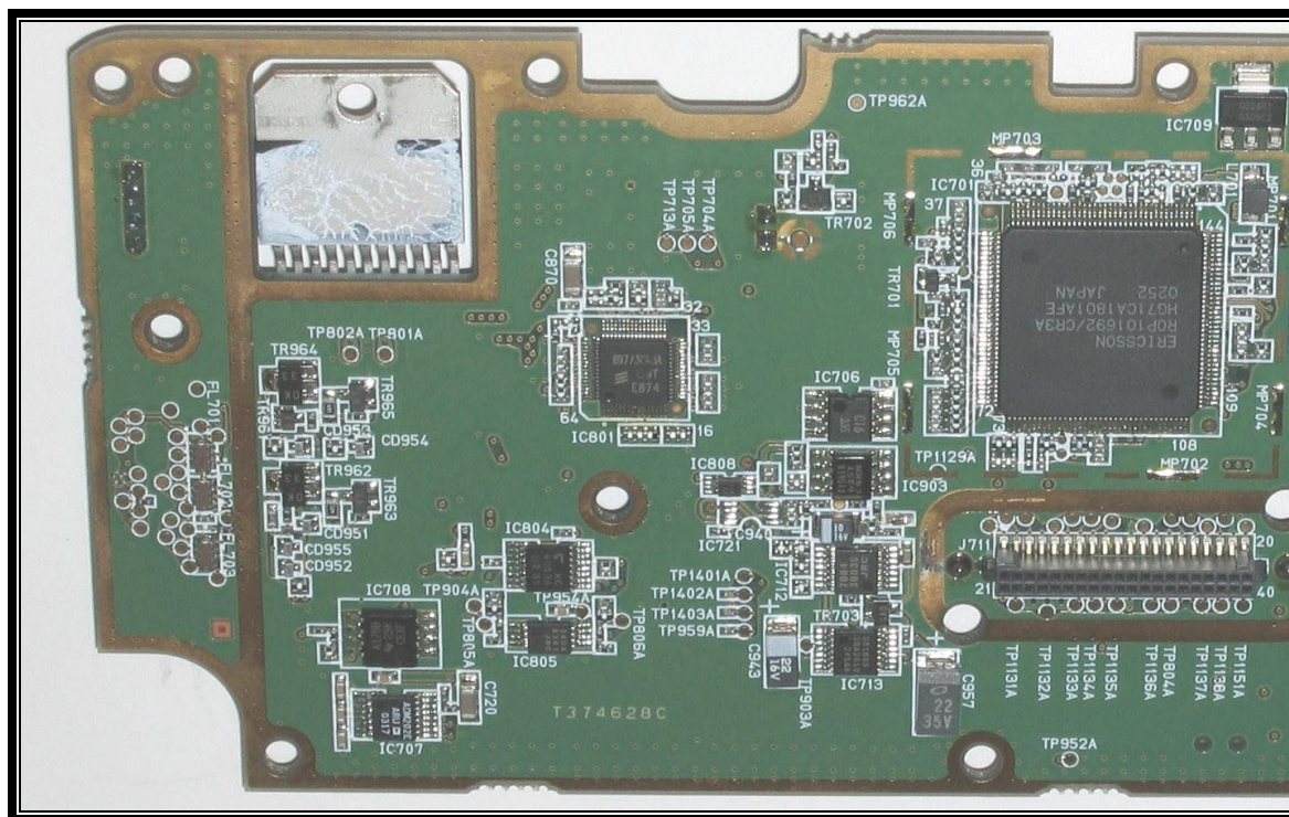
PHOTOGRAPH 15: AUDIO LOGIC BOARD SOLDER SIDE, LEFT SIDE
