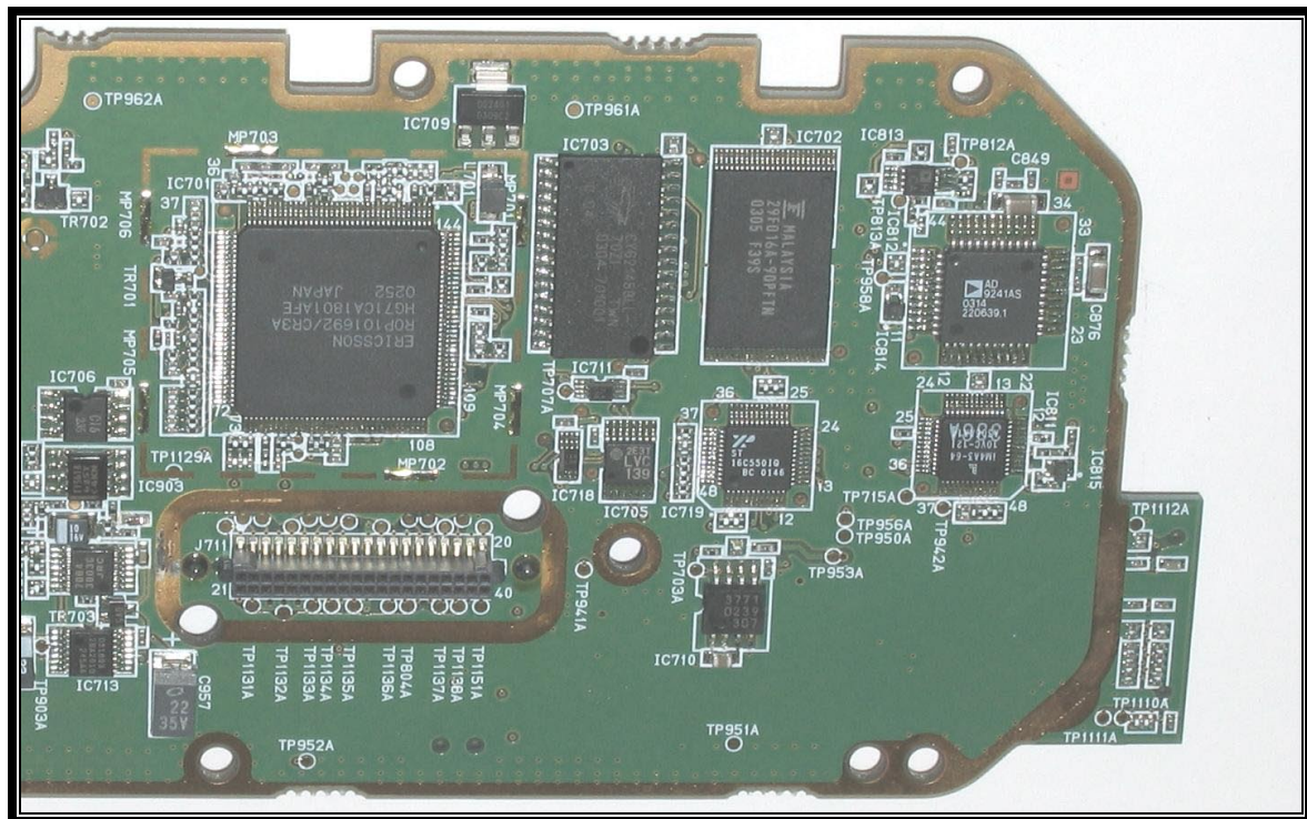
PHOTOGRAPH 16: AUDIO LOGIC BOARD SOLDER SIDE, RIGHT SIDE
