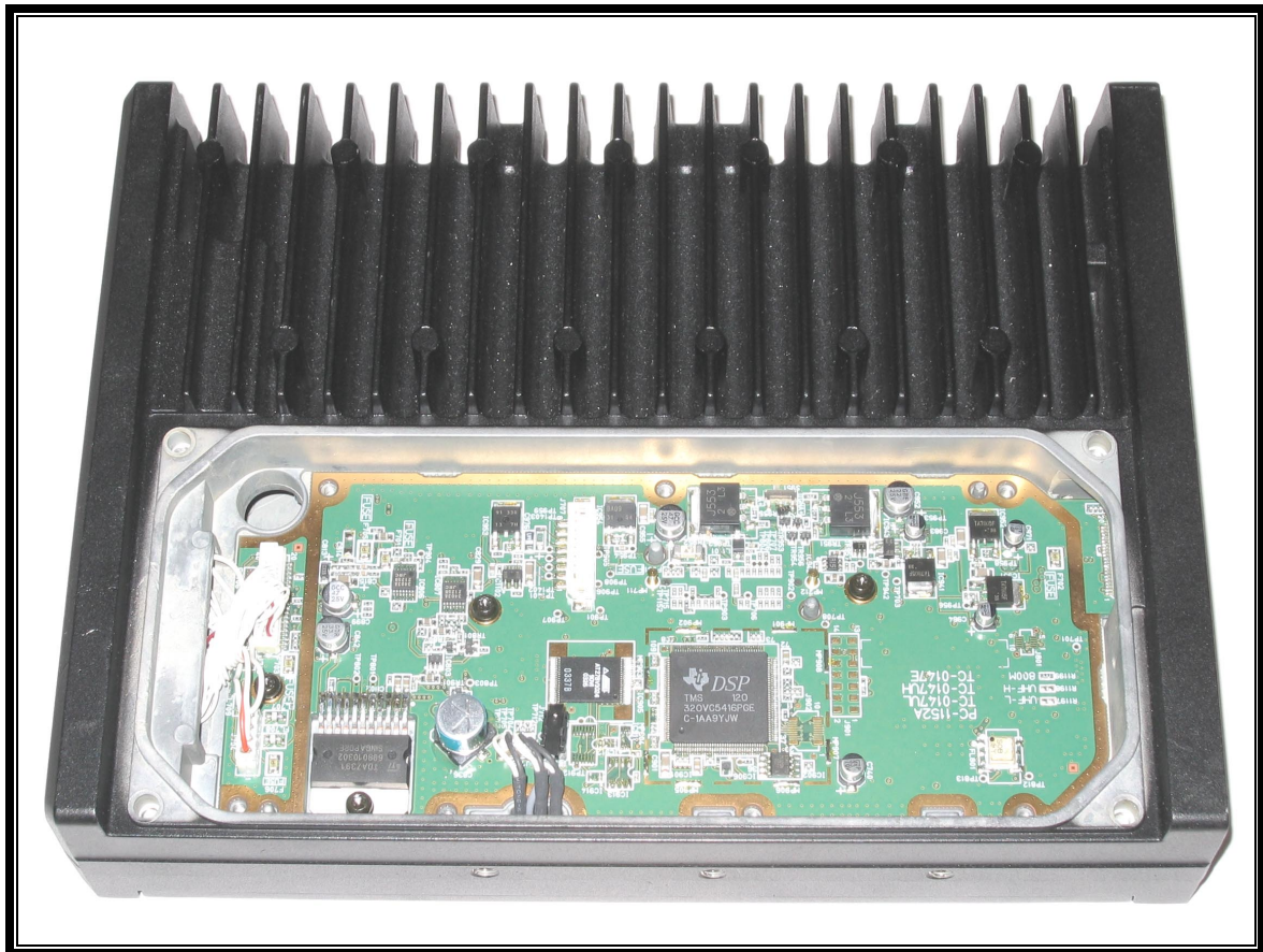
PHOTOGRAPH 17: TOP COVER AND INNER SHIELD REMOVED
