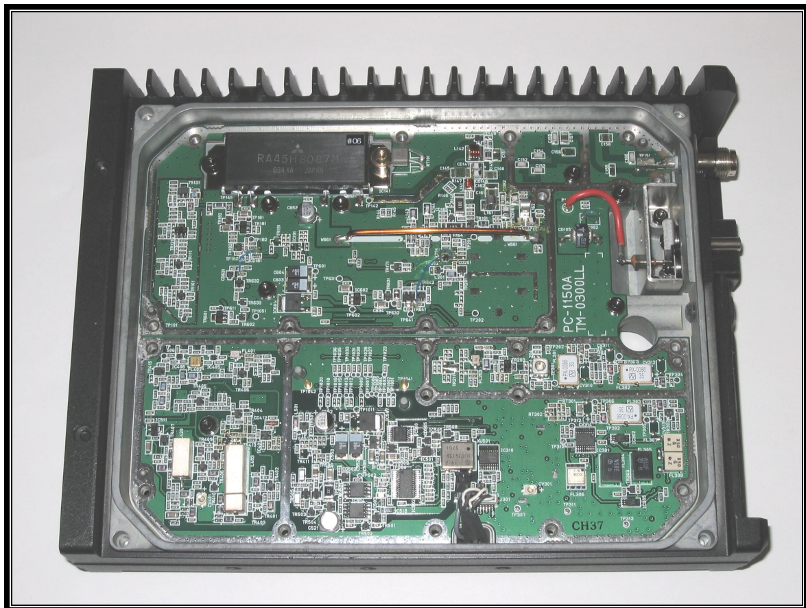
PHOTOGRAPH 10: BOTTOM COVER AND INNER SHIELD REMOVED
