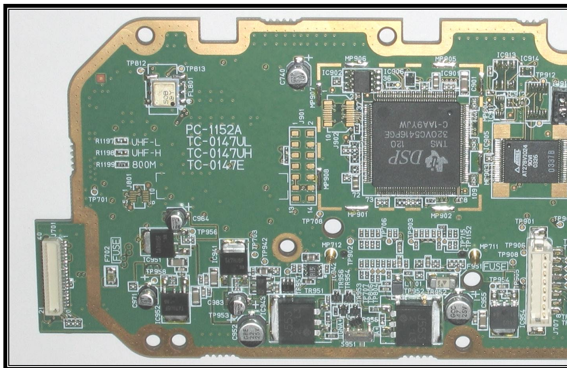
PHOTOGRAPH 12: AUDIO LOGIC BOARD COMPONENT SIDE, LEFT SIDE
