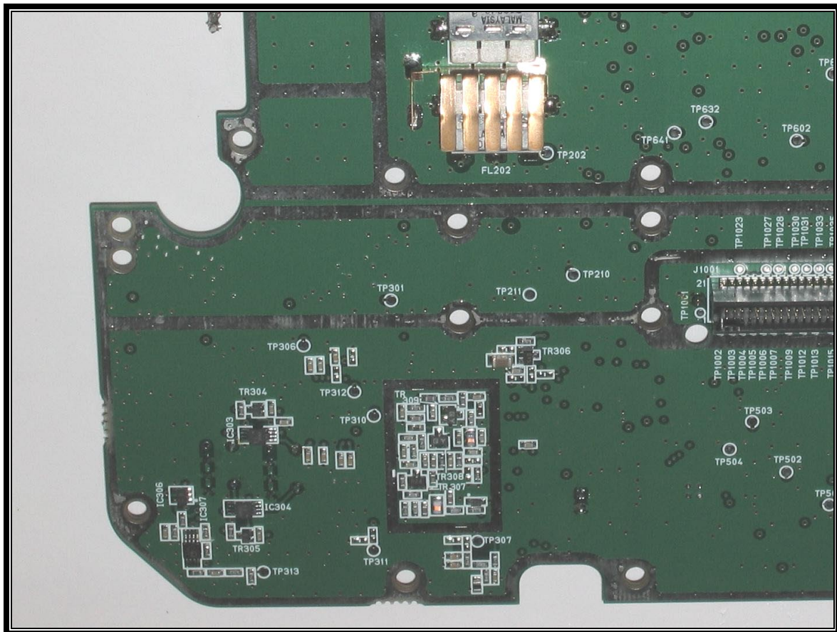
PHOTOGRAPH 24: TRX SYN BOARD SOLDER SIDE, LOWER LEFT
