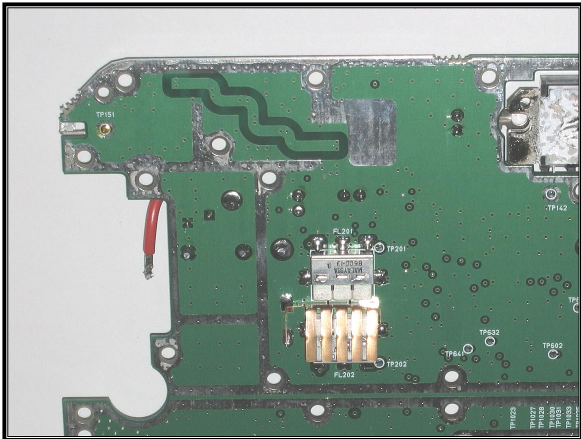
PHOTOGRAPH 26: TRX SYN BOARD SOLDER SIDE, UPPER LEFT
