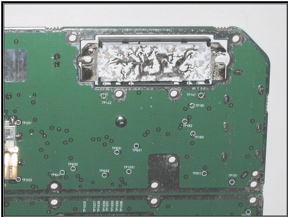
PHOTOGRAPH 27: TRX SYN BOARD SOLDER SIDE, UPPER RIGHT
