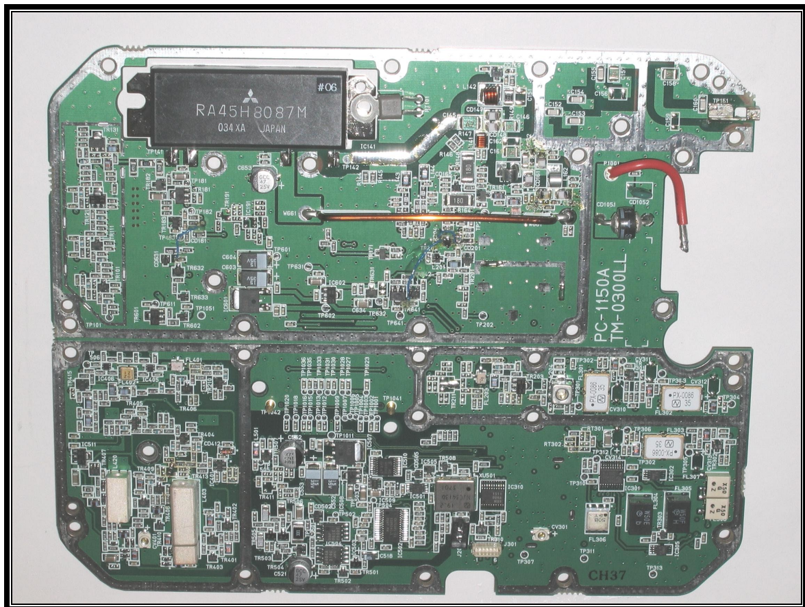
PHOTOGRAPH 18: TRX SYN BOARD COMPONENT SIDE, COMPLETE VIEW
