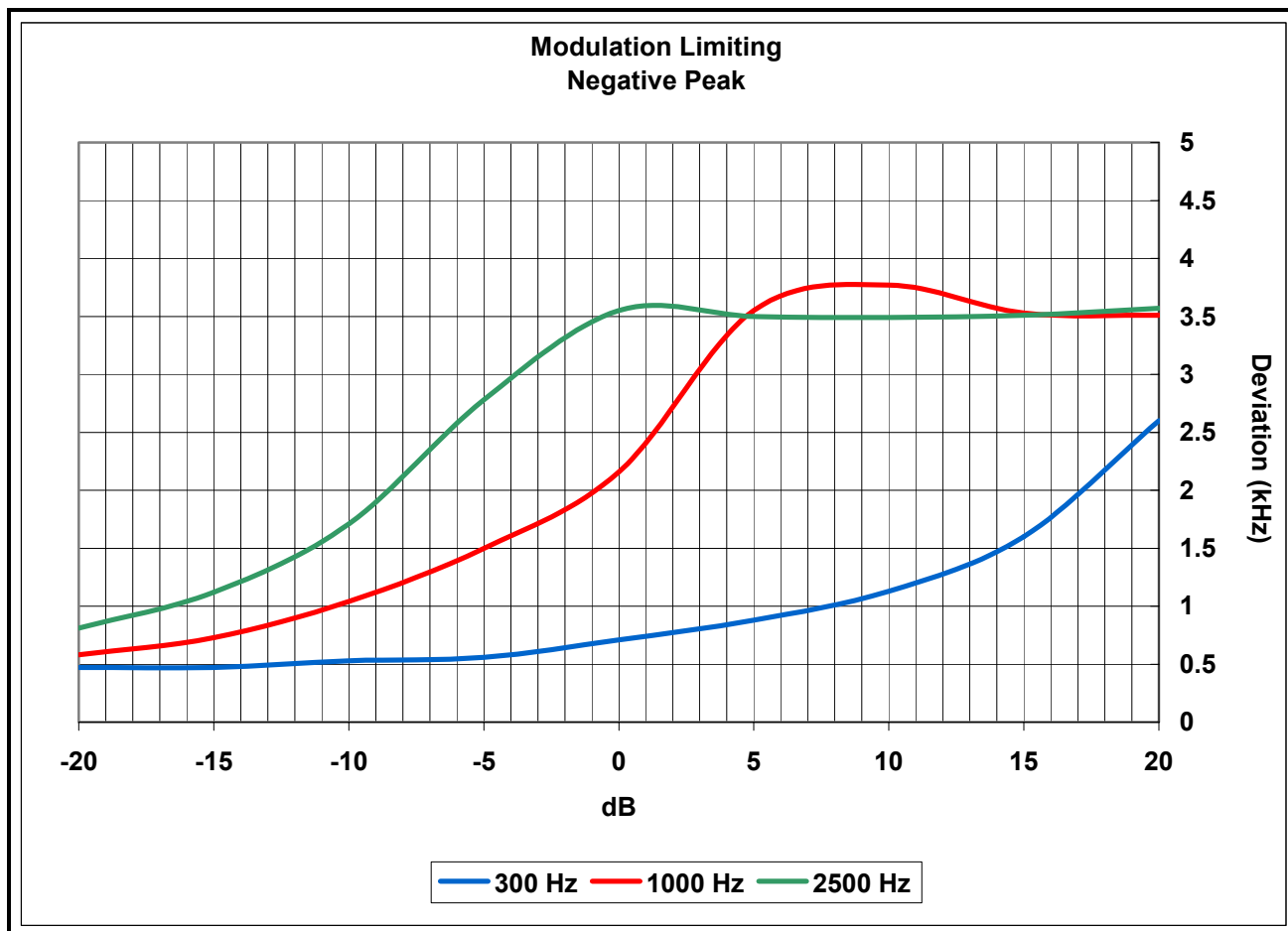
PLOT 12-4: MODULATION CHARACTERISTICS – MODULATION LIMITING: NPSPAC; NEGATIVE PEAK
