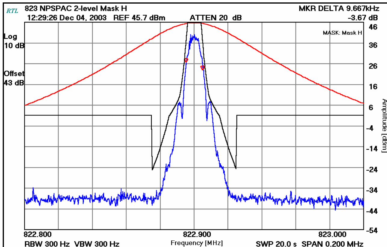
PLOT 8-7: 99% OCCUPIED BANDWIDTH – 2-LEVEL; NPSPAC; 9600; (MASK H)
