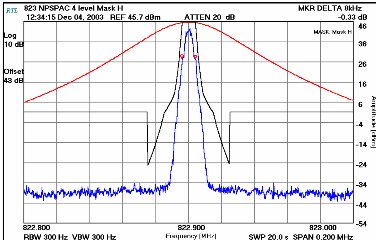
PLOT 8-12: 99% OCCUPIED BANDWIDTH – 4-LEVEL; NPSPAC; (MASK H)
