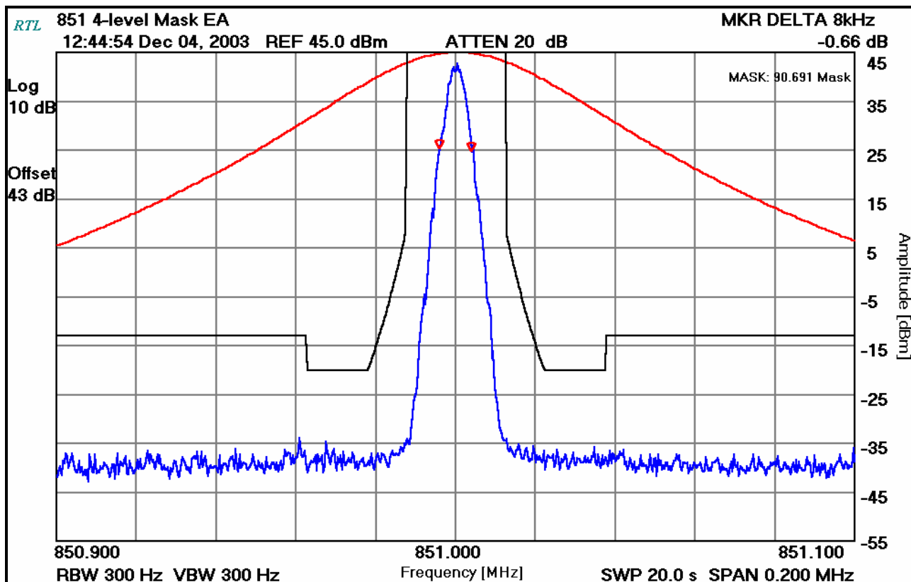
PLOT 8-13: 99% OCCUPIED BANDWIDTH – 4-LEVEL; (MASK EA)
