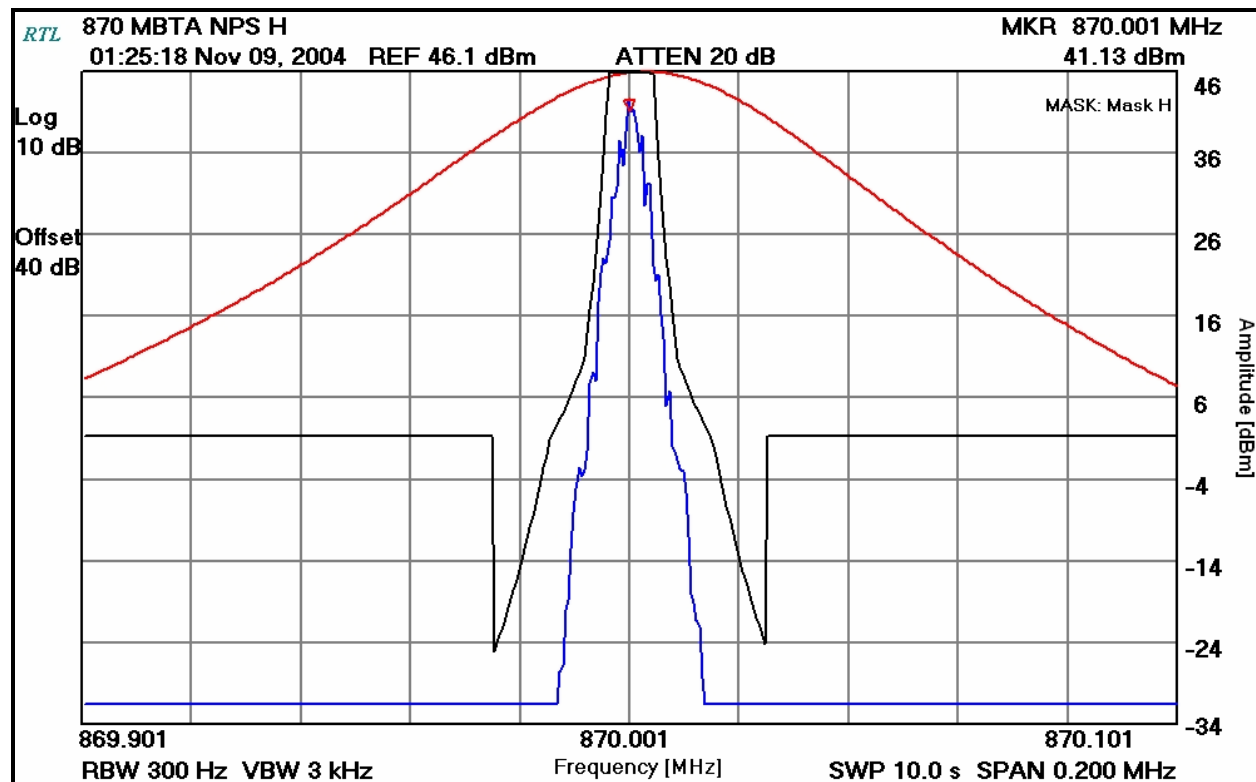
PLOT 5: 870.0 MHZ NPS DATA – MASK H
