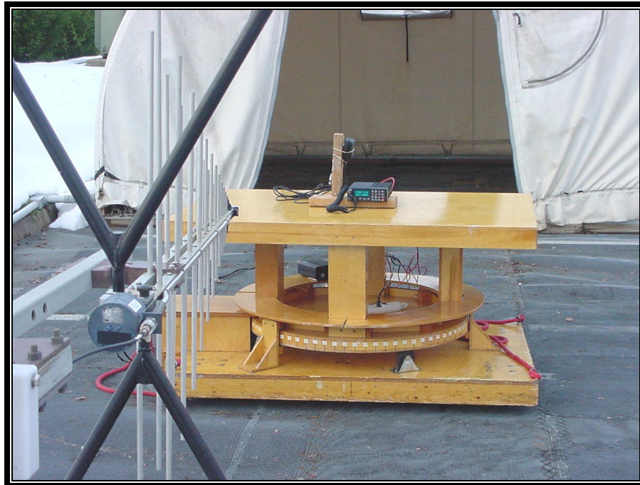
PHOTOGRAPH 3: RADIATED EMISSIONS – STANDARD CONFIGURATION
