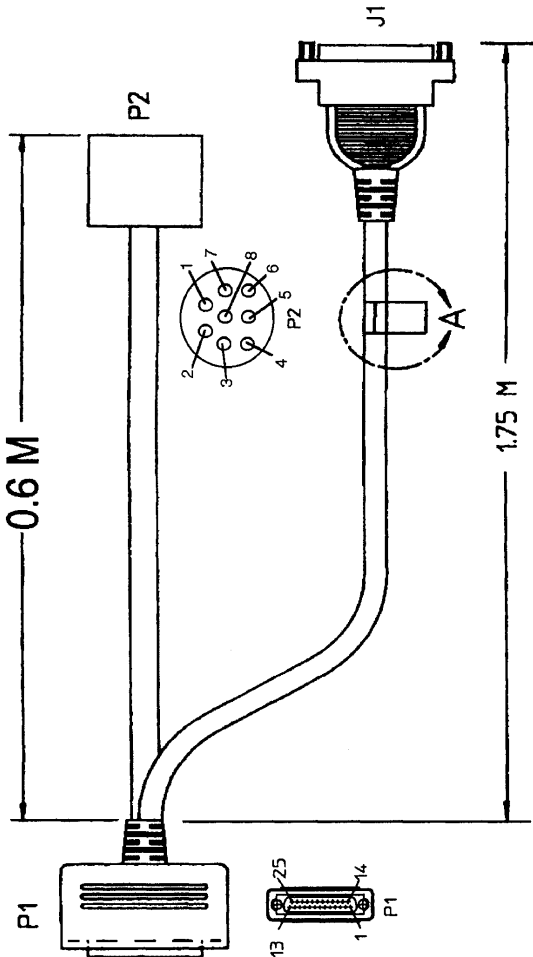
Motorcycle Accessory Cable (19B802554P24, Sh. 24, Rev. 27)
