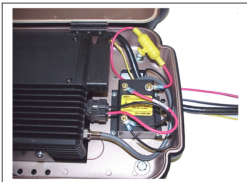
Figure 6-4: Radio Connections
