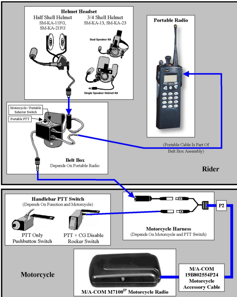
Figure 8-1: Headset Option with M7100 IP Mobile Radio with Portable Radio (P7100 IP shown)
