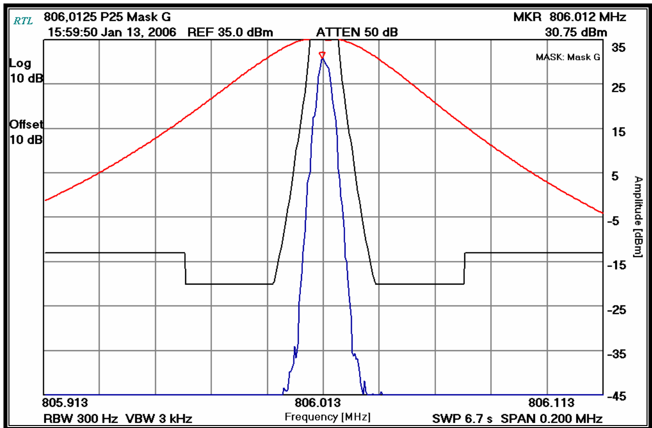
Plot 8-13: 99% Occupied Bandwidth – 4-level; (Mask G)
