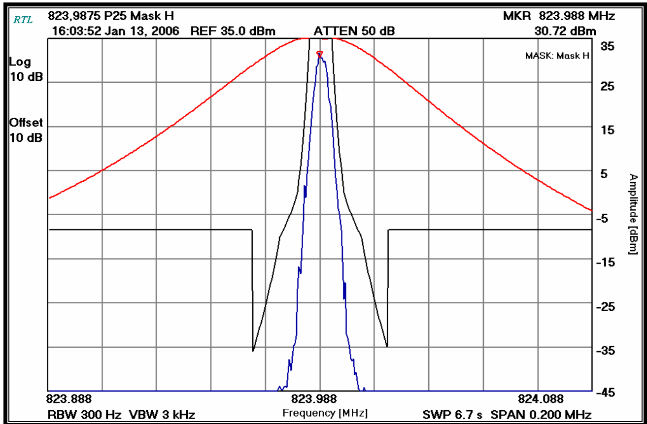
Plot 8-15: 99% Occupied Bandwidth – 4-level; (Mask H)
