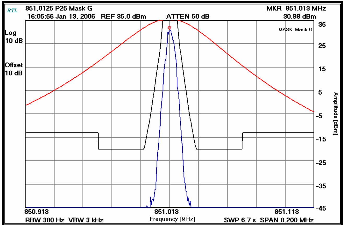
Plot 8-16: 99% Occupied Bandwidth – 4-level; (Mask g)
