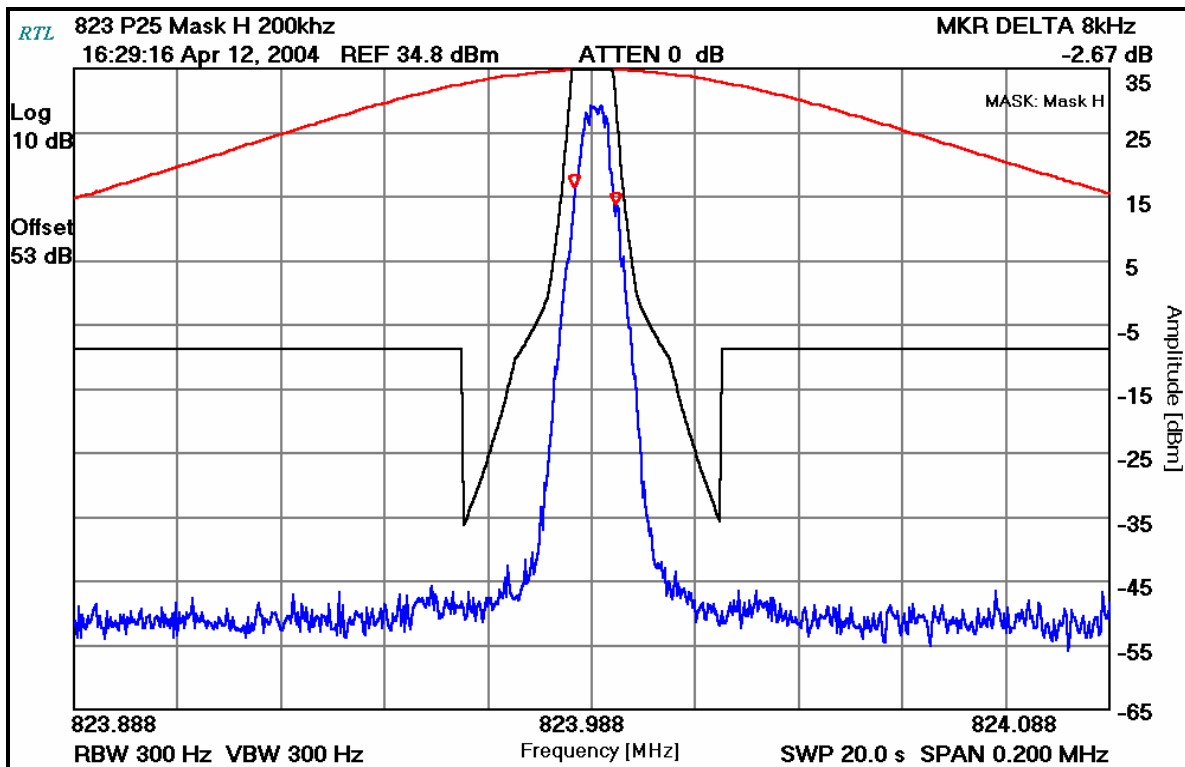
PLOT 8-15: 99% OCCUPIED BANDWIDTH - 4-LEVEL; (MASK H)
