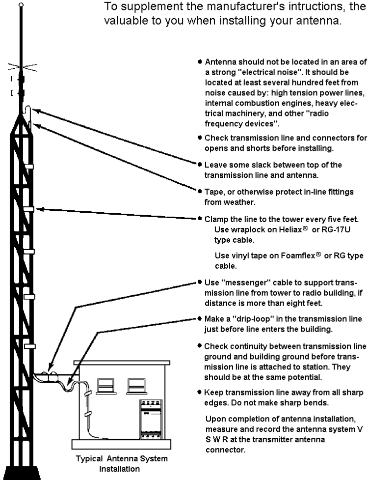
Figure 14 - Antenna Installation
