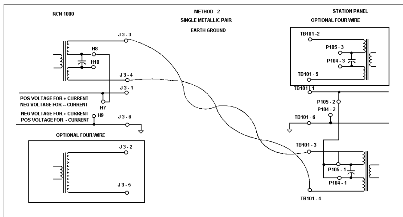
Figure 9 - METHOD 2 (Single Metallic, Earth Ground)
