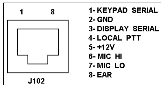
Figure 5 - Microphone Connections
