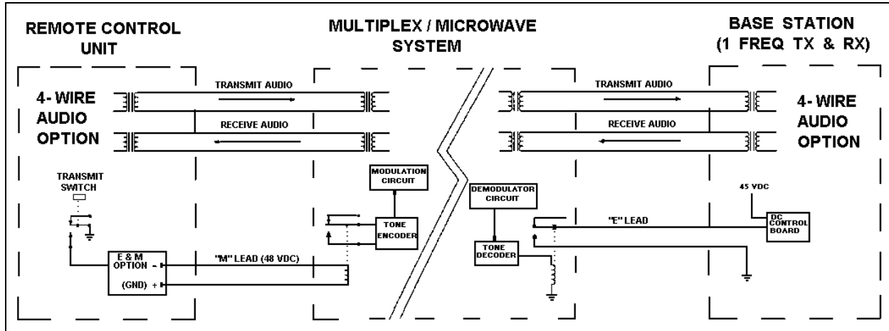
Figure 7 - Typical E &amp; M Signaling Application
