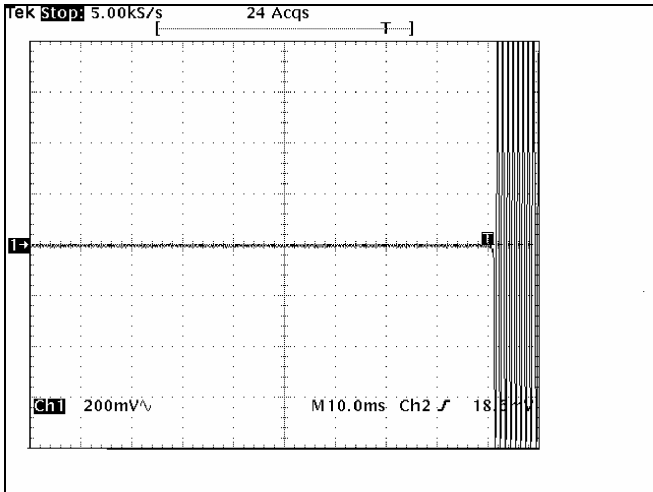
PLOT 13-4: TRANSIENT FREQUENCY BEHAVIOR – 420.525 MHZ; HIGH POWER; NARROW BAND; CARRIER OFF TIME
