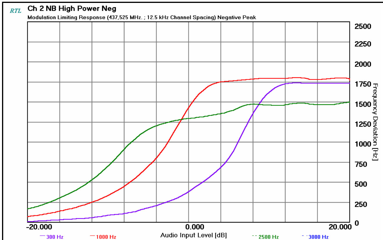
PLOT 12-4: MODULATION CHARACTERISTICS – MODULATION LIMITING: NARROW BAND; NEGATIVE PEAK
