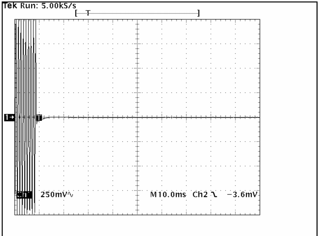
PLOT 13-3: TRANSIENT FREQUENCY BEHAVIOR – 460.525 MHZ; HIGH POWER; NARROW BAND; CARRIER ON TIME
