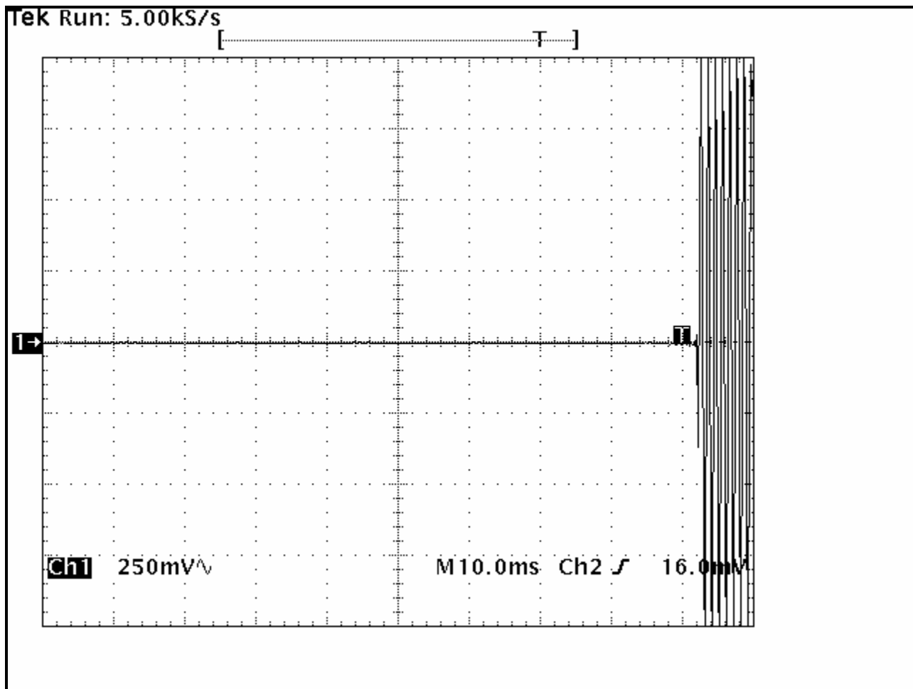
PLOT 13-4: TRANSIENT FREQUENCY BEHAVIOR – 460.525 MHZ; HIGH POWER; NARROW BAND; CARRIER OFF TIME
