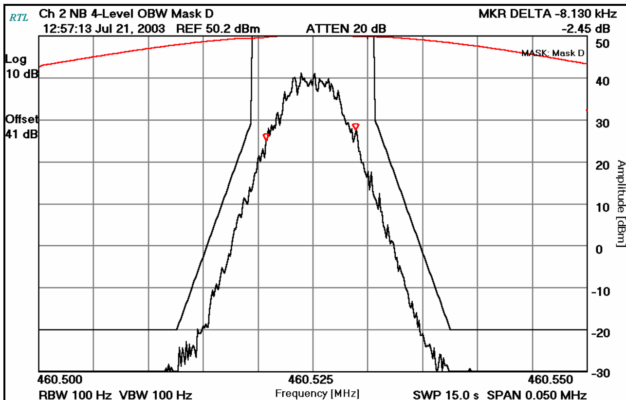
PLOT 8-6: 99% OCCUPIED BANDWIDTH - C4FM; NARROW BAND; 4800 BAUD
