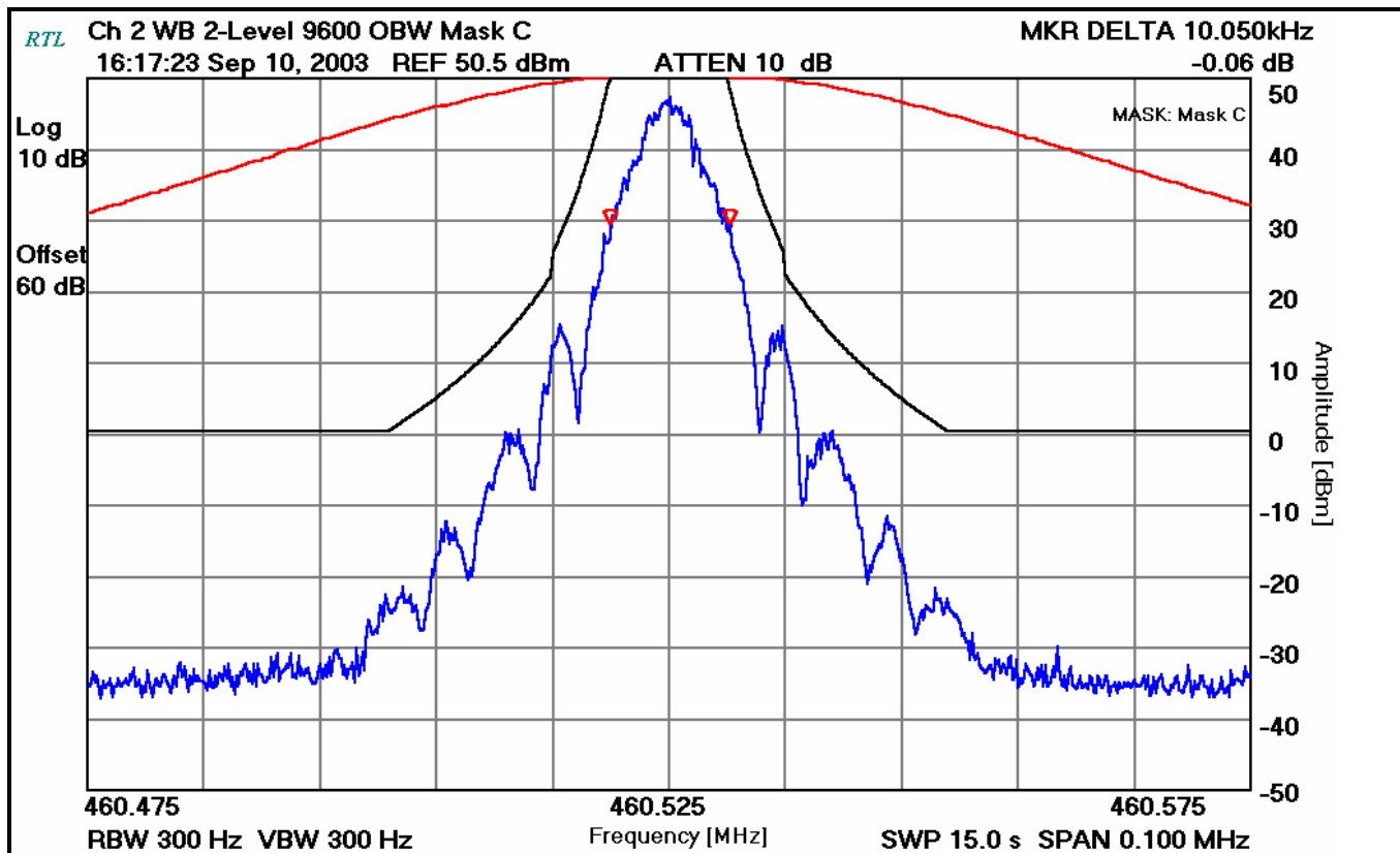
PLOT 8-3: 99% OCCUPIED BANDWIDTH - 2 LEVEL DIGITAL; WIDE BAND; 9600 BAUD
