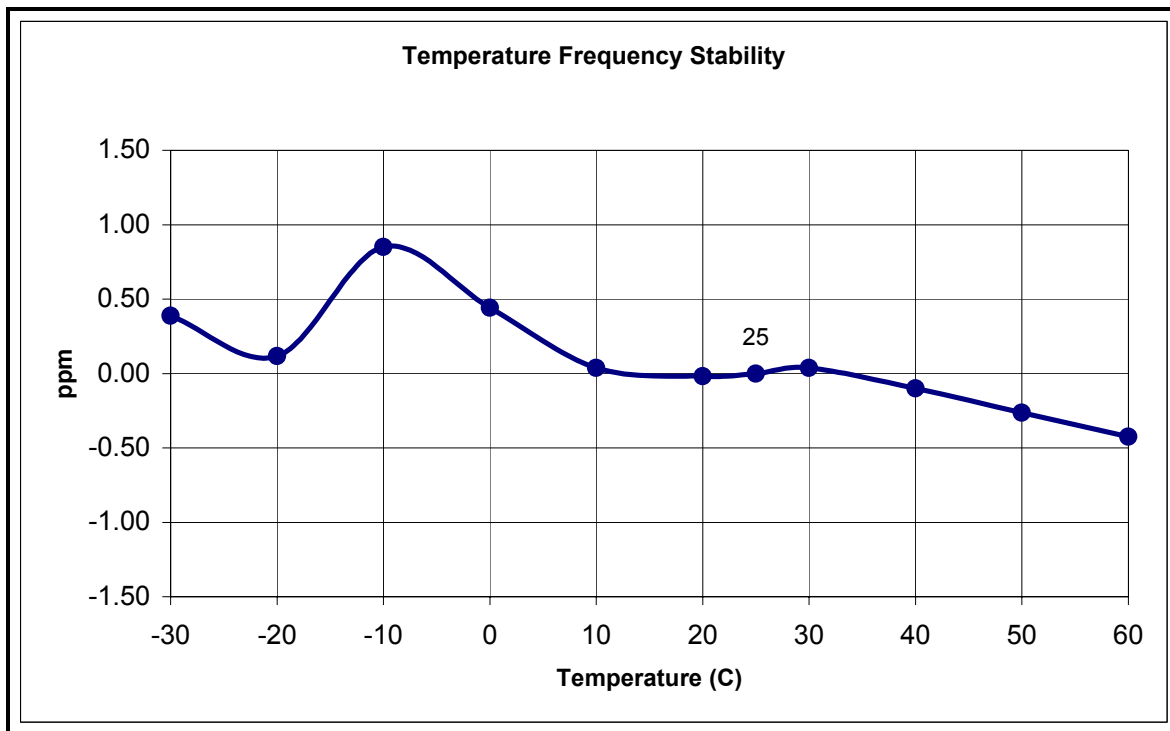
PLOT 9-1: TEMPERATURE FREQUENCY STABILITY
