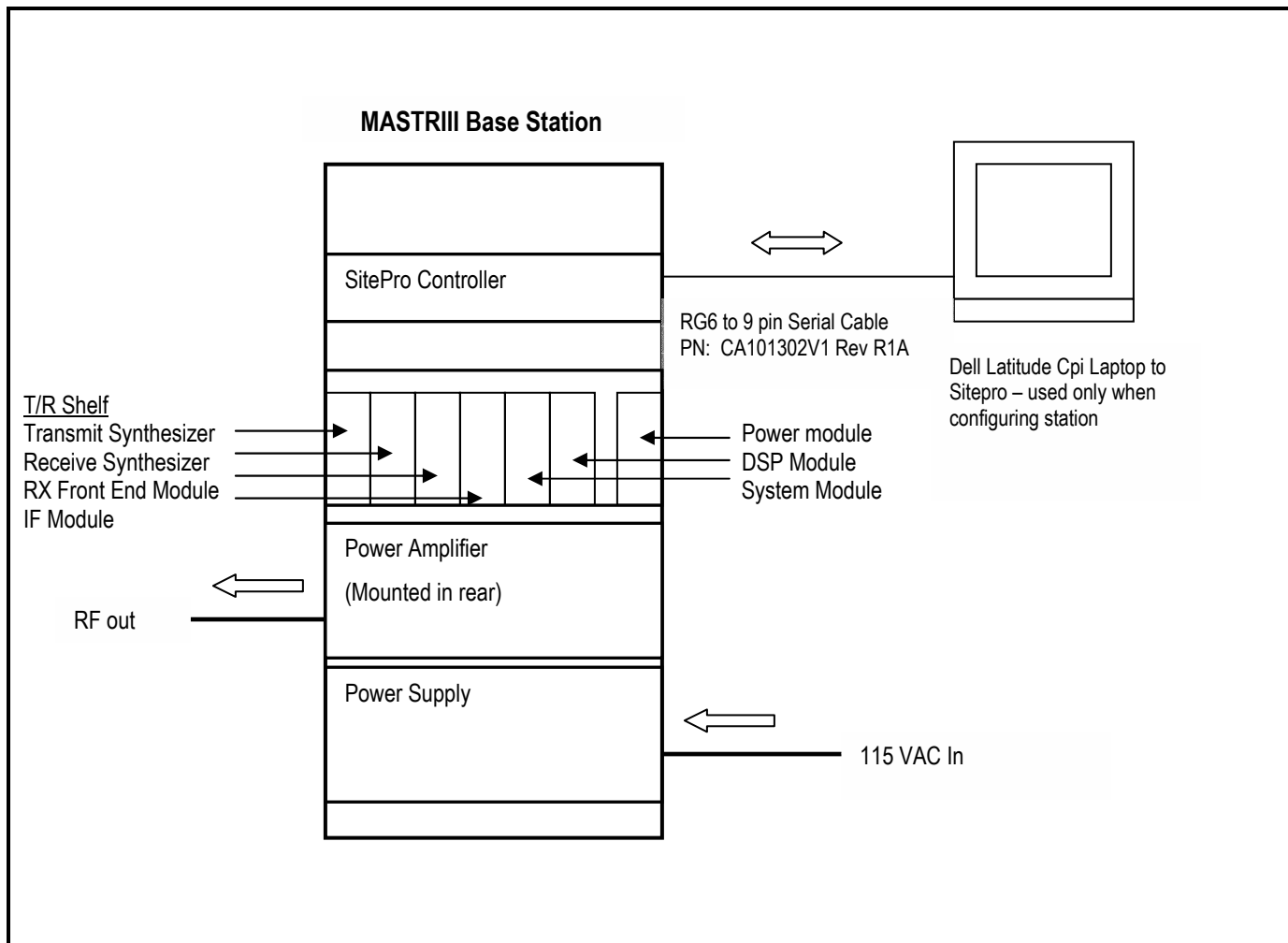
FIGURE 3-1: CONFIGURATION OF TESTED SYSTEM
