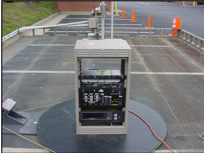
PHOTOGRAPH 1: RADIATED EMISSIONS FRONT VIEW
