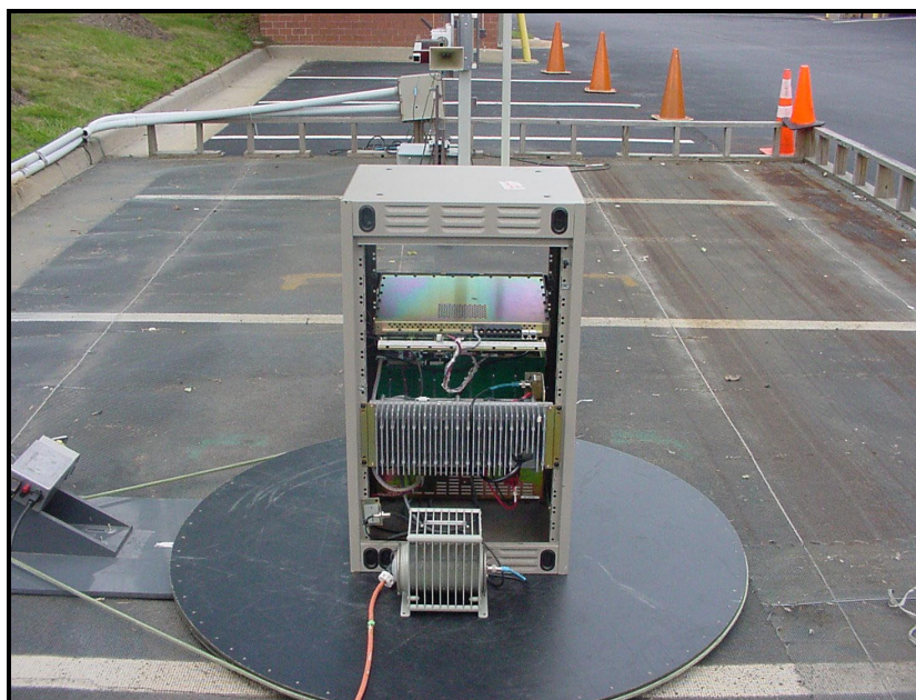
PHOTOGRAPH 2: RADIATED EMISSIONS REAR VIEW
