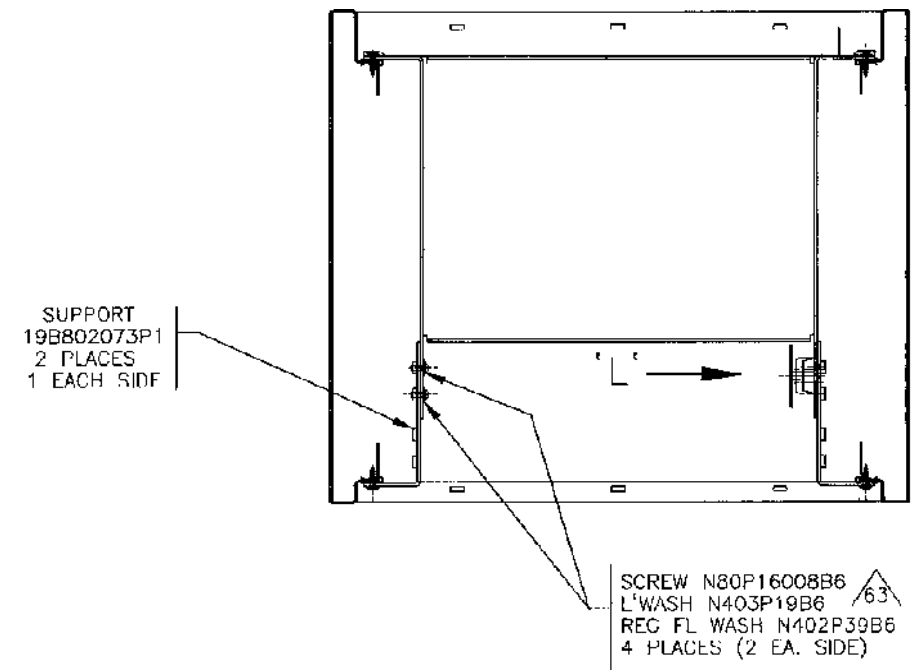
SECTION K-K
