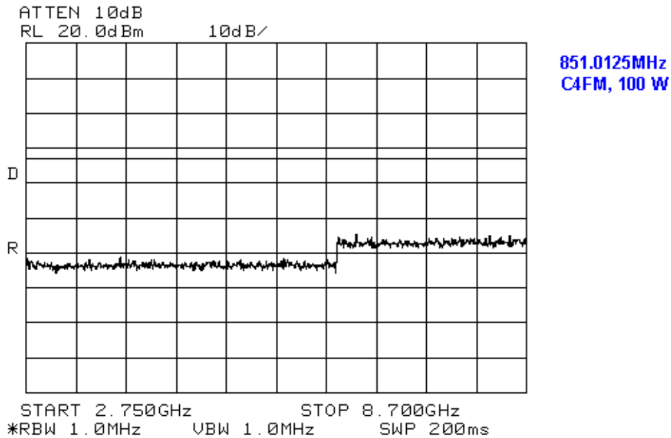
Figure 7-4: Tx at 851.0125 MHz, 100 W power, 2.75 GHz to 8.7 GHz
