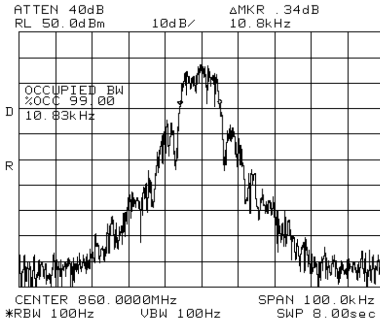
Figure 7-30: 2 level 9600 baud signal with 3 kHz deviation
