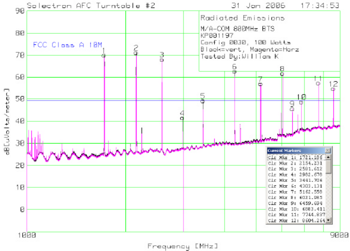
Figure 7-20: Field Strength With 100 W Tx, 1 GHz to 9 GHz
