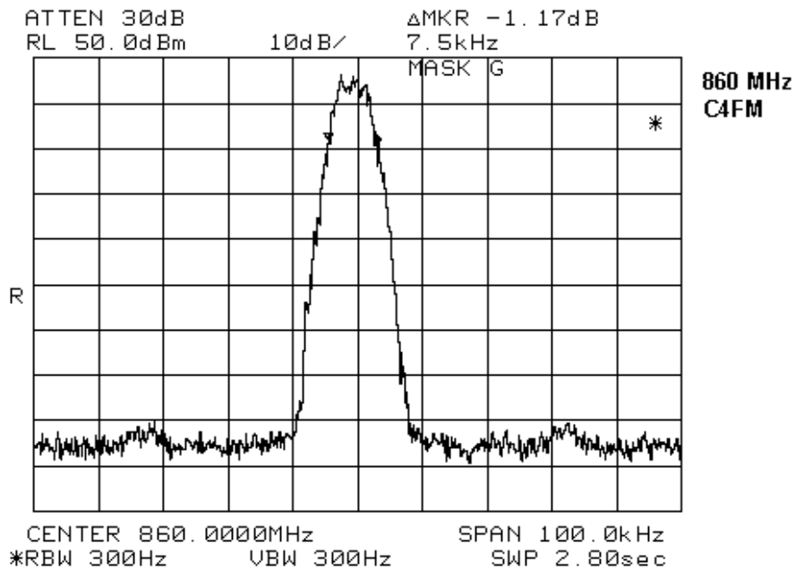
Figure 7-24: NPSPAC (9600 baud) Signal
