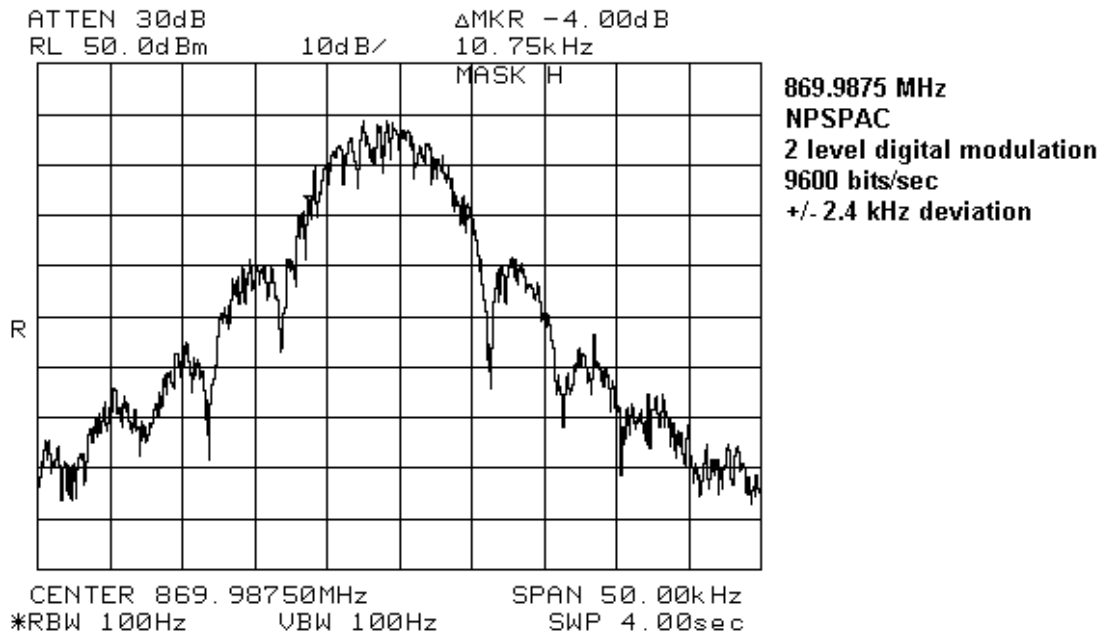
Figure 7-24: NPSPAC (9600 baud) Signal
