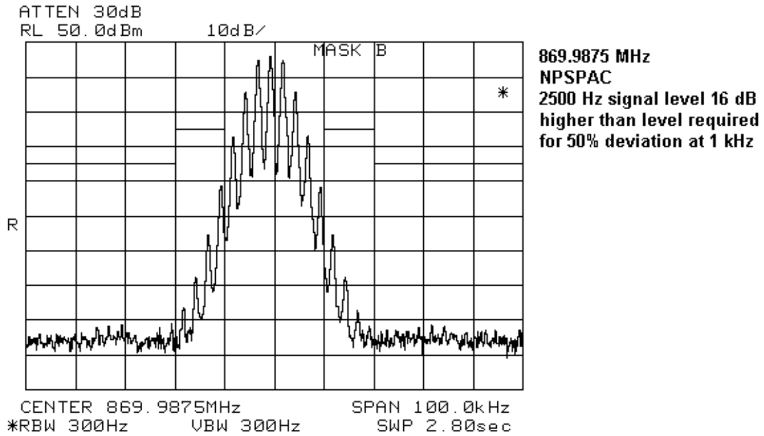
Figure 7-18: NPSPAC (Analog) signal
