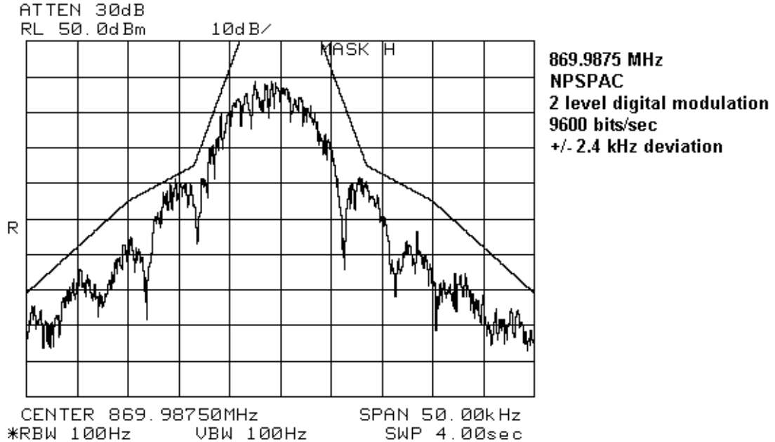
Figure 7-17: NPSPAC (9600 baud) Signal
