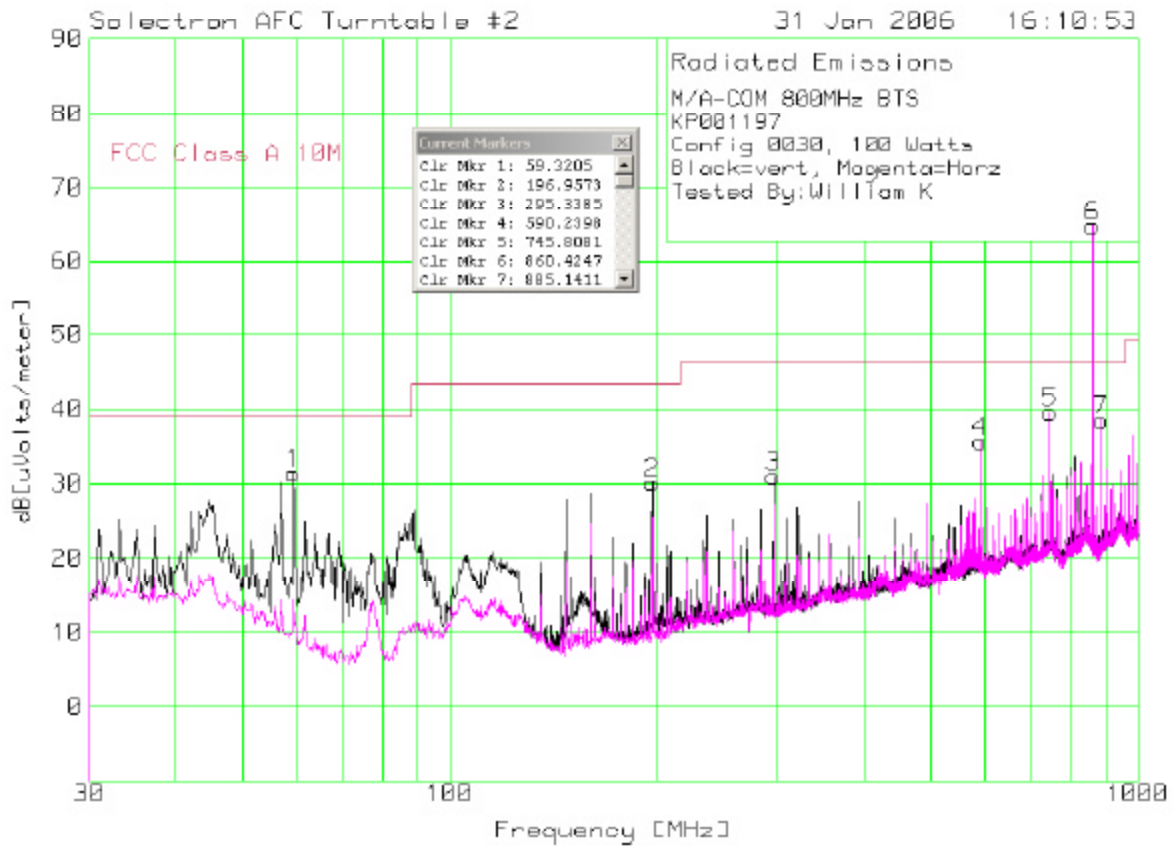
Figure 7-19: Field Strength With 100 W Tx, 30 MHz to 1 GHz
