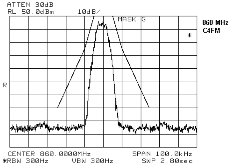
Figure 7-17: NPSPAC (9600 baud) Signal
