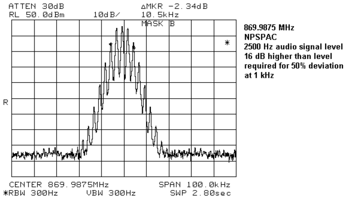
Figure 7-25: NPSPAC (Analog) Signal
