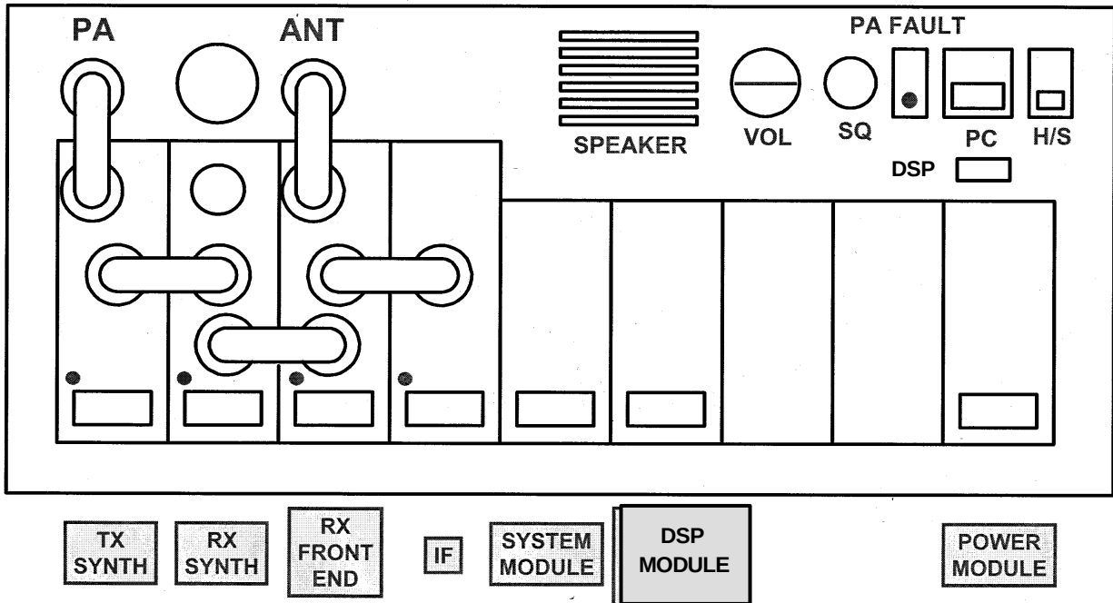
Figure 3-2: Module Configuration
