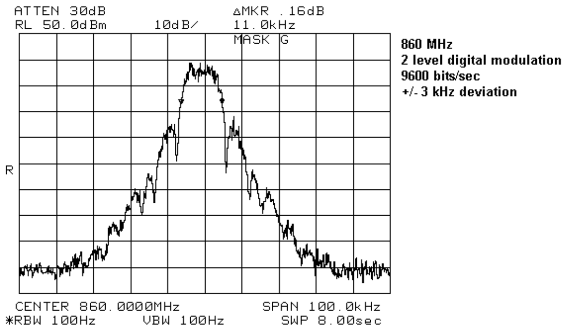
Figure 7-22: 2 Level 9600 baud Signal With 3 kHz Deviation
