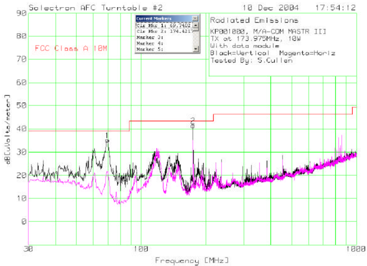
Figure 7-17: Field Strength with 10 W Tx, 30 MHz to 1 GHz, 173.975 MHz
