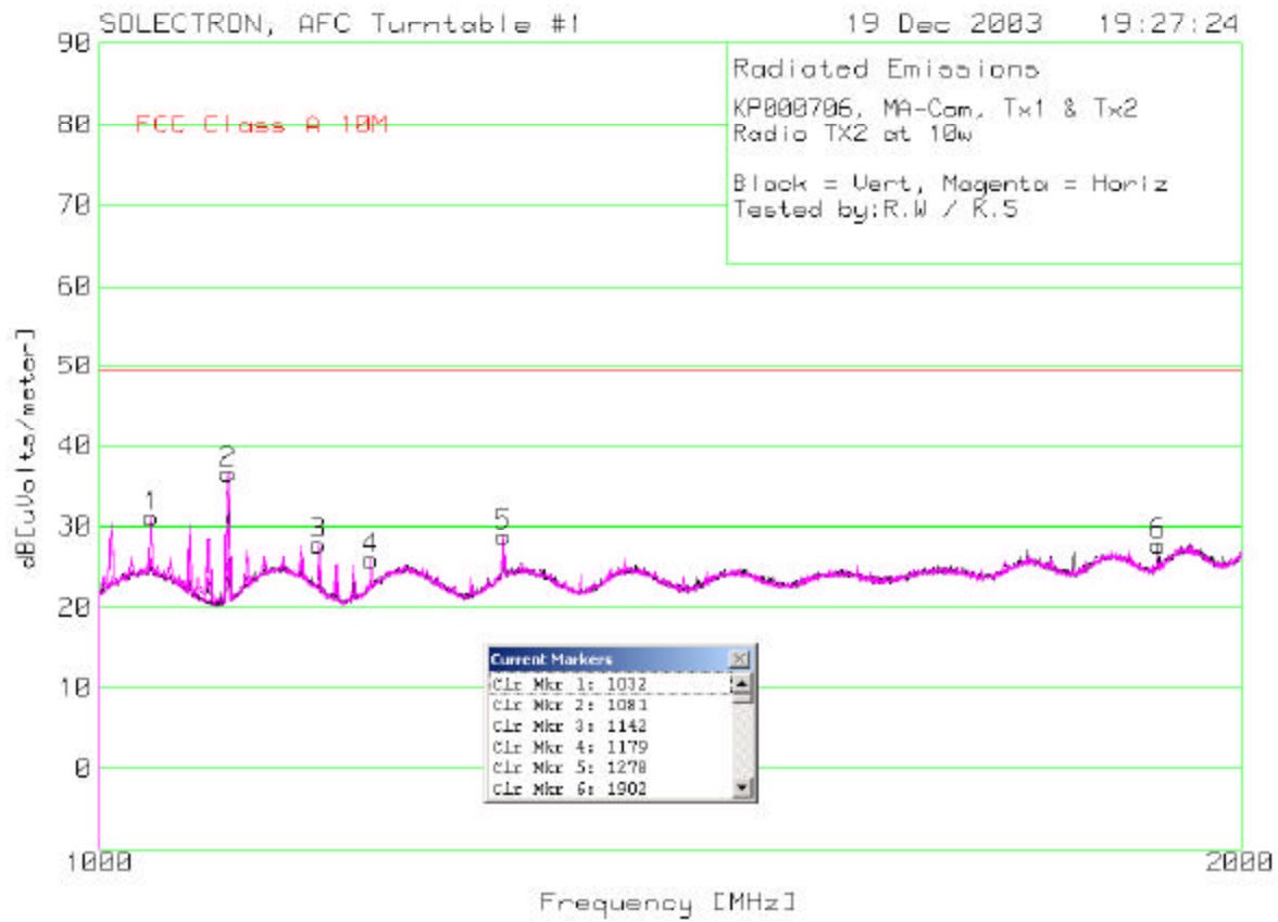
Figure 7-26: Field strength with 10 W Tx, 1 GHz to 2 GHz, high frequency split
