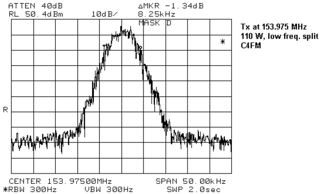
Figure 7-35: C4FM signal
