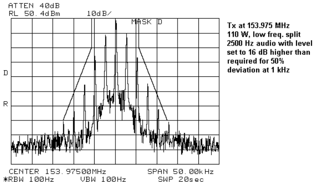
Figure 7-15: 2500 Hz audio signal Narrowband
