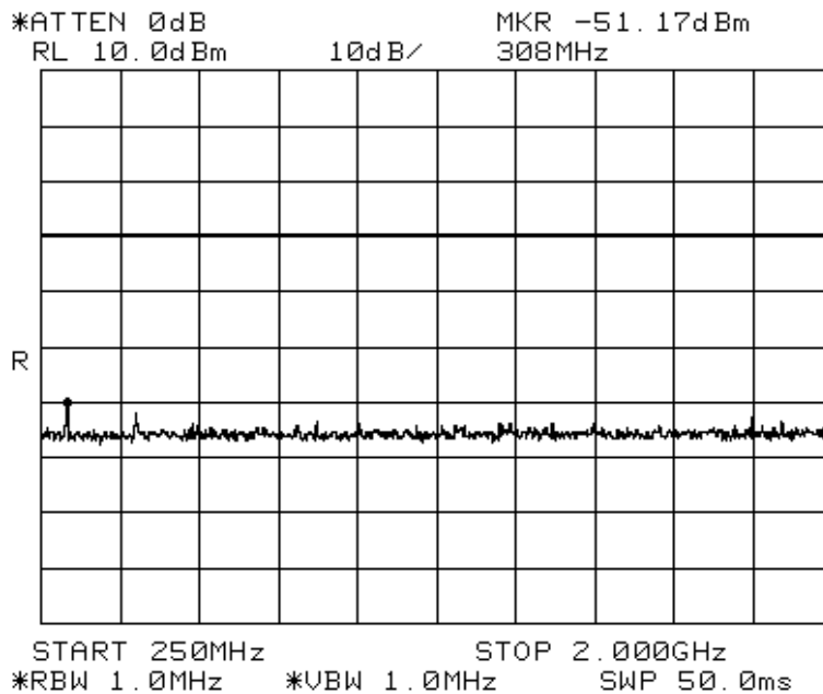
Figure 7-5: Tx at 153.975 MHz (low split), 10 W Power, 250 MHz to 2 GHz
