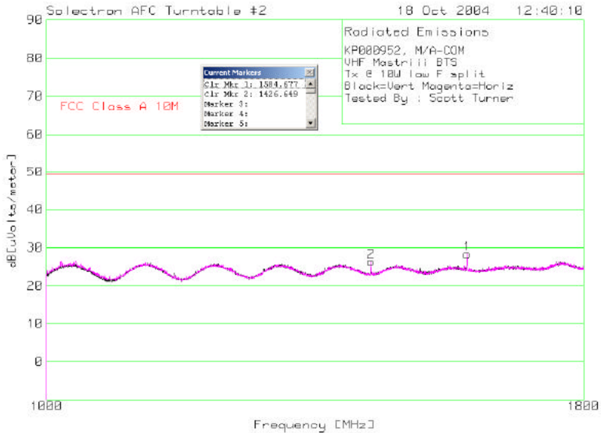
Figure 7-19: Field Strength with 10 W Tx, 1 GHz to 1.8 GHz, Low Frequency Split
