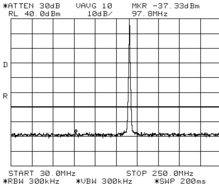
Figure 7-4: Tx at 153.975 MHz (low split) , 10 W Power, 30 MHz to 250 MHz
