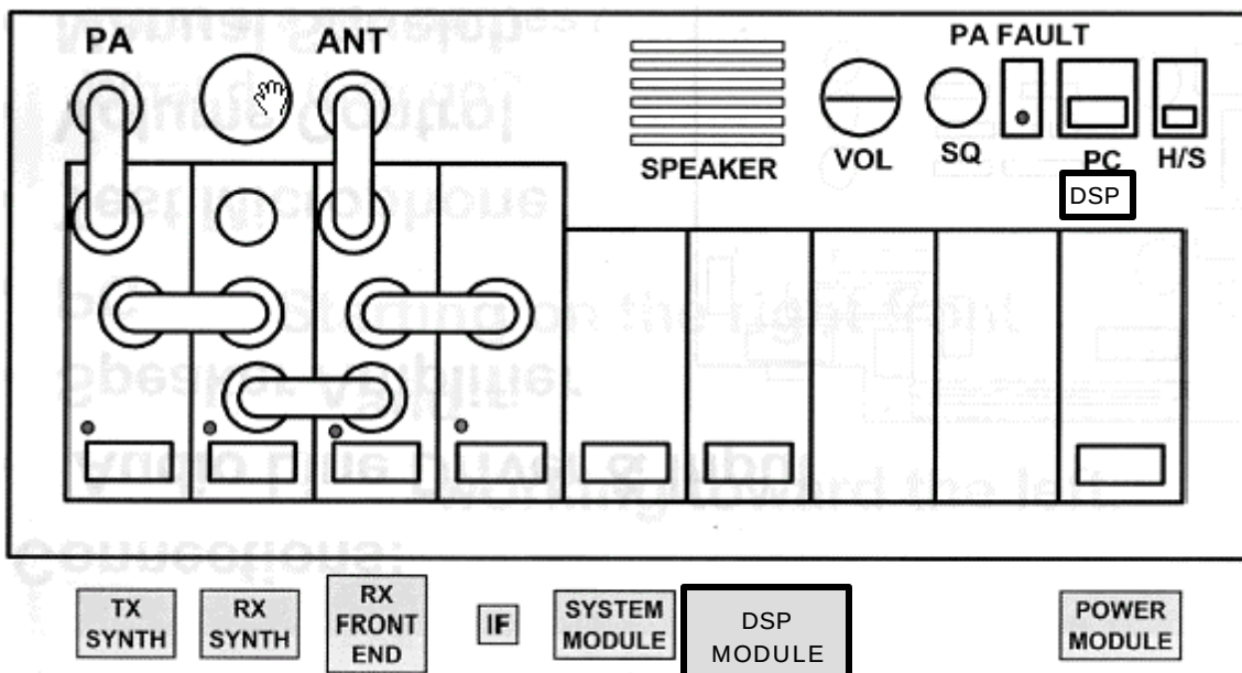
Figure 3-2: Module Configuration
