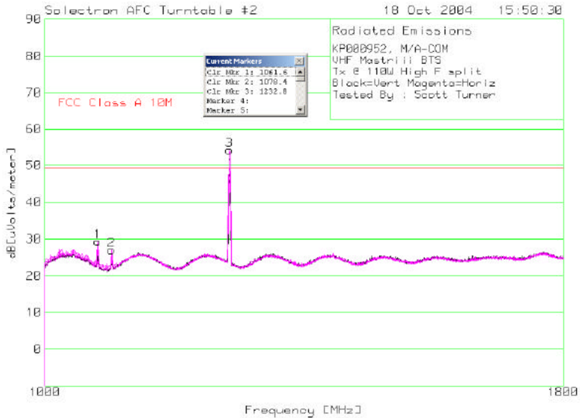
Figure 7-17: Field Strength with 110 W Tx, 1 GHz to 1.8 GHz, High Frequency Split
