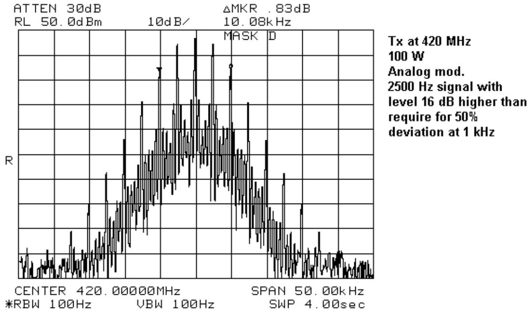
Figure 7-39: 2500 Hz audio signal Wideband, 420 MHz
