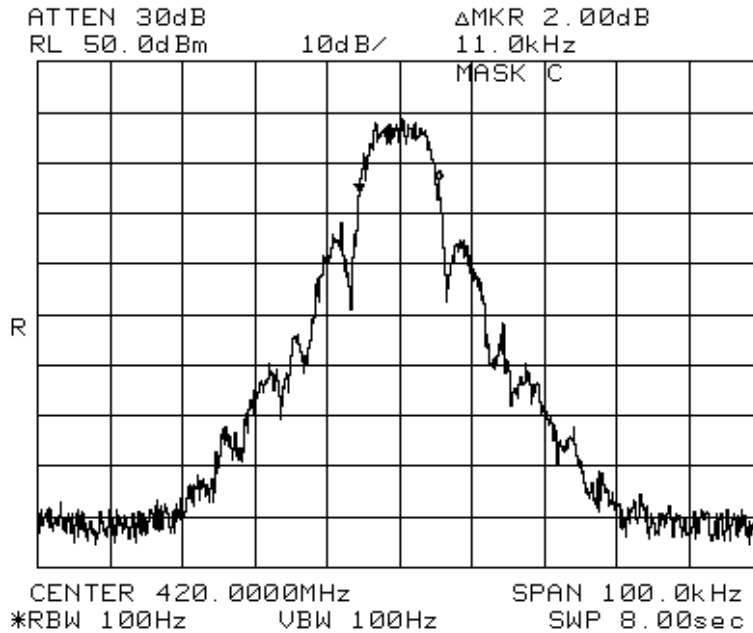
Figure 7-41: 2 level 9600 baud signal with +/- 3 kHz deviation, 420 MHz
