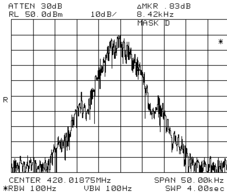
Figure 7-42: 2 level 9600 baud signal with +/- 1.9 kHz deviation, 420 MHz
