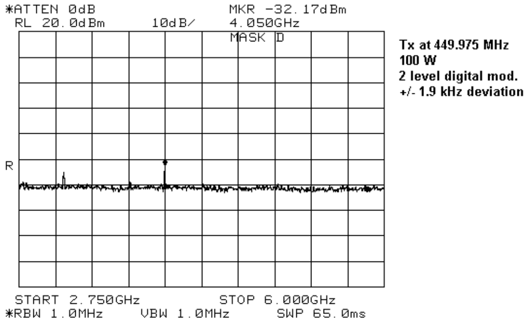
Figure 7-16: Tx at 449.975 MHz , 100 W power, 2.75 GHz to 6 GHz
