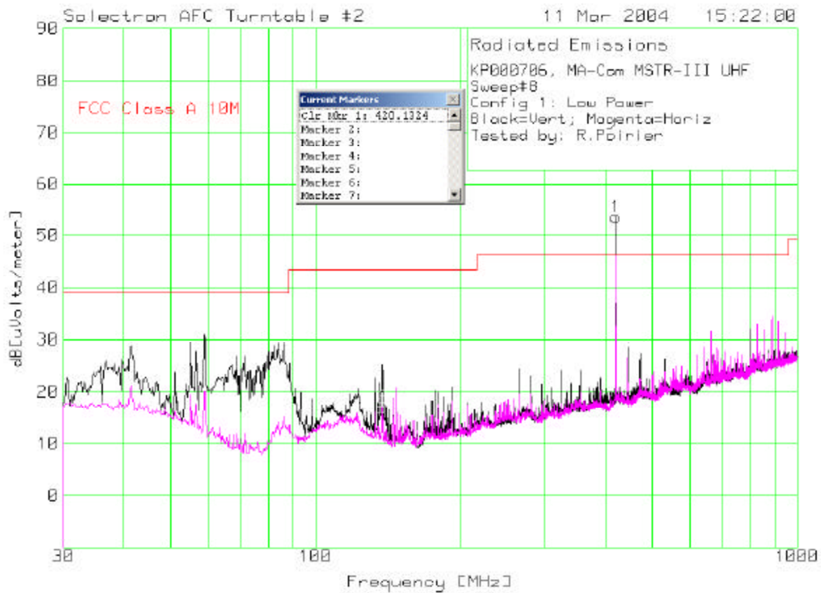
Figure 7-29: Field strength with 10 W Tx, 30 MHz to 1 GHz (Tx at 420 MHz)
