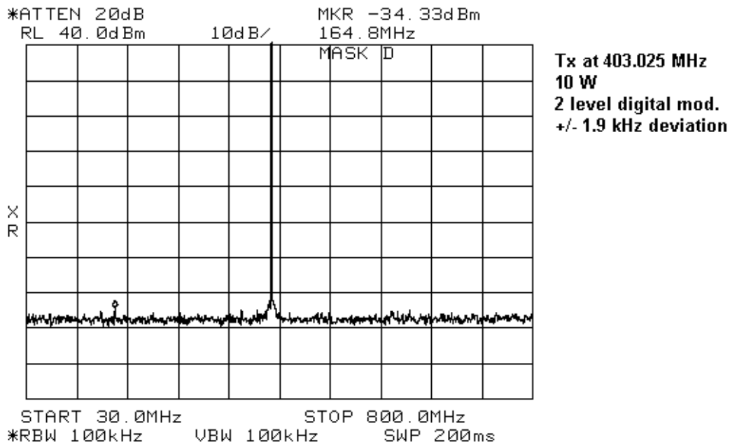
Figure 7-7: Tx at 403.025 MHz , 10 W power, 30 MHz to 800 MHz
