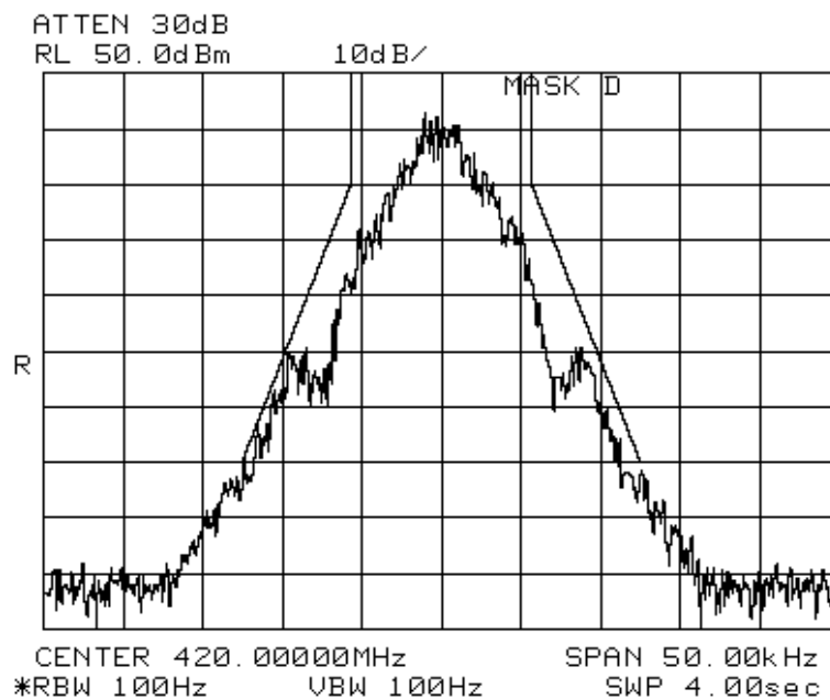
Figure 7-25: 2 level 9600 baud signal with +/- 1.9 kHz deviation, 420 MHz
