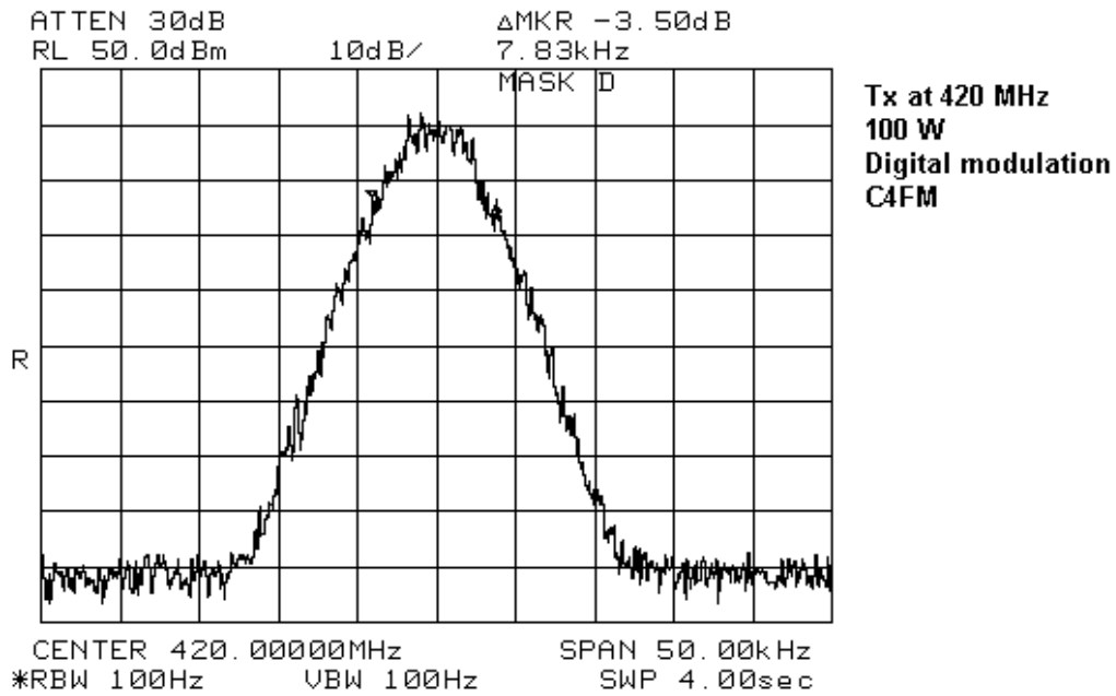
Figure 7-43: C4FM signal, 420 MHz
