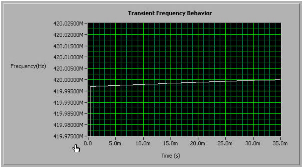
Figure 7-37 Transient Frequency Behavior, Tx at 420 MHz, Narrowband, Transmitter on
