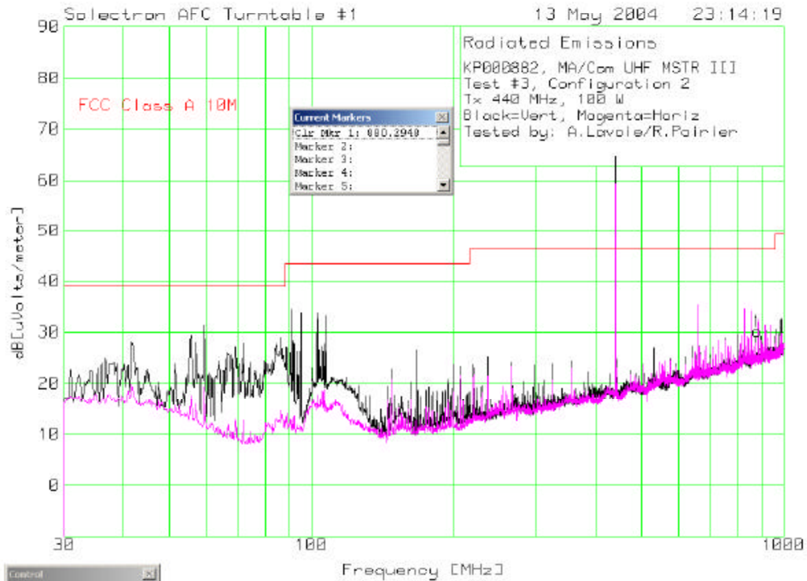
Figure 7-31: Field strength with 100 W Tx, 30 MHz to 1 GHz (Tx at 440 MHz)
