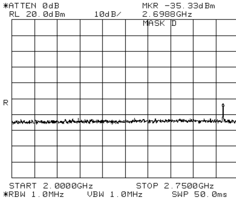
Figure 7-15: Tx at 449.975 MHz , 100 W power, 2 GHz to 2.75 GHz
