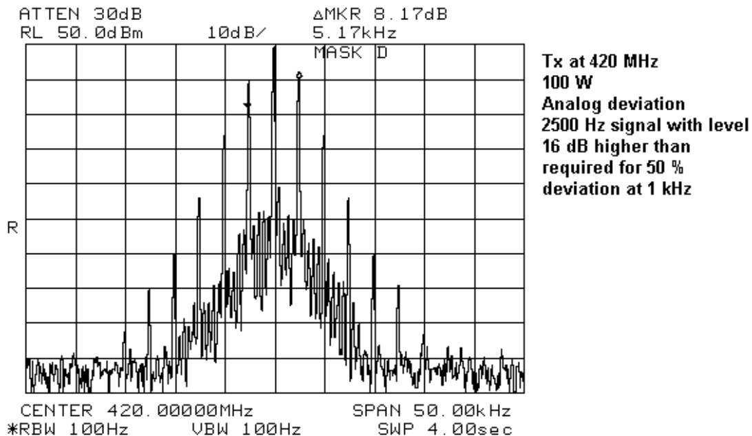
Figure 7-40: 2500 Hz audio signal Narrowband, 420 MHz
