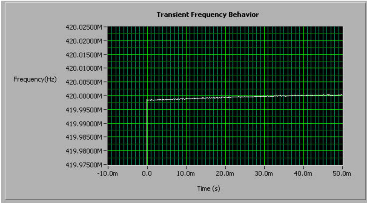
Figure 7-35 Transient Frequency Behavior, Tx at 420 MHz, Wideband, Transmitter on
