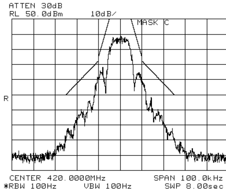
Figure 7-24: 2 level 9600 baud signal with +/- 3 kHz deviation, 420 MHz
