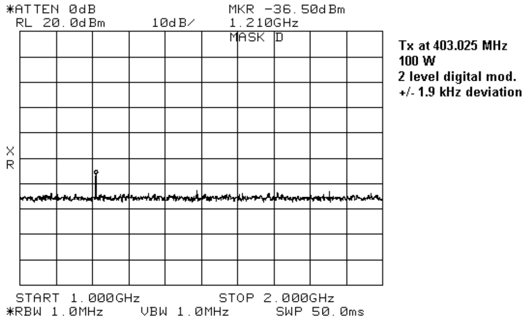
Figure 7-4: Tx at 403.025 MHz , 100 W power, 1 GHz to 2 GHz
