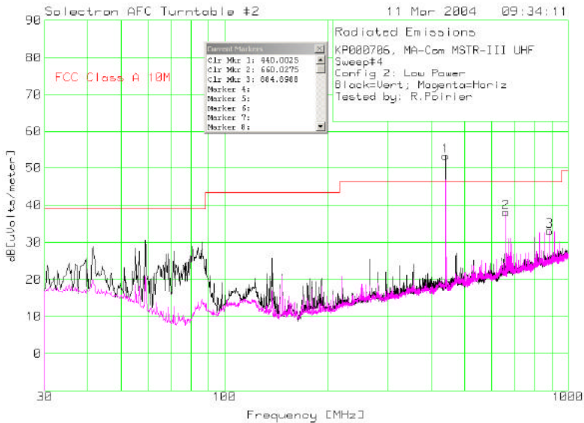
Figure 7-33: Field strength with 10 W Tx, 30 MHz to 1 GHz (Tx at 440 MHz)
