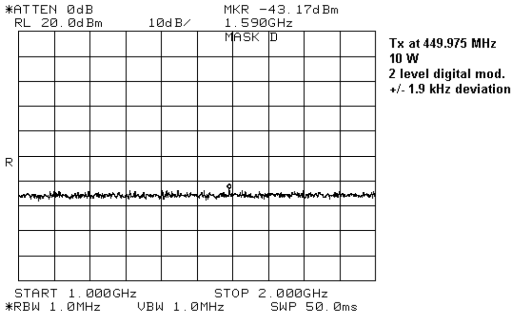
Figure 7-19: Tx at 449.975 MHz , 10 W power, 1 GHz to 2 GHz
