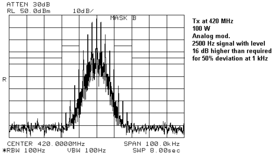
Figure 7-22: 2500 Hz audio signal Wideband, 420 MHz
