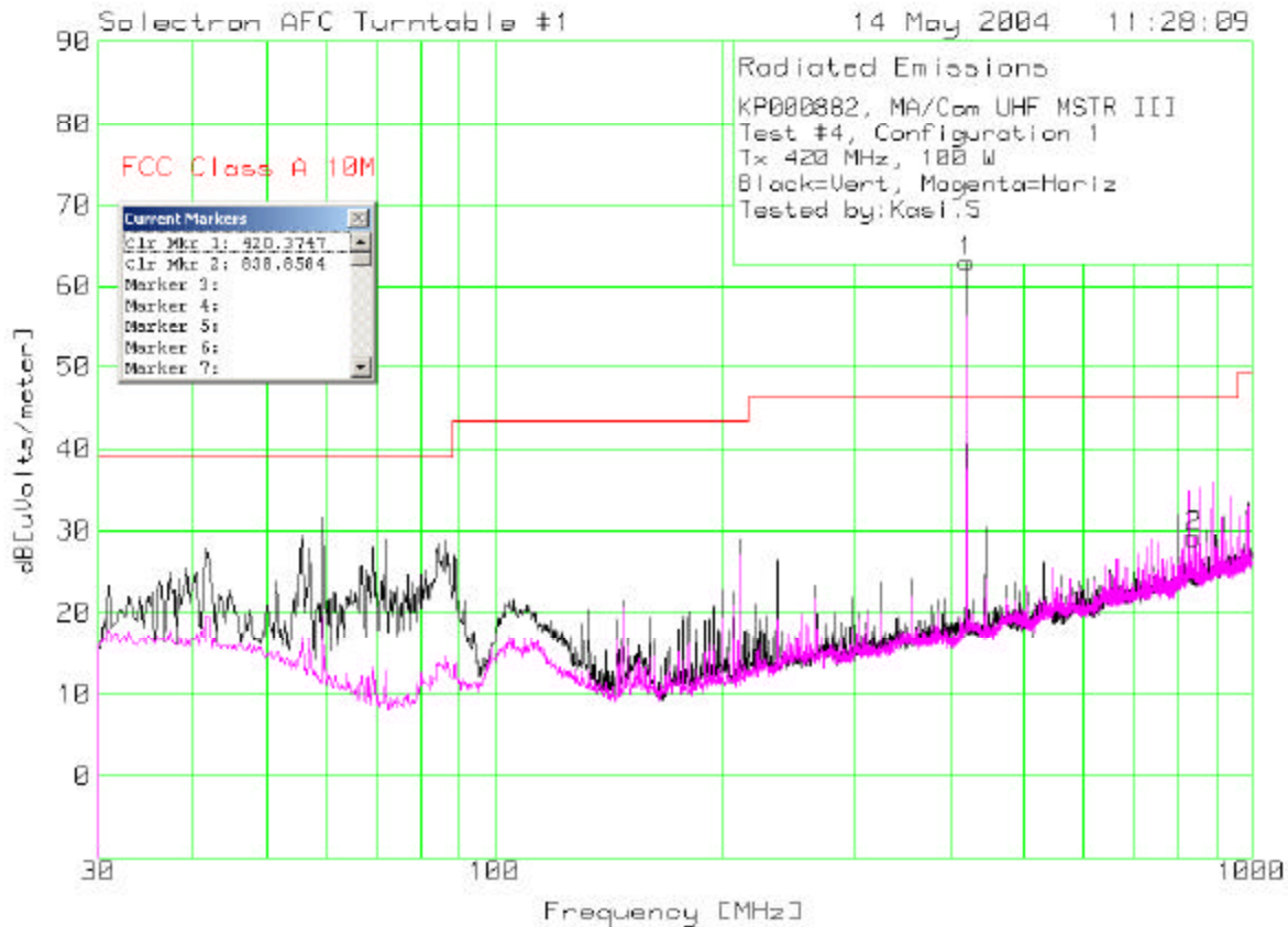
Figure 7-27: Field strength with 100 W Tx, 30 MHz to 1 GHz (Tx at 420 MHz)
