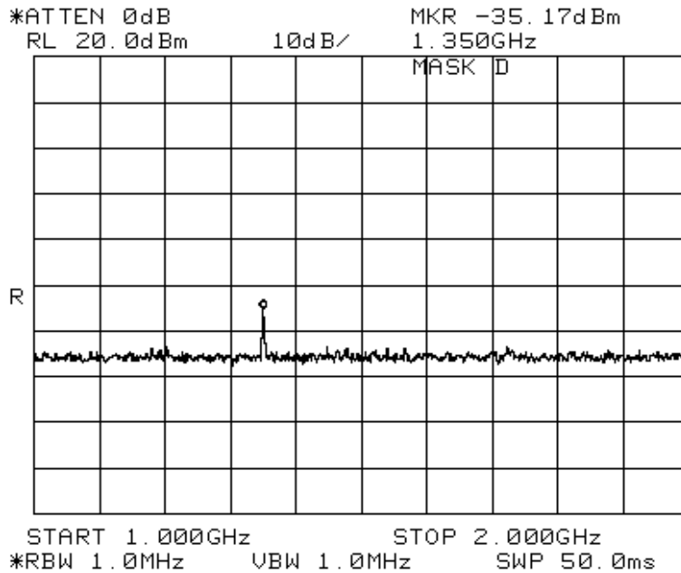
Figure 7-14: Tx at 449.975 MHz , 100 W power, 1 GHz to 2 GHz
