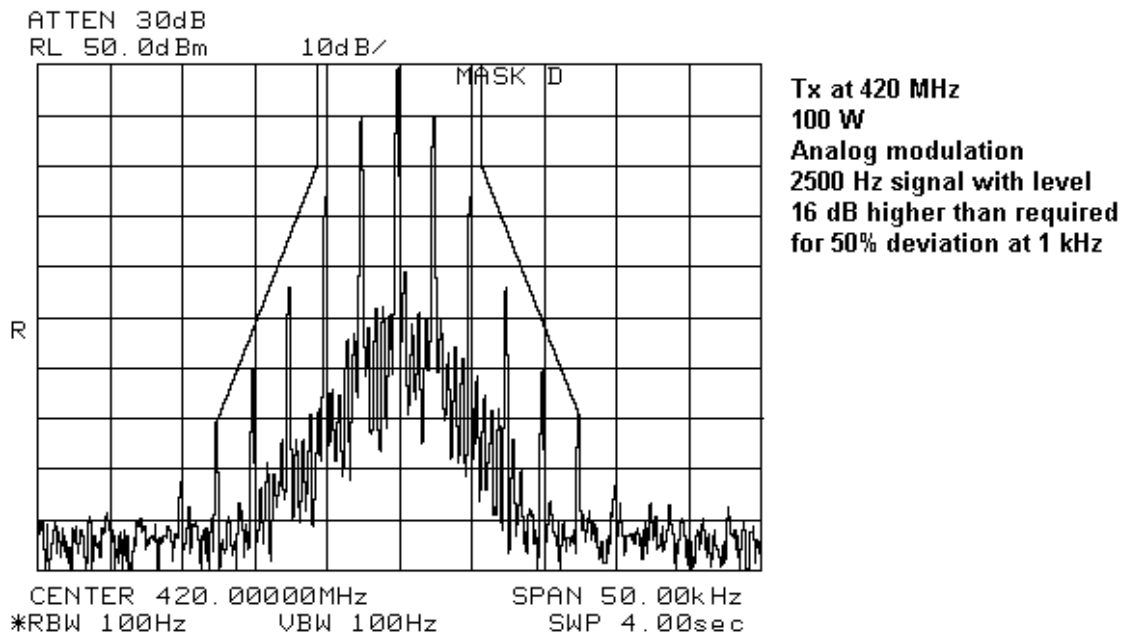
Figure 7-23: 2500 Hz audio signal Narrowband, 420 MHz
