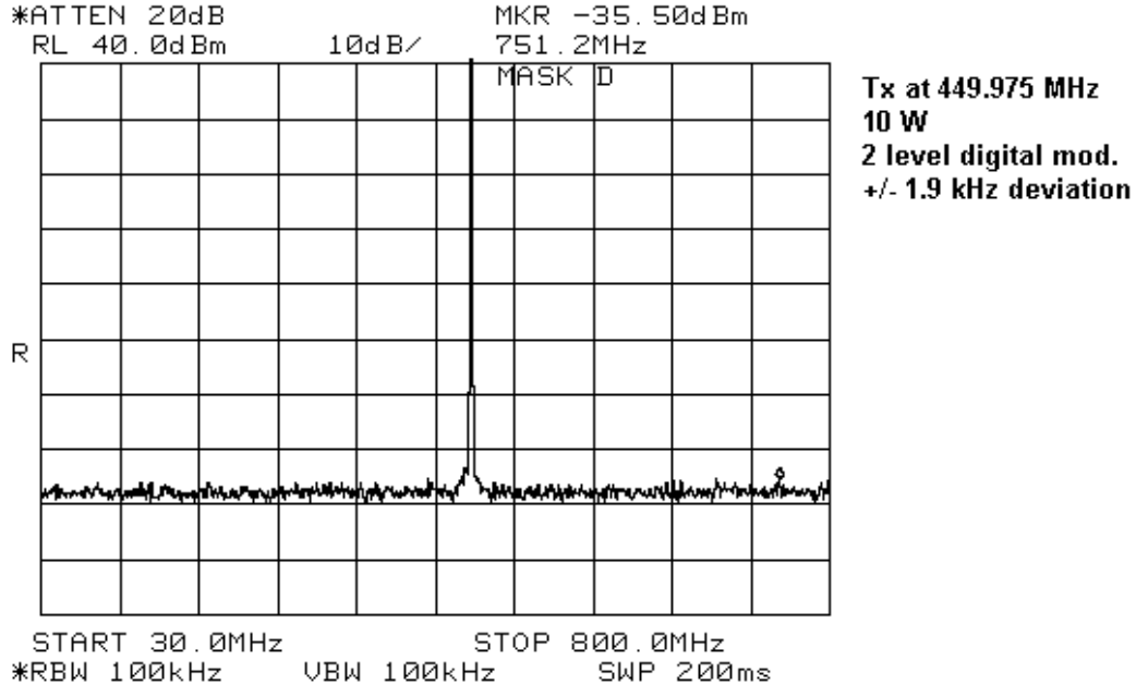
Figure 7-17: Tx at 449.975 MHz , 10 W power, 30 MHz to 800 MHz
