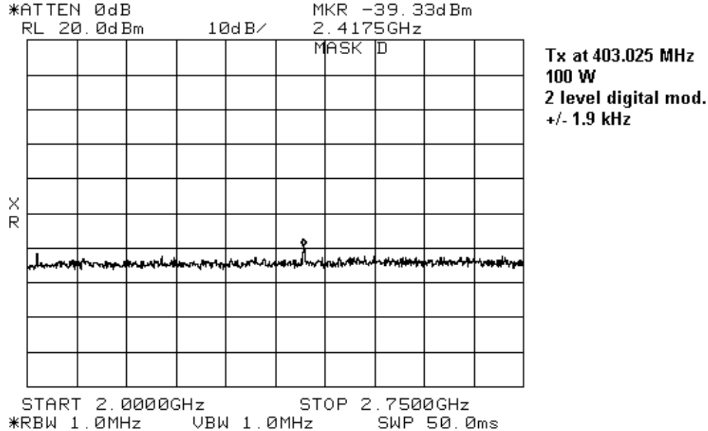
Figure 7-5: Tx at 403.025 MHz , 100 W power, 2 GHz to 2.75 GHz
