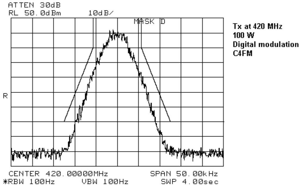
Figure 7-26: C4FM signal, 420 MHz
