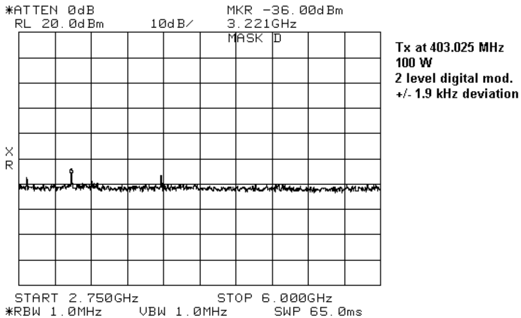
Figure 7-6: Tx at 403.025 MHz , 100 W power, 2.75 GHz to 6 GHz
