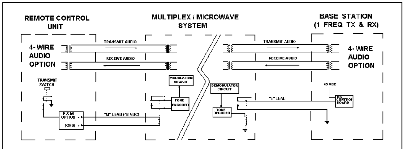
Figure 7 - Typical E &amp; M Signaling Application
