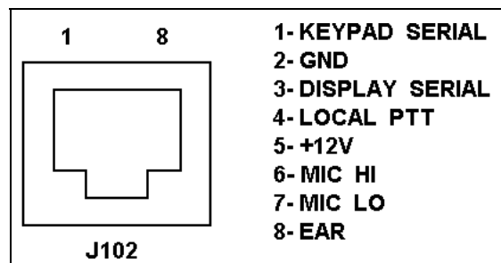
Figure 5 - Microphone Connections
