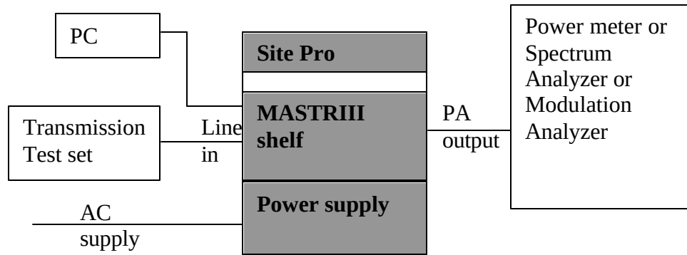
Figure 3-3: System Configuration
