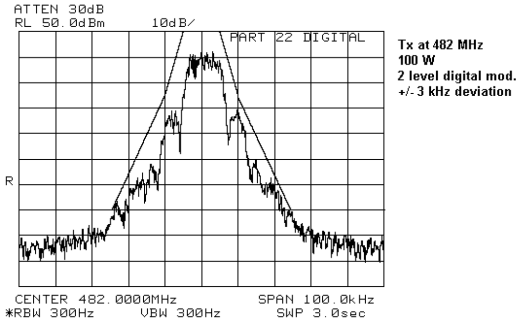
Figure 7-29: 2 level 9600 baud signal with +/- 3 kHz deviation, 482 MHz, FCC Part 22 mask
