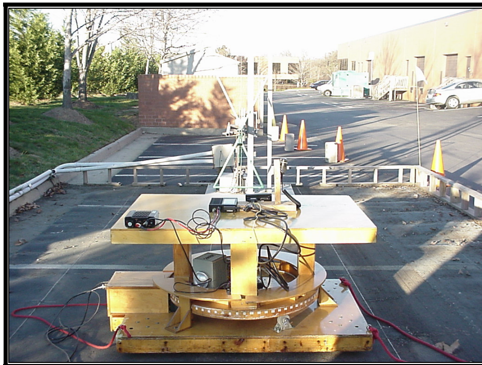
PHOTOGRAPH 9: RADIATED EMISSIONS REAR VIEW
