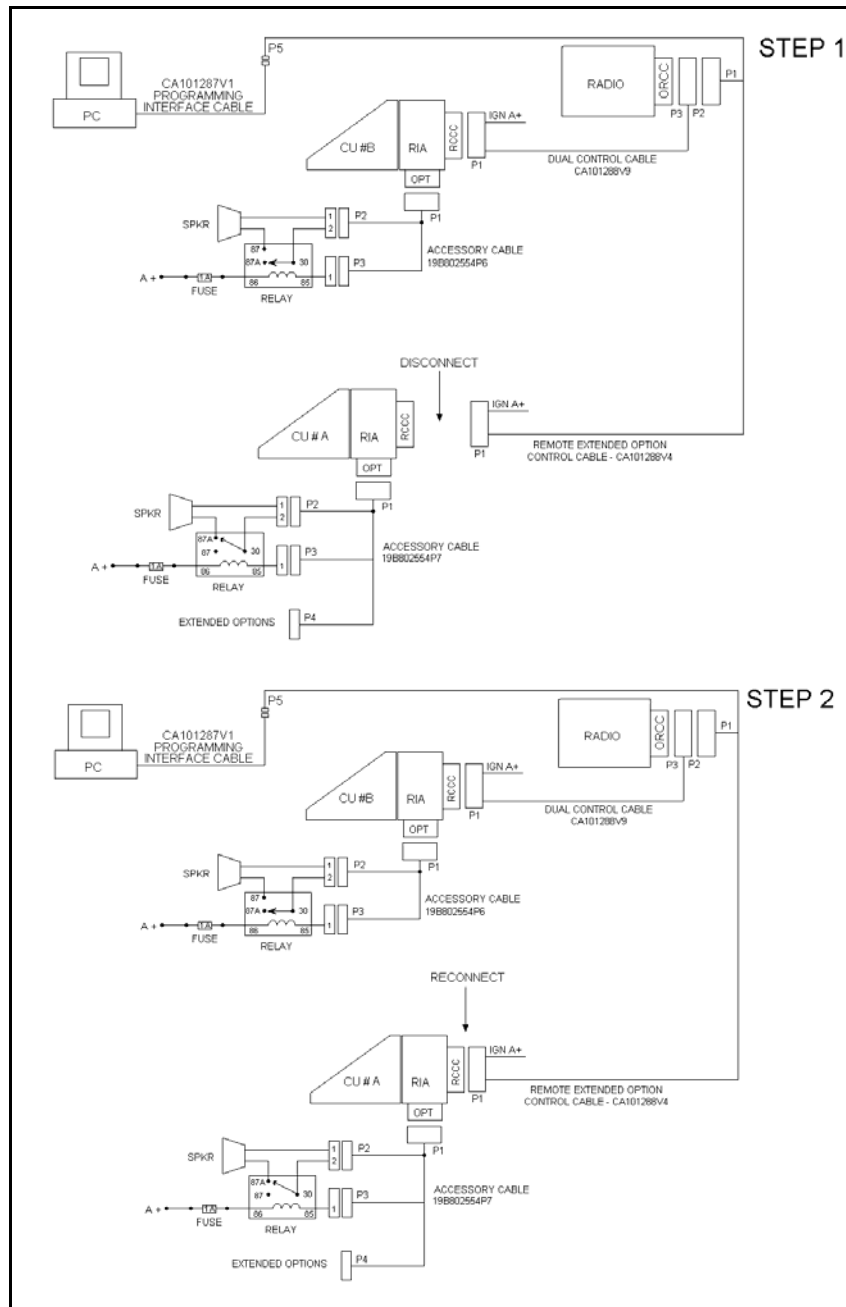
Figure 10-9: M7100 IP Field Programming – Dual Control Unit Remote/Remote Mount Configuration
