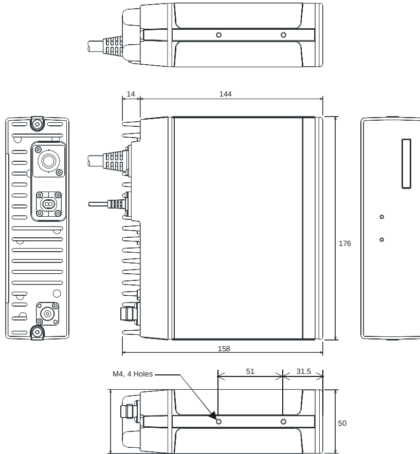
D3100 MECHANICAL VIEWS
